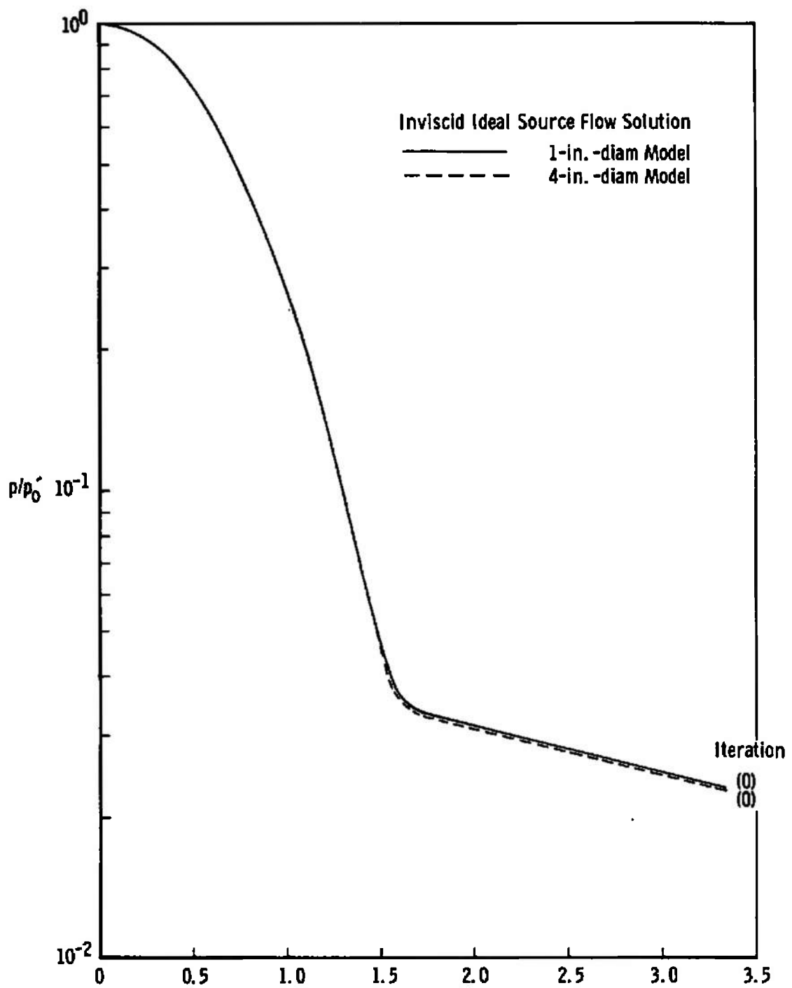
Fig. 6 Scale Effects on Surface Pressure Distribution in Ideal Source Flow in Tunnel F
