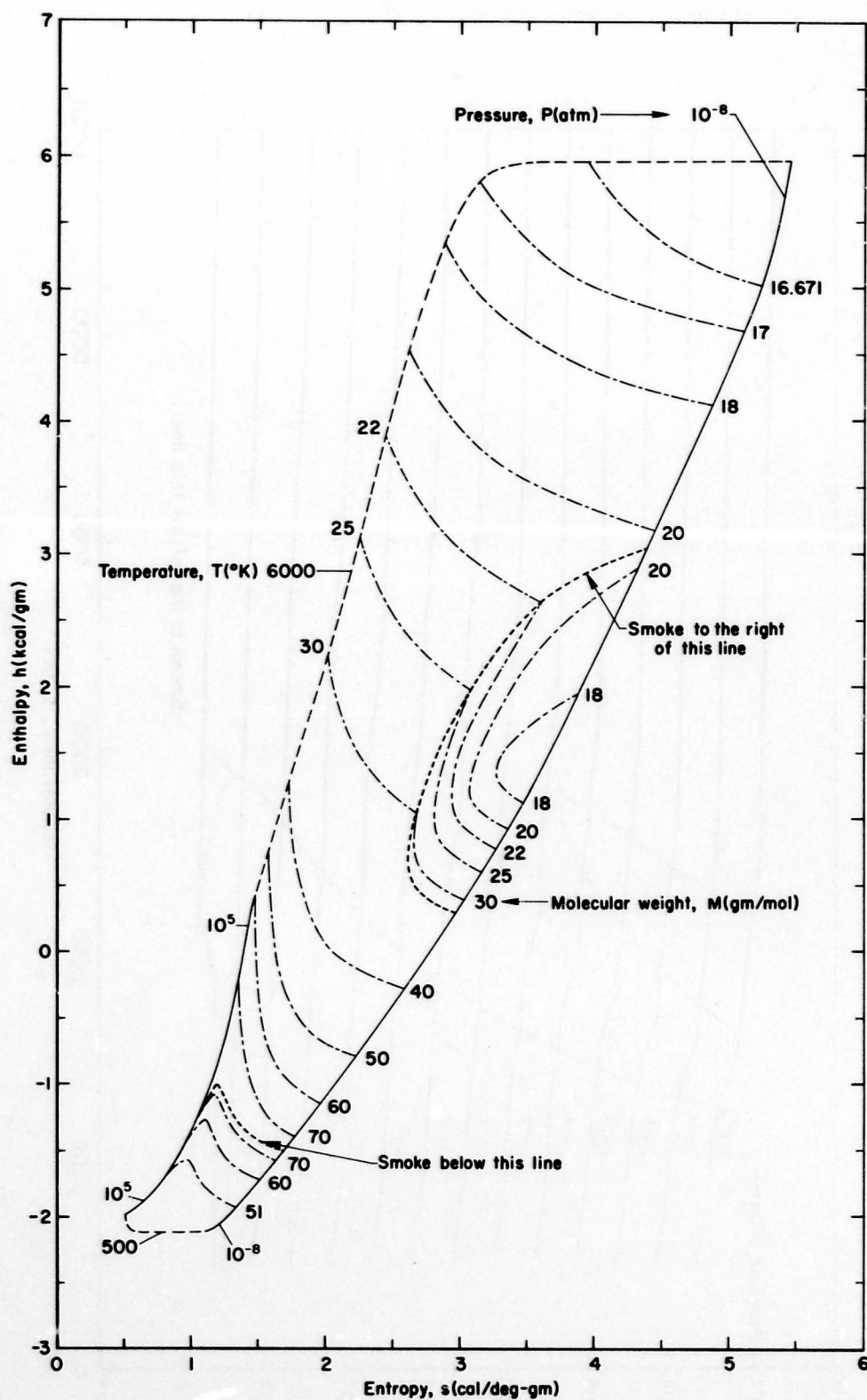
Fig.2—Enthalpy versus entropy for Teflon with cross plots of constant molecular weight
