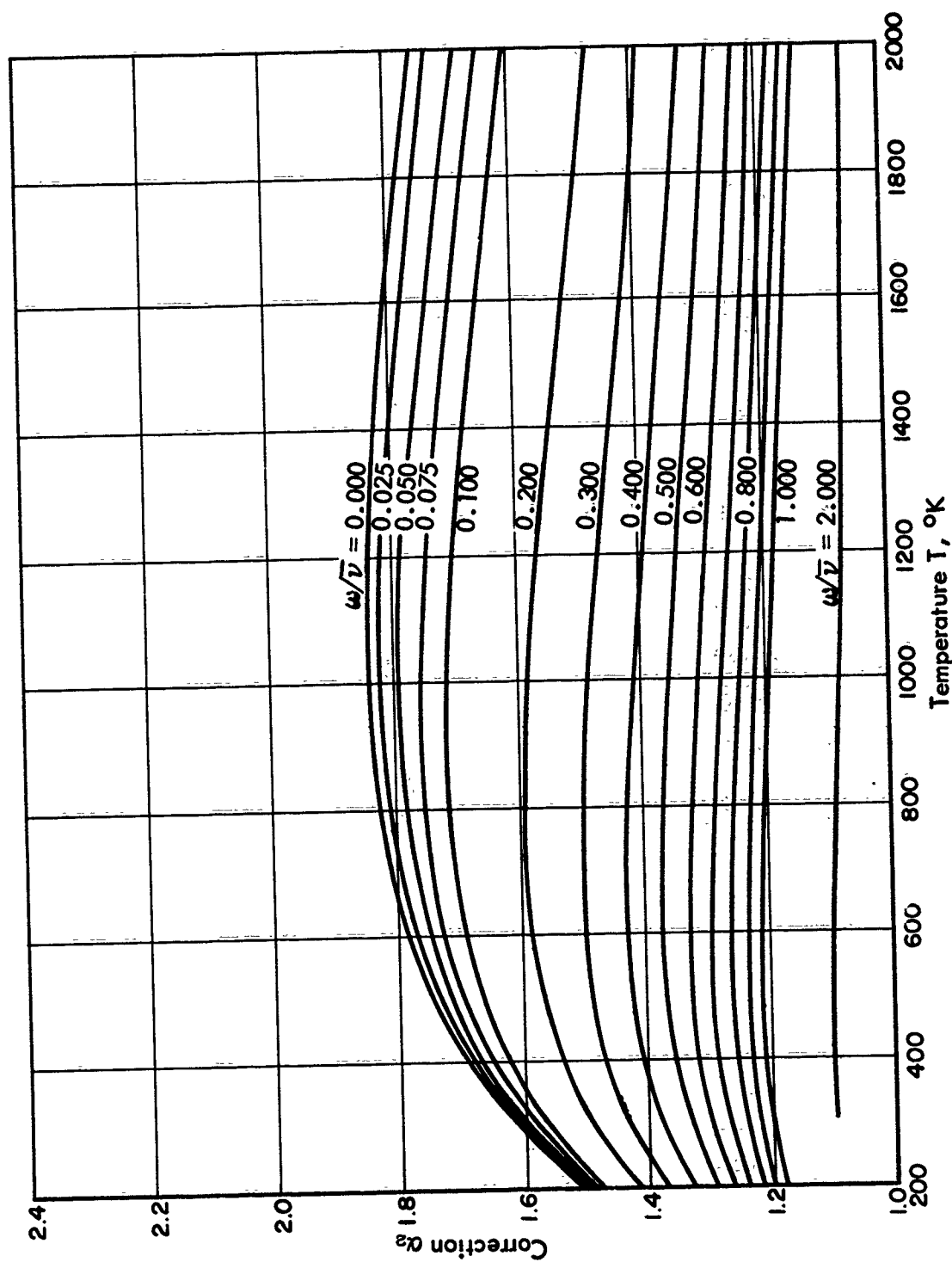
FIGURE 19 Correction \alpha_2 for Weakly Ionized Oxygen, O_2 , at Constant \omega/\bar{v} (MODEL I)
