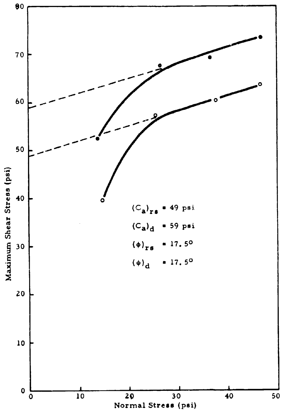
Figure III. 8 Failure Envelopes for Jordan Buff Clay: w \approx 10\%
