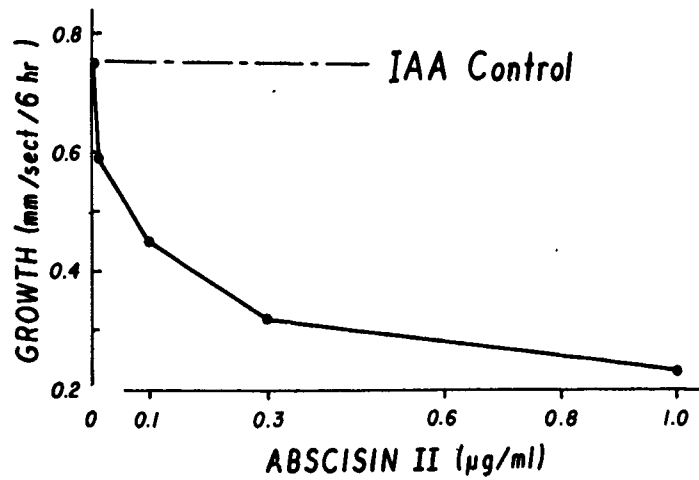
Figure 2. Effect of Inhibitor Eluate and Abscisin II on Growth of Avena Coleoptile Sections.
