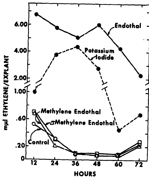
Figure 4. Effect of Deoiliants on Ethylene Production by Bean Petiole Explants.
