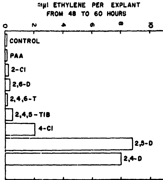
Figure 1. Effect of Various Phenoxycetic Acids on Ethylene Production of Bean Petiole Abscission Zones. Explants were in plain agar for 48 hours before being transferred to test substances.
