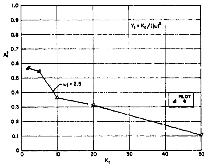
Figure 53. Relative Remnant Versus K_c for Y_c = K_c/(j\omega)^2
