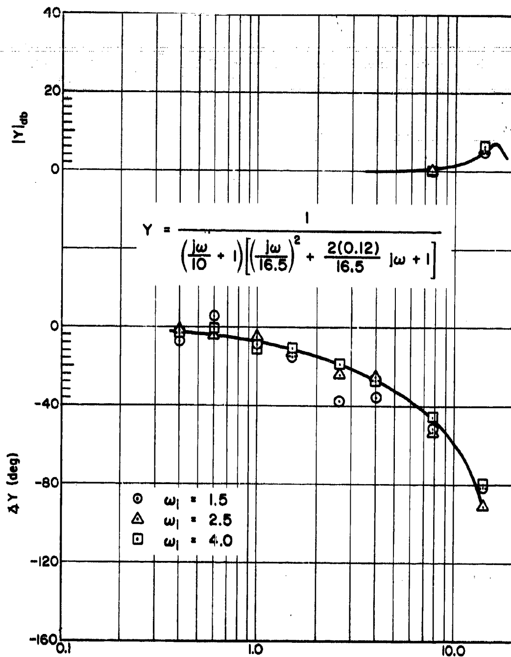
Figure 84. Residual Amplitude Ratio and Phase Giving High Frequency Neuromuscular System Characteristics for Y_c = K_0 / (j\omega - 2)
