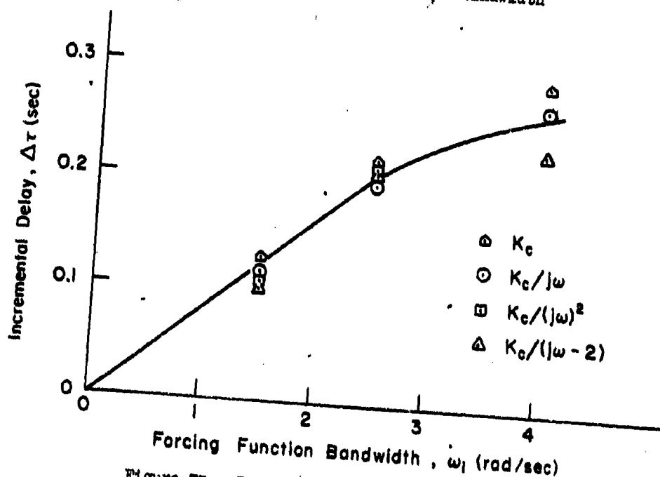
Figure 75. Dependence of Incremental Time Delay on Forcing Function Bandwidth
