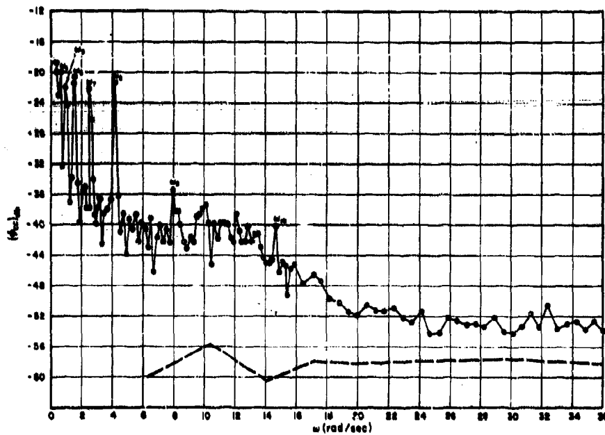
Figure 69. Output Power Spectrum; Y_0 = K_0 = 10 , \omega_1 = 4 , 1" Pilot 5
