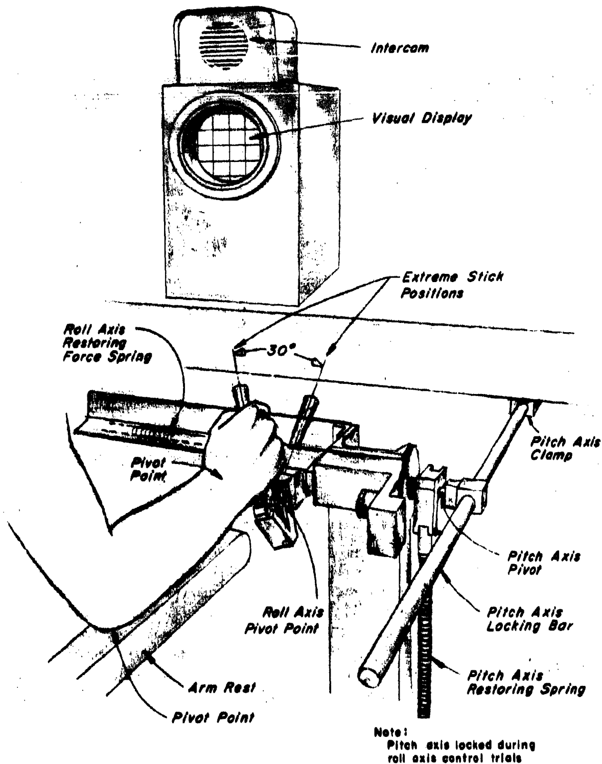
FIGURE 24. STICK MANIPULATOR
