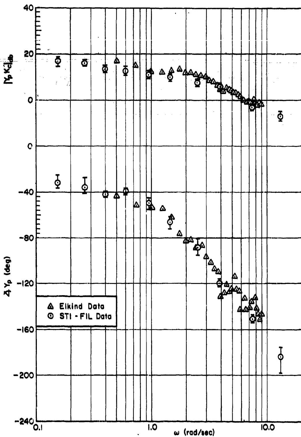
Figure 29. Comparison of Y_0 = K_0 Data with Elkind Data
