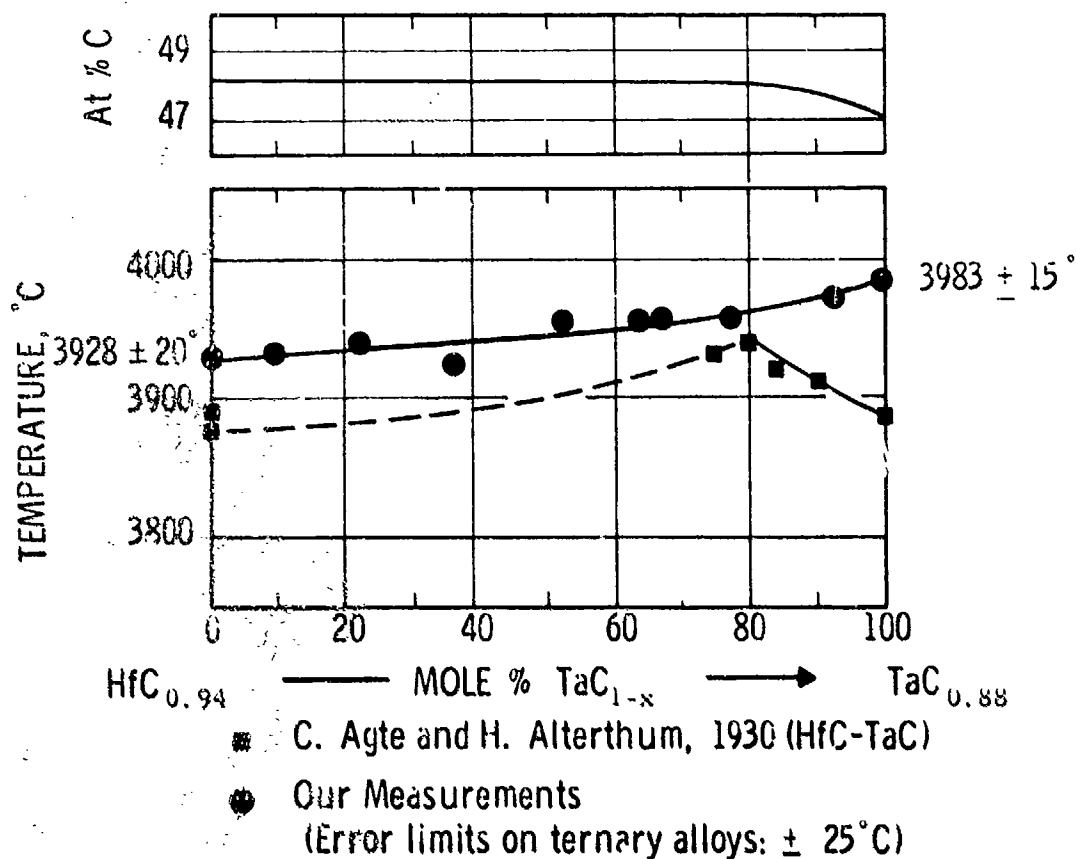
Figure 3. Maximum Solidus Temperatures of the Crystal Solution (\text{Ta}, \text{Hf})\text{C}_{1-x} Top: Concentration Line of Maximum Melting ( \pm 0.3 At%)
