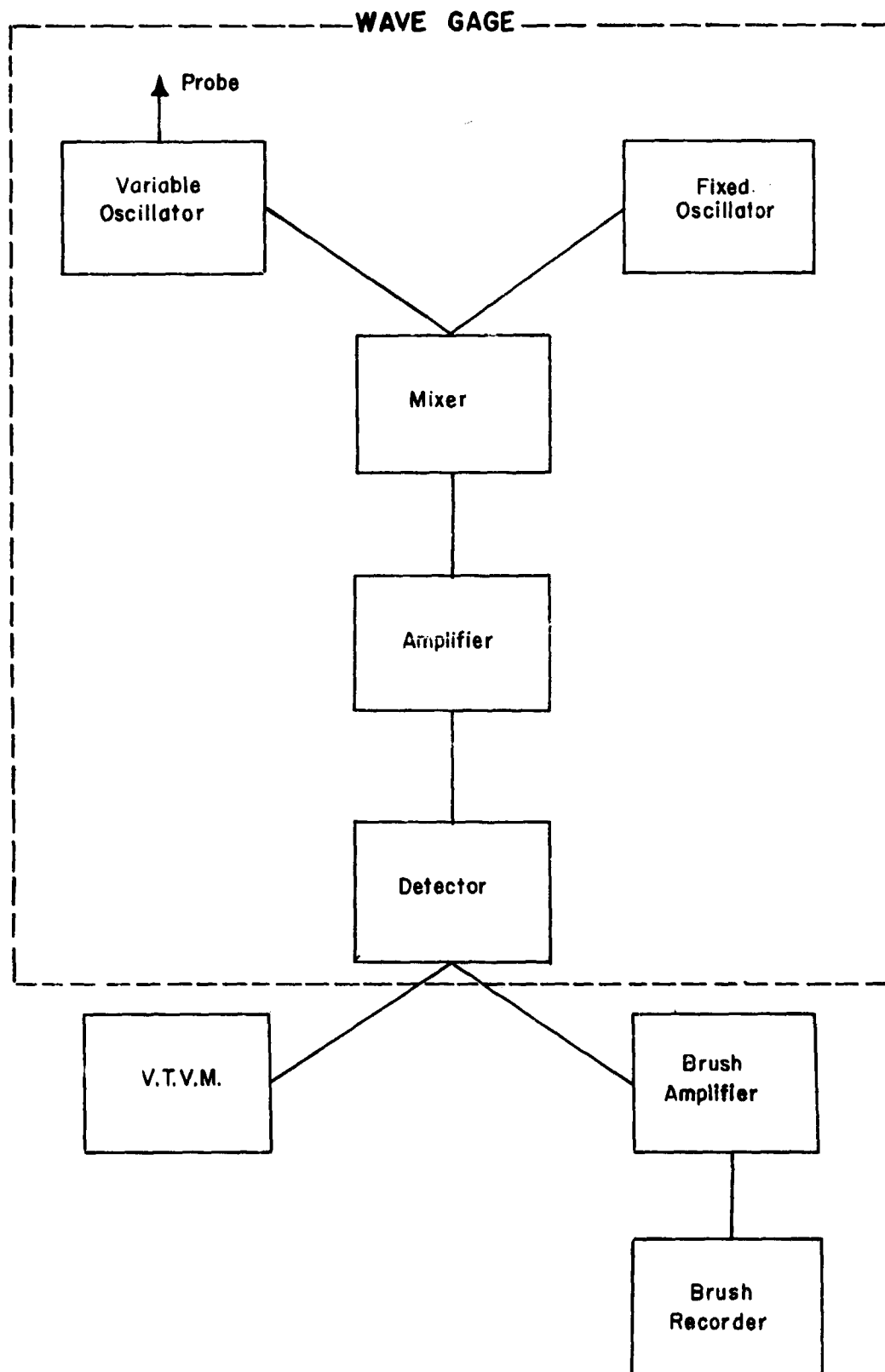
FIGURE 1. BLOCK DIAGRAM FOR ELECTRONIC WAVE GAGE AND RECORDING EQUIPMENT
