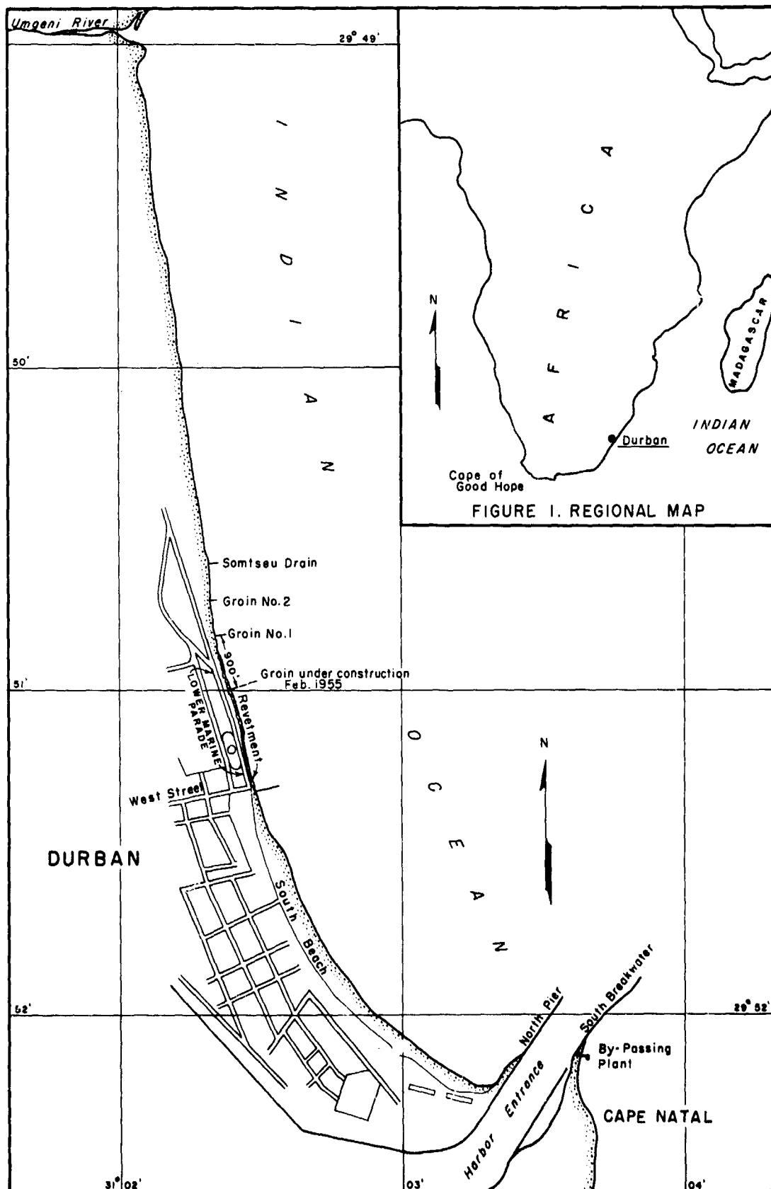
FIGURE 2. SHORE FEATURES AT DURBAN, SOUTH AFRICA
