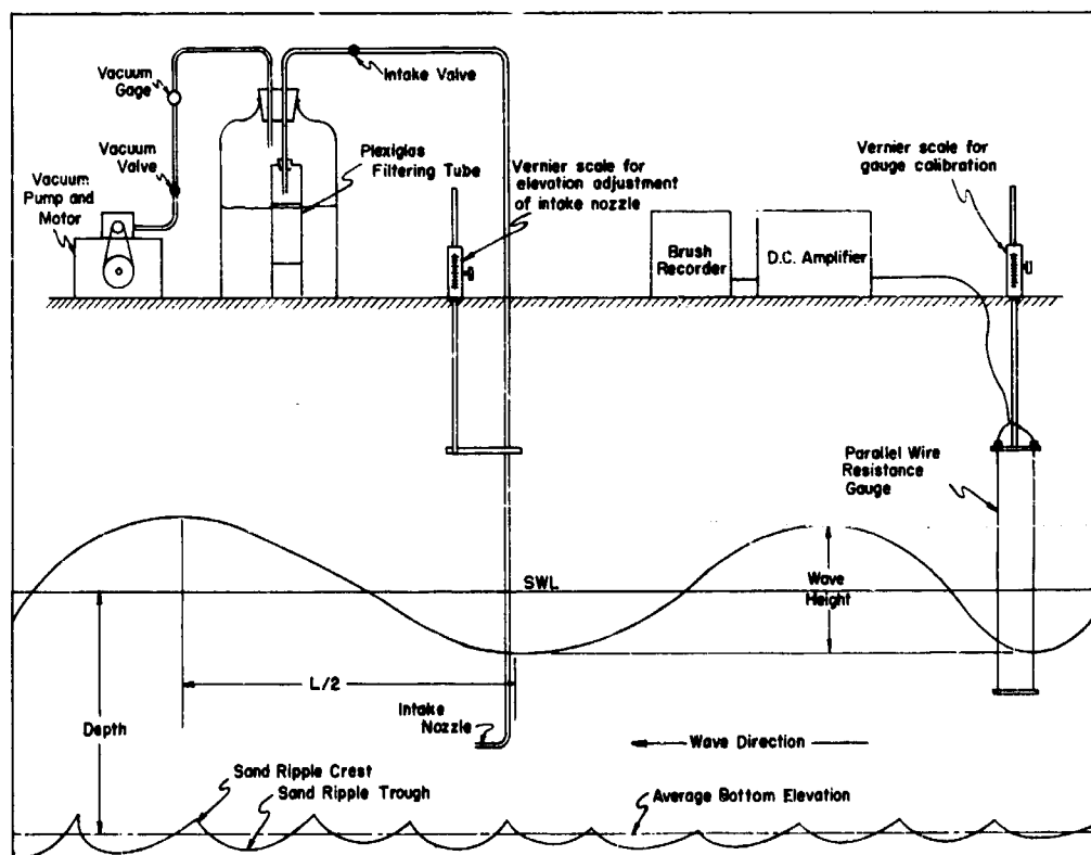
FIGURE 4 · SCHEMATIC DIAGRAM OF TEST SET-UP
