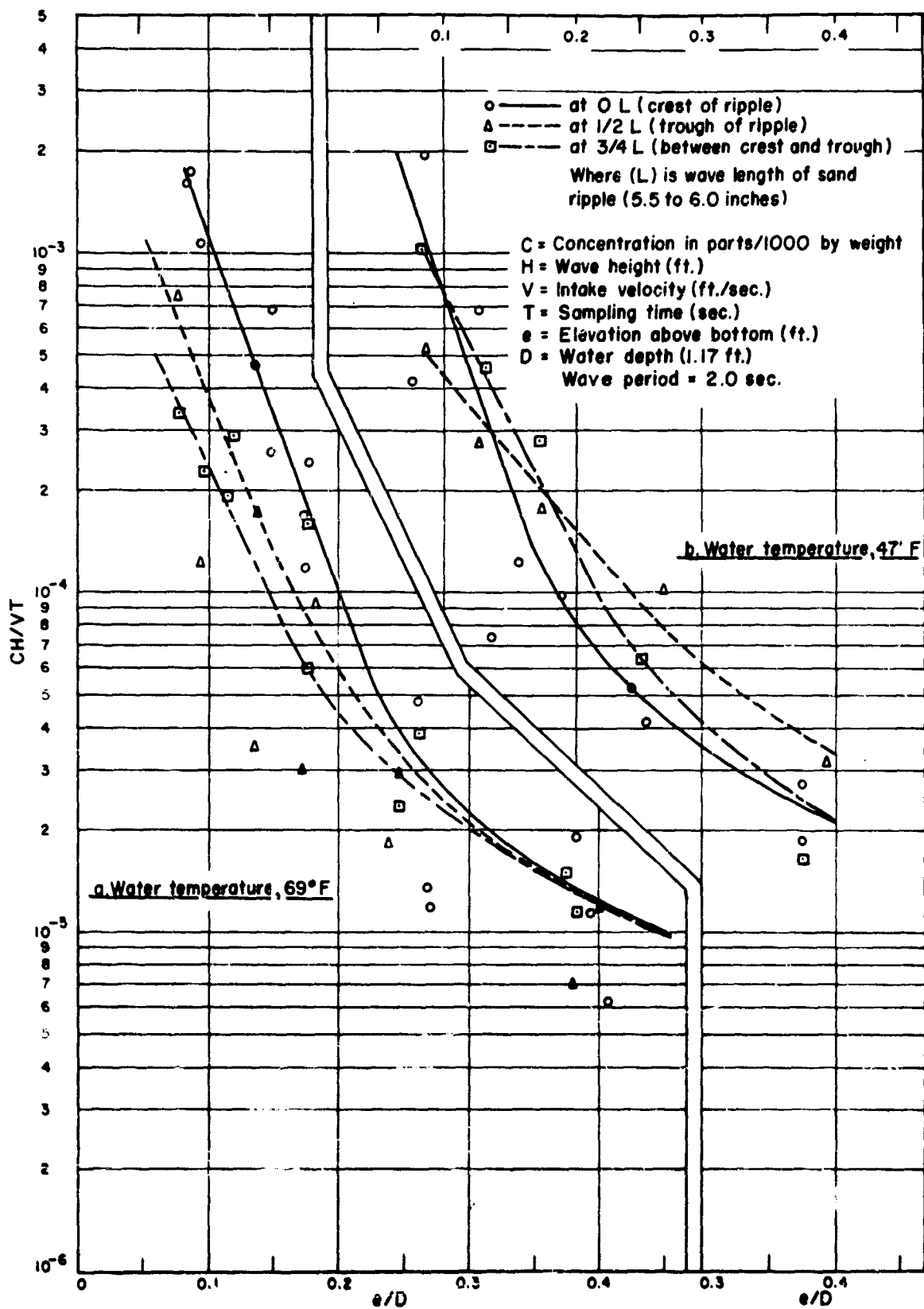
FIGURE 11 - SUSPENDED SEDIMENT CONCENTRATION AT THREE NOZZLE POSITIONS ALONG THE SAND RIPPLE PROFILE
