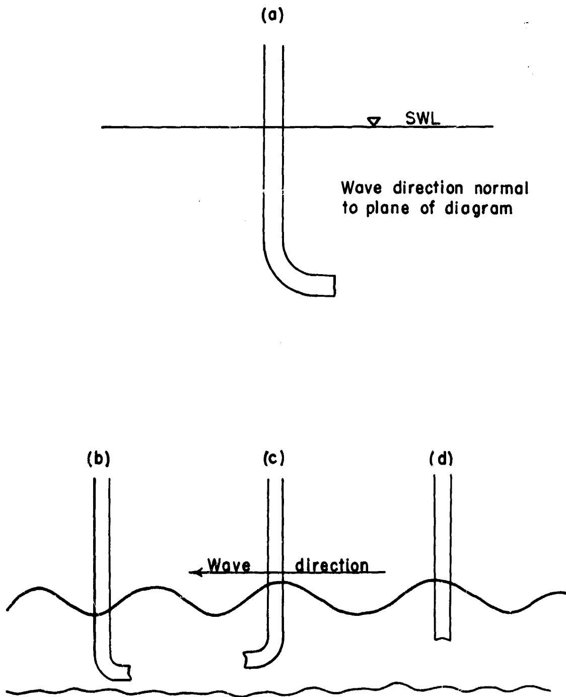
FIGURE 10. INTAKE NOZZLE ORIENTATIONS RELATIVE TO WAVE DIRECTION
