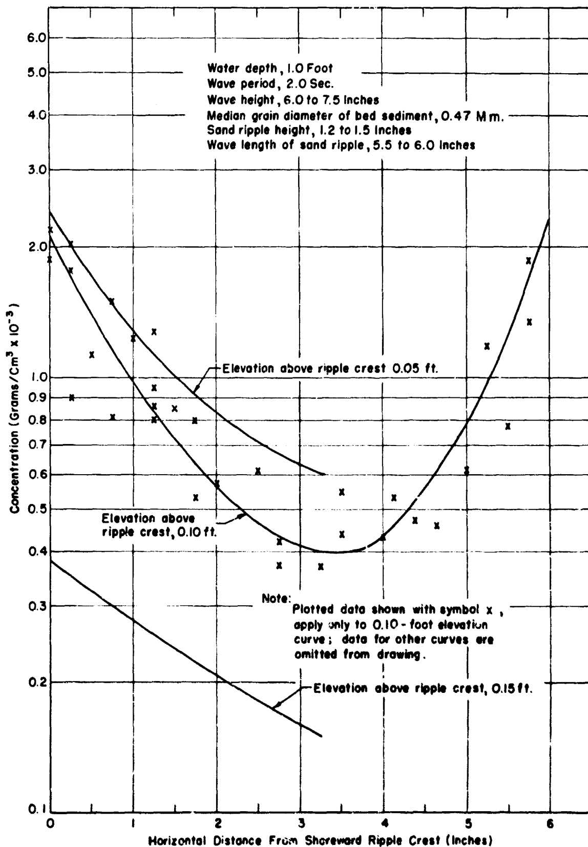
FIGURE 12 · SUSPENDED SEDIMENT CONCENTRATION VS HORIZONTAL DISTANCE FROM SAND RIPPLE CREST
