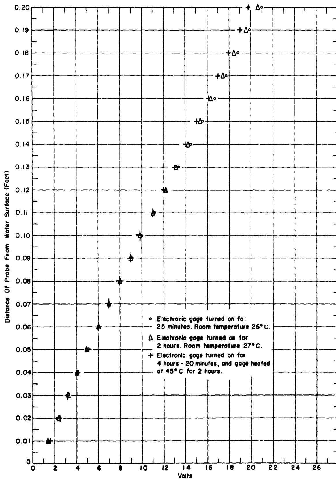
FIGURE 4 · CALIBRATION DRIFT DUE TO TEMPERATURE CHANGE
