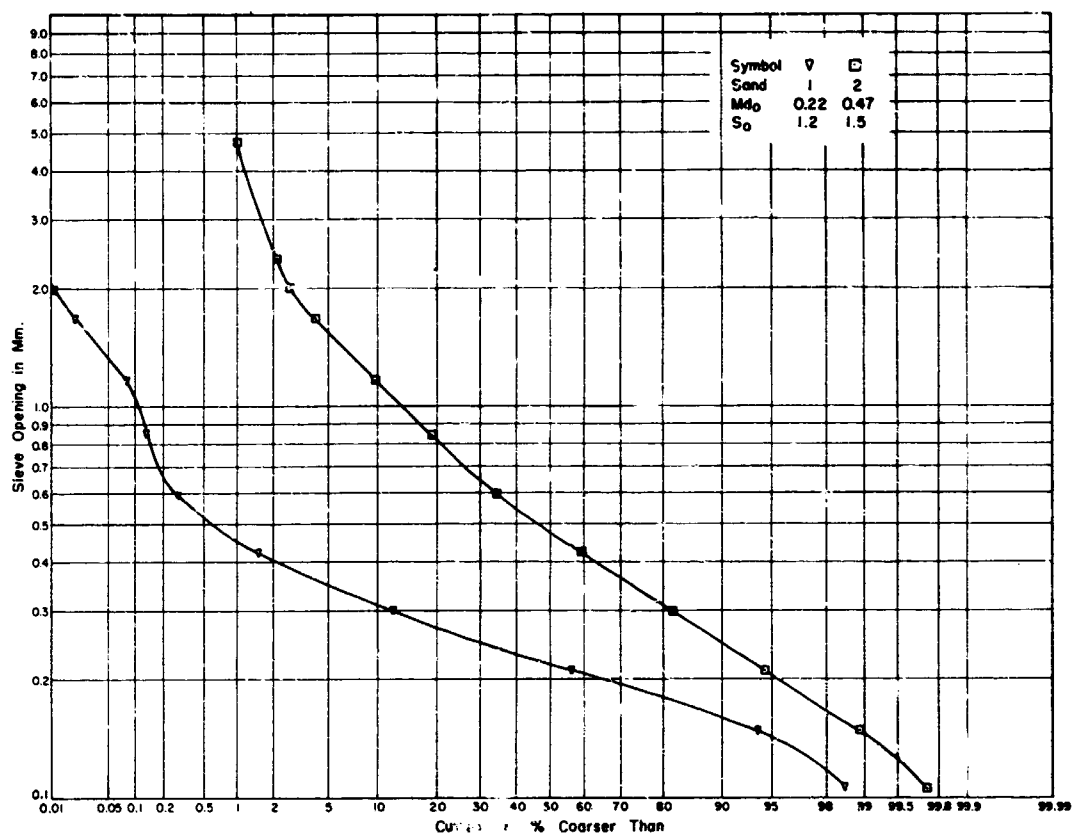
FIGURE 3 · SIZE FREQUENCY BY WEIGHT OF BED MATERIALS USED IN THE STUDY
