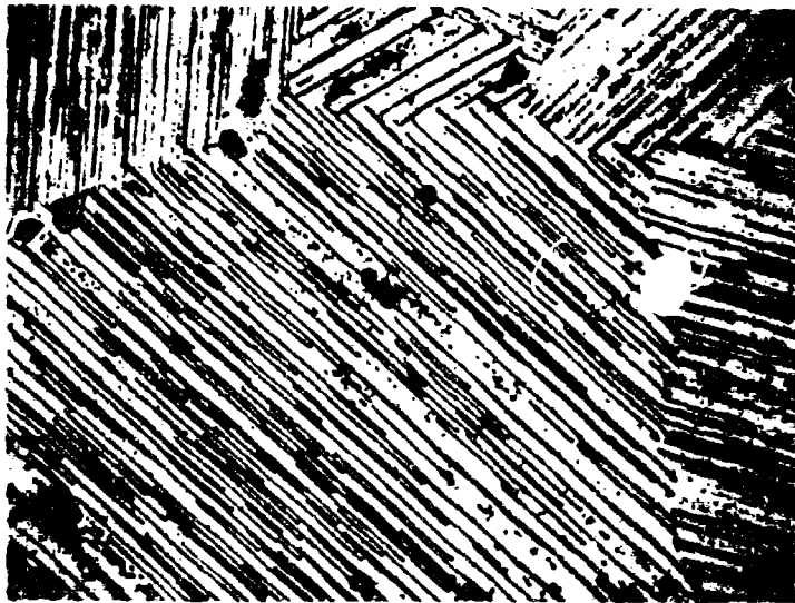
Figure 20c. Hf-C (14.9 At% C) Sample from Figure 20a X500 Re-equilibrated for 1 Hour at 2300°C. \alpha -Hf-Solid Solution with Oriented Precipitations of Monocarbide Within the Grains and Small Amounts of Excess Monocarbide Distributed Along the Grain Boundaries.
