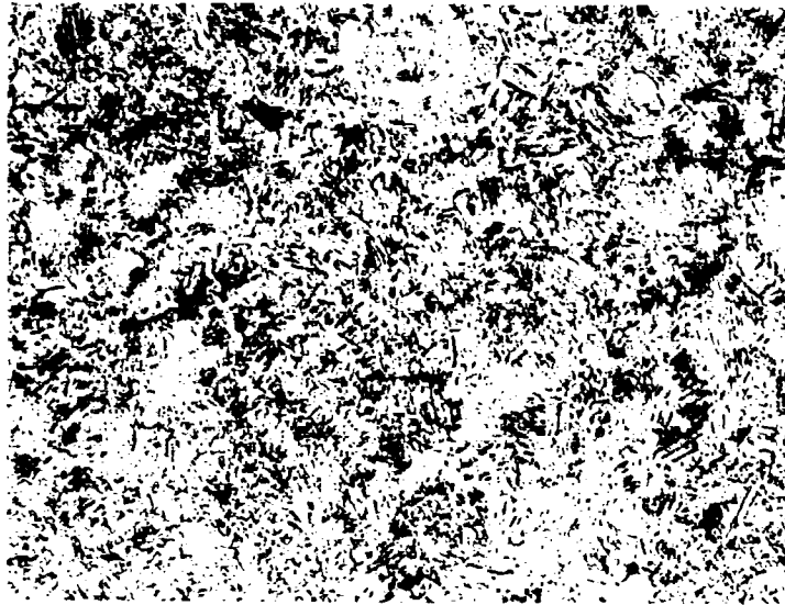
Figure 20b Hf-C (14.9 At% C). Sample from Figure 20a X450 Re-equilibrated for 15 Minutes at 2300°C. Carbide Phase in Process of Dissolution
