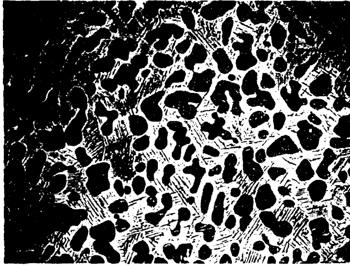
Figure 19a. Hf-C (13 At% C), Quenched from 2450°C. X100 Monocarbide (Dark, with Metal Precipitations), in a Matrix of Metal-Rich Melt ( \alpha -Hf-ss with Carbide Precipitations).
