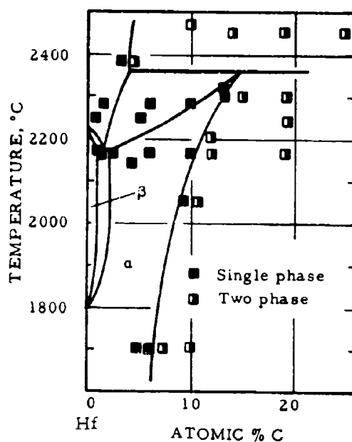
Figure 17. Metal-Rich Portion of the System Hafnium-Carbon: Qualitative Results of the Metallographic Examinations of Equilibrated and Quenched Alloys.
