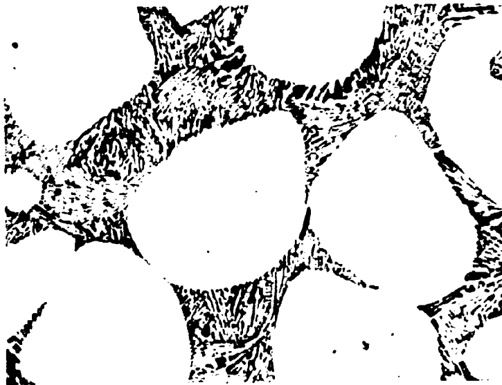
Figure 28b. Hf-C (39.5 At% C), Quenched from 3500°C. X1000
