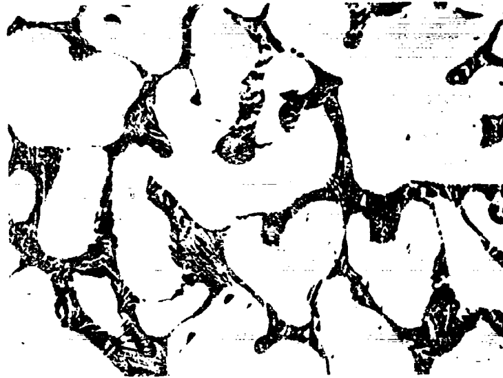
Figure 28a. Hf-C (56.1 At% C), Quenched from 3500°C. X500
