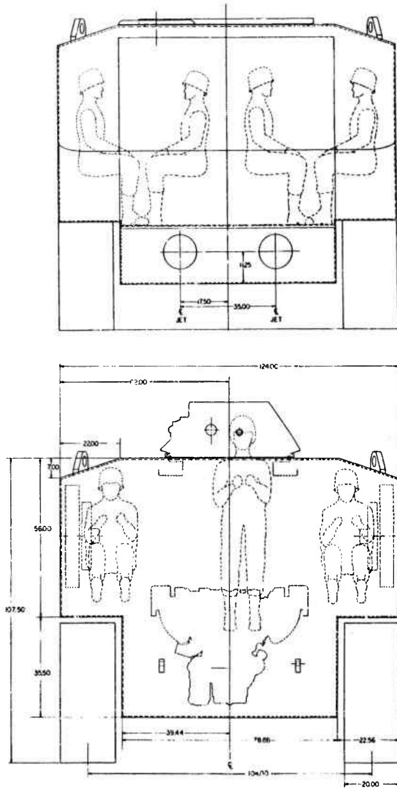
Figure 5-11 LVTPX12 With Bottom Jets - End Views
