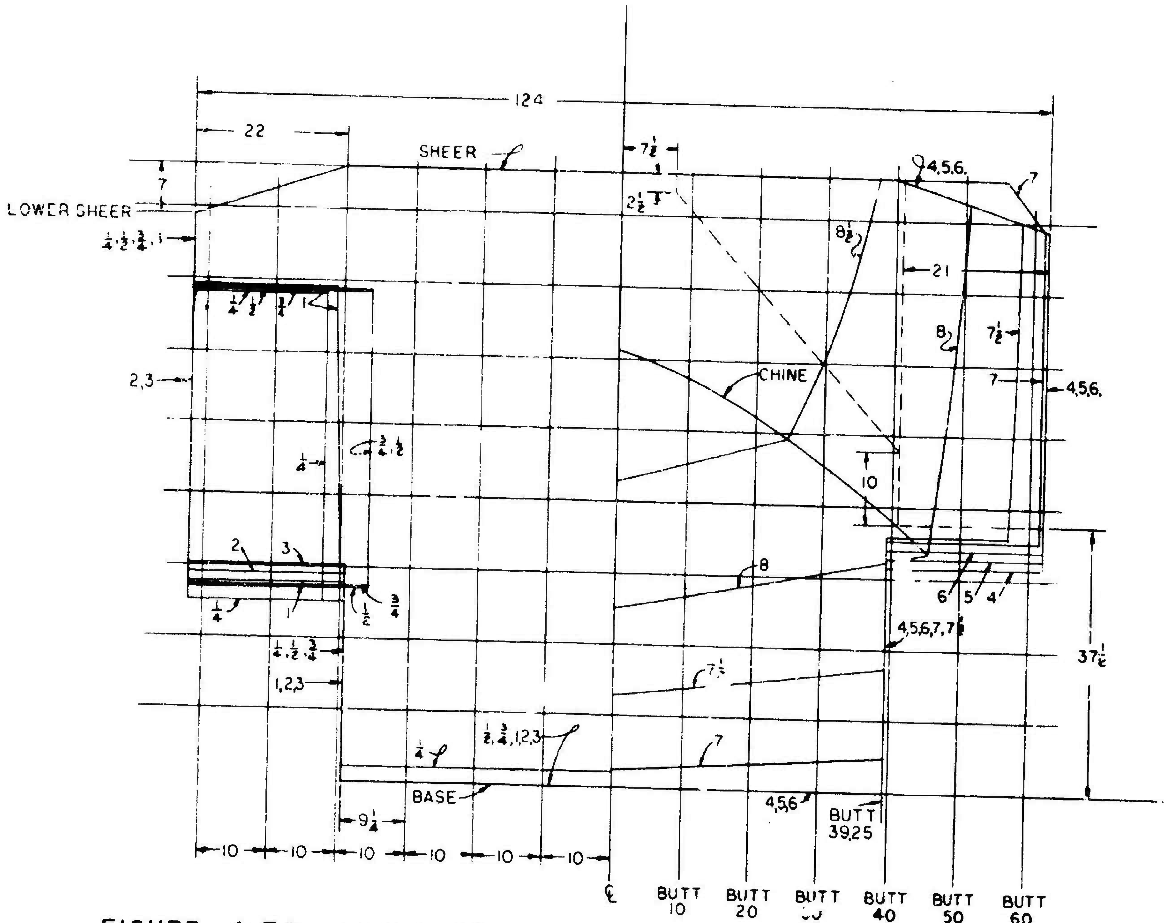
FIGURE 4-72 LINES DRAWING OF PROPELLER DRIVEN VEHICLE
