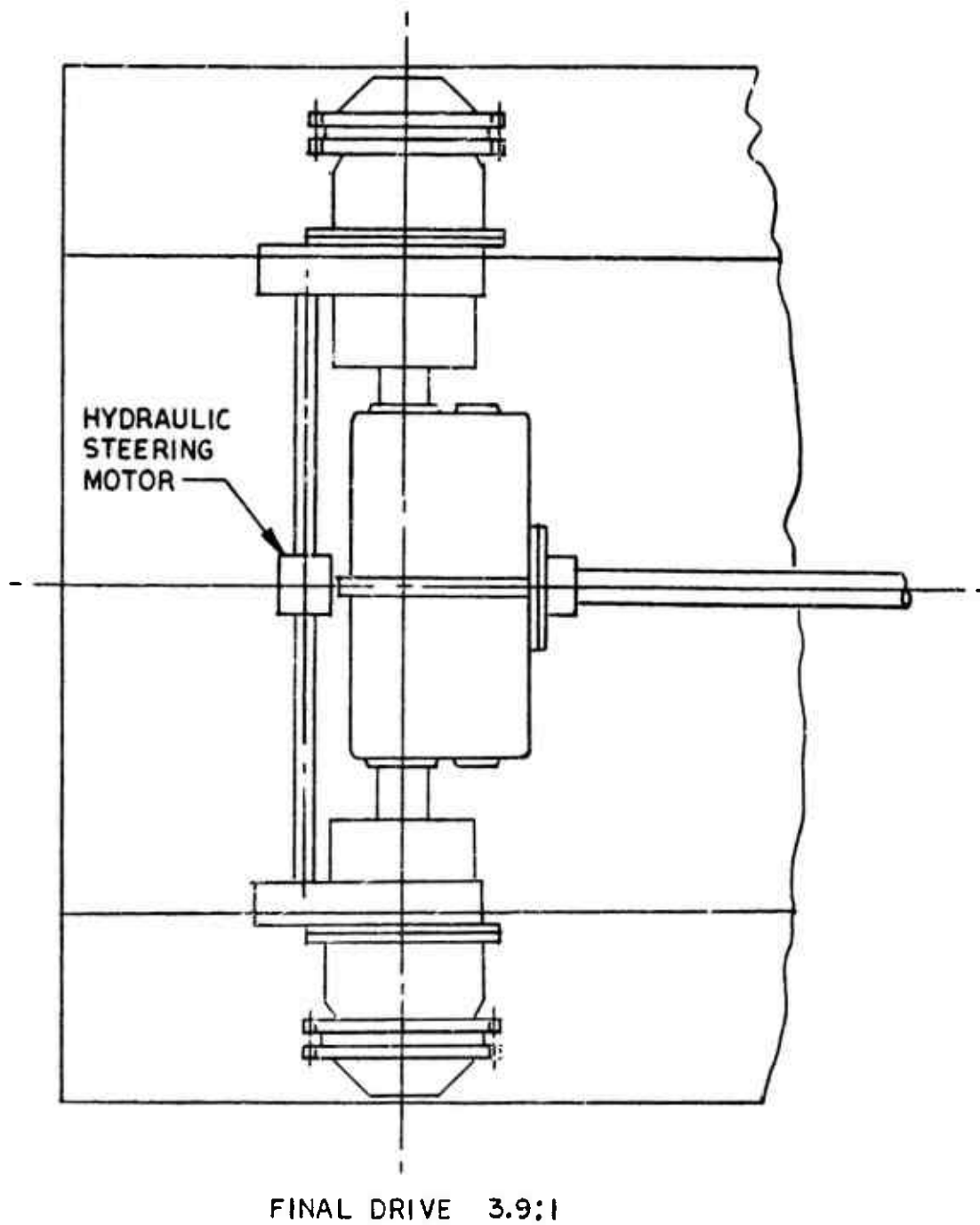
Figure 8-18 Buehler Transmission Concept
