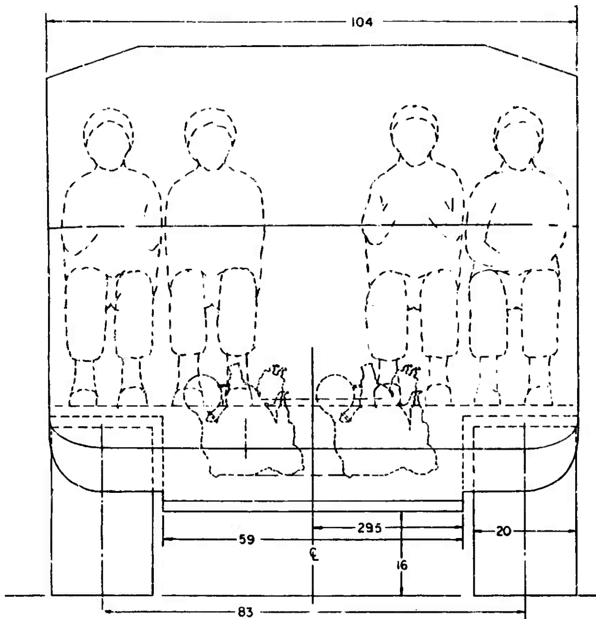
Figure 5-5 Narrow Track-Propelled Vehicle - End View
