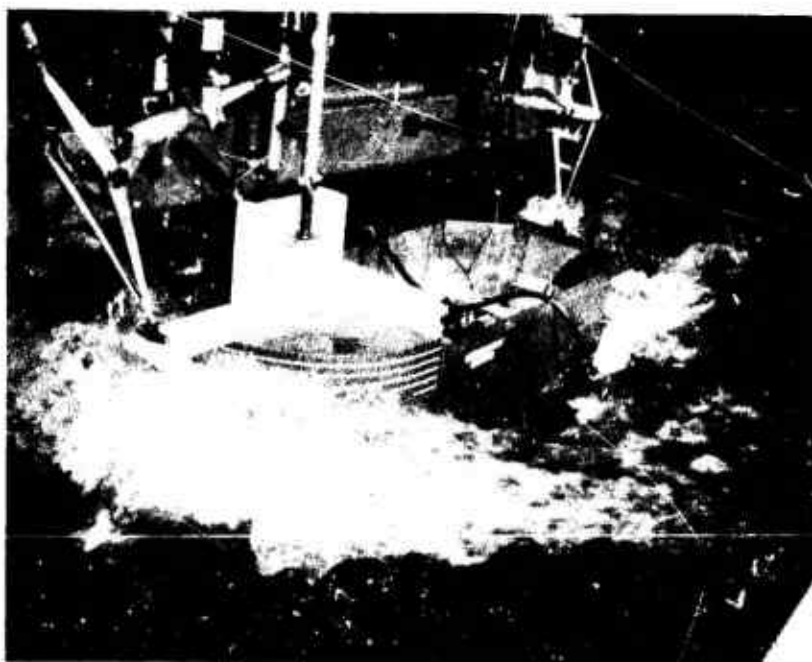
Figure 4-65 10 MPH, Trimmed 8 Inches by Bow, 43,000 Pounds - Wave 4 Inches from Deck
