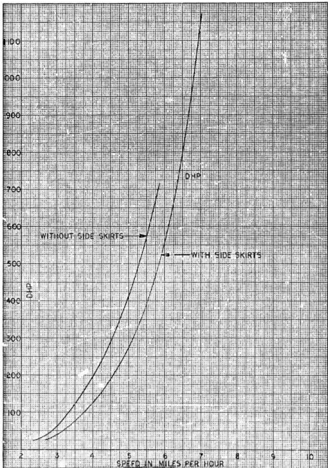
FIG. 4-49. Side Skirts
