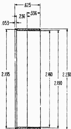
⑧ CUPRONICKEL SLEEVE
