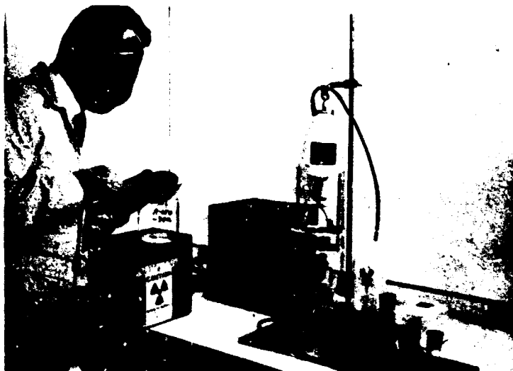
Figure 2.8 Sonic vibrator and ultrasonicator for wet-sieve particle-size analyses. (NRDL photo)
