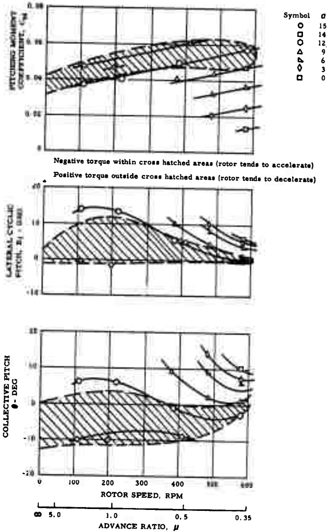
Figure 34. Control Characteristics During Pseudoconversion Test
