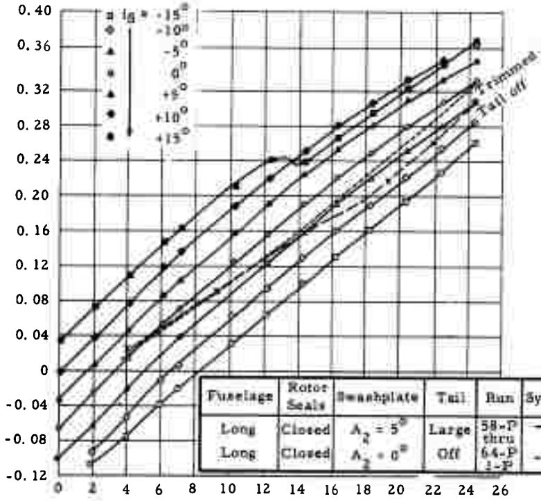
Figure 55. Lift and Pitching Moment Characteristics
