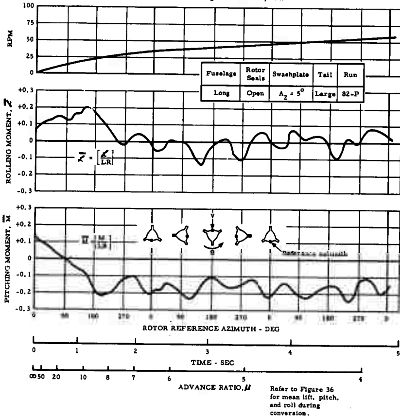
Figure 37. Rotor/Wing Rolling and Pitching Moments During Acceleration From RPM = 0
