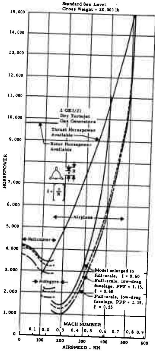
Figure 62. Full-Scale Rotor/Wing Performance
