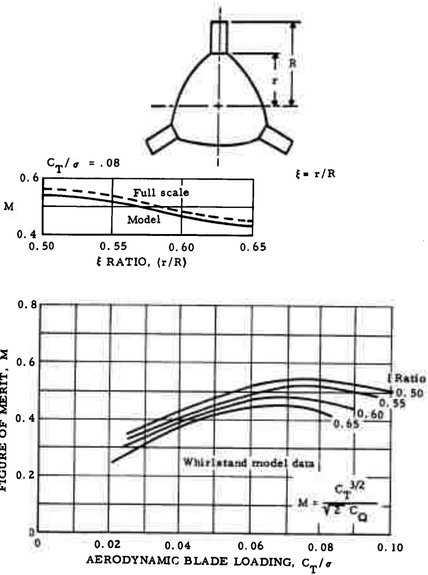
Figure 65. Hovering Figure of Merit
