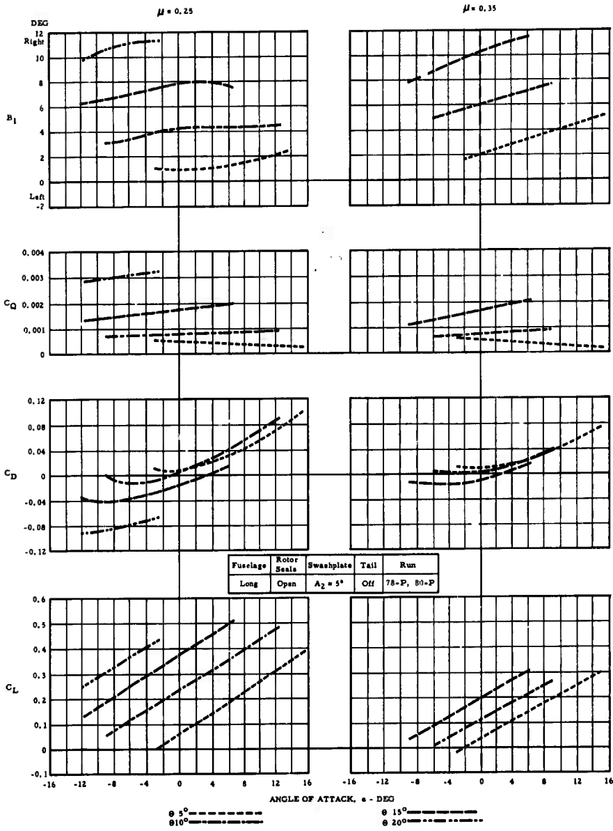
Figure 26. Powered Rotor Aerodynamic Characteristics, A_2 = 5^\circ
