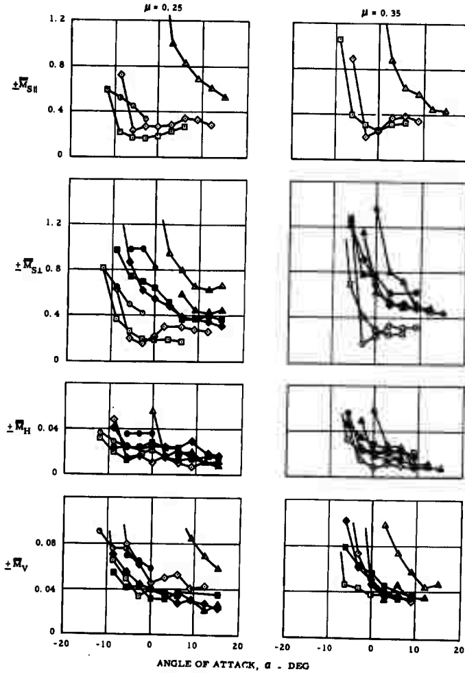
Figure 29. Blade Root and Shaft Alternating Bending Moments
