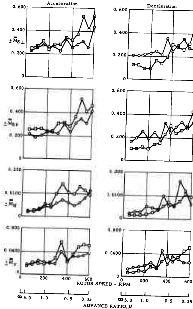
Figure 40. Blade Root and Shaft Alternating Bending Moments During Automatic Conversion
