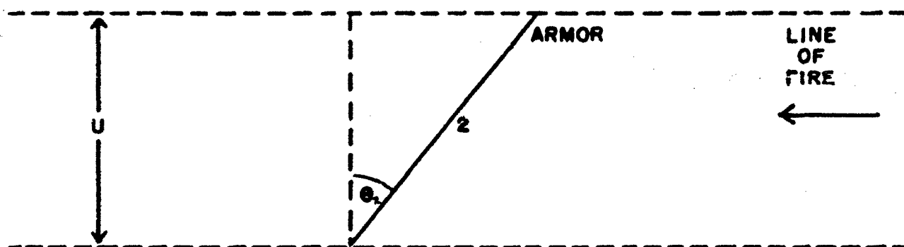
FIG. 4. ARMOR AT OBLIQUITY TO LINE OF FIRE
