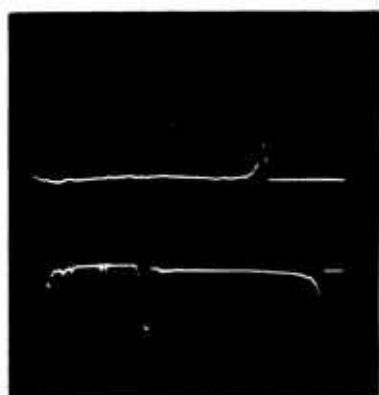
100 \mu sec/cm, 0.5 v/cm Top and Outside Gauges
