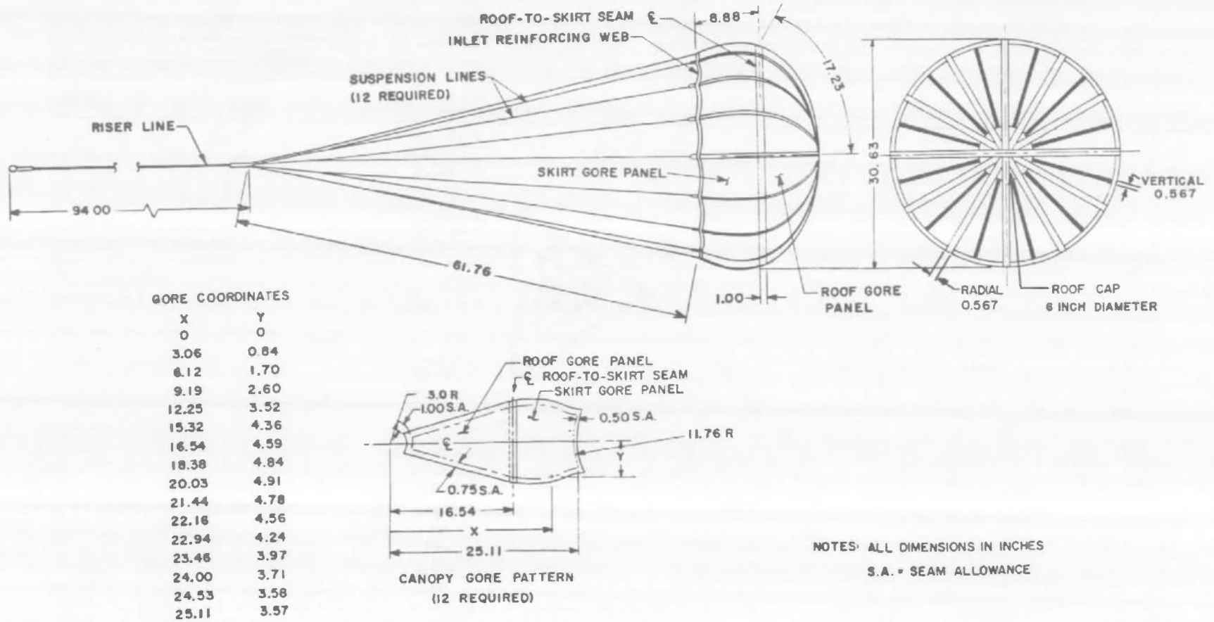
Fig. 10 Parasonic Parachute Details, Configuration 14
