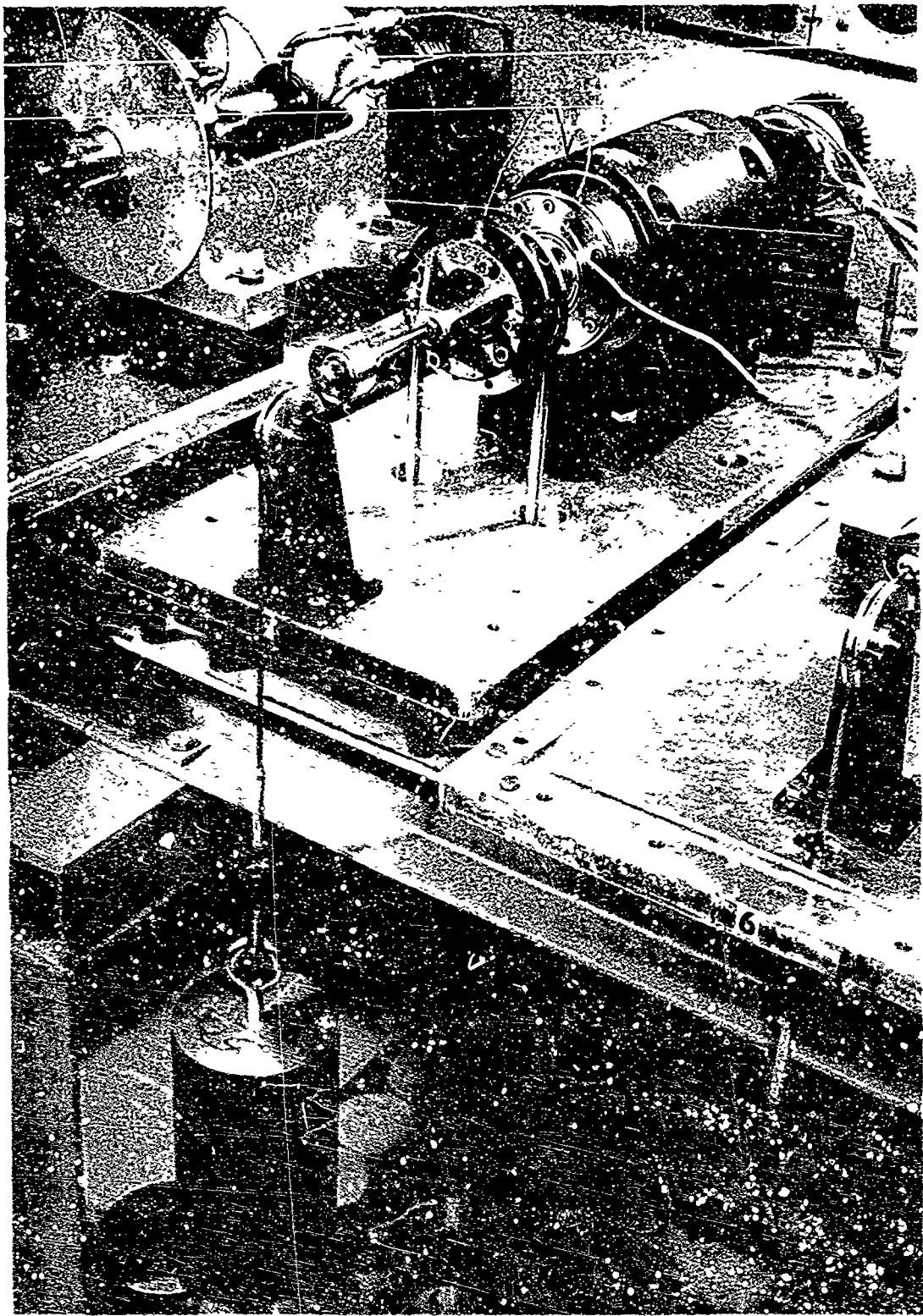
FIGURE 7 30,000 RPM TEST SPINDLE
