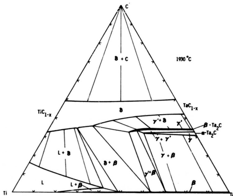
Figure 53. Ti-Ta-C: Isothermal Section at 1930 °C
