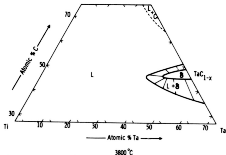
Figure 63. Ti-Ta-C: Isothermal Section at 3800°C
