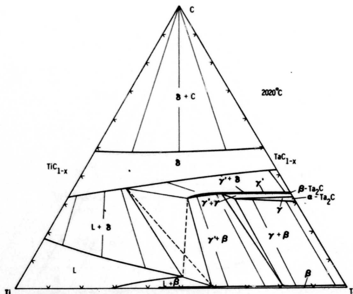
Figure 54. Ti-Ta-C: Isothermal Section at 2020 °C
