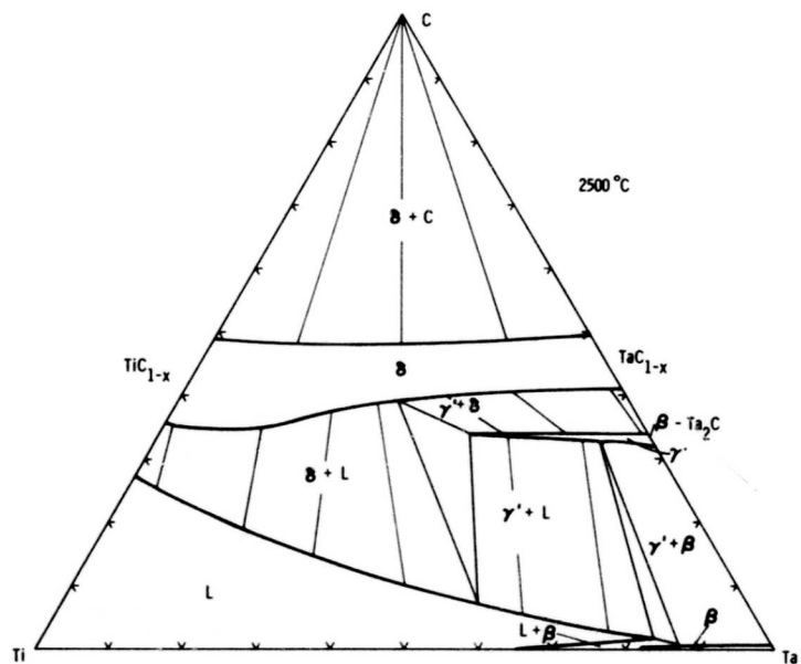
Figure 57. Ti-Ta-C: Isothermal Section at 2500°C
