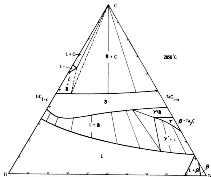
Figure 59. Ti-Ta-C: Isothermal Section at 2850°C
