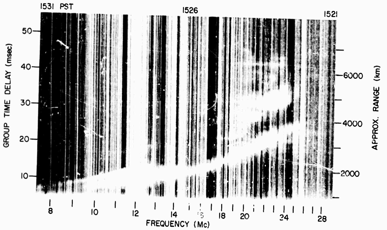
Z RECORDS, 12 APR 1965, 122° BEARING
