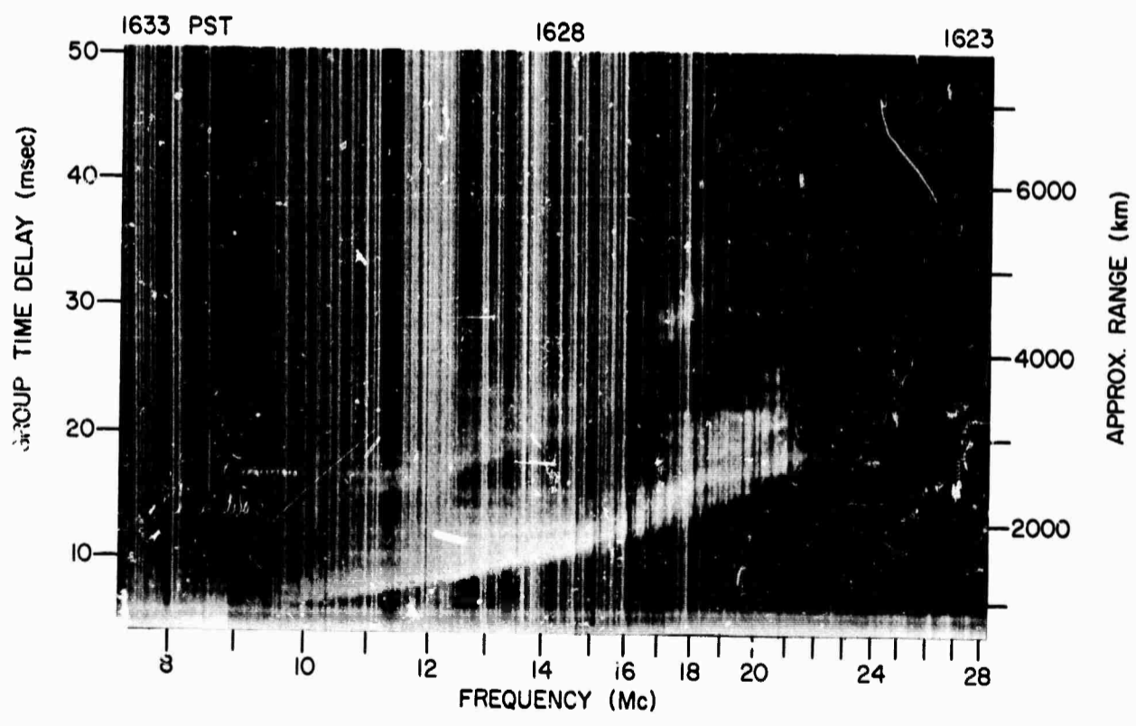
Z RECORD, 16 FEB 1965, 122° BEARING
