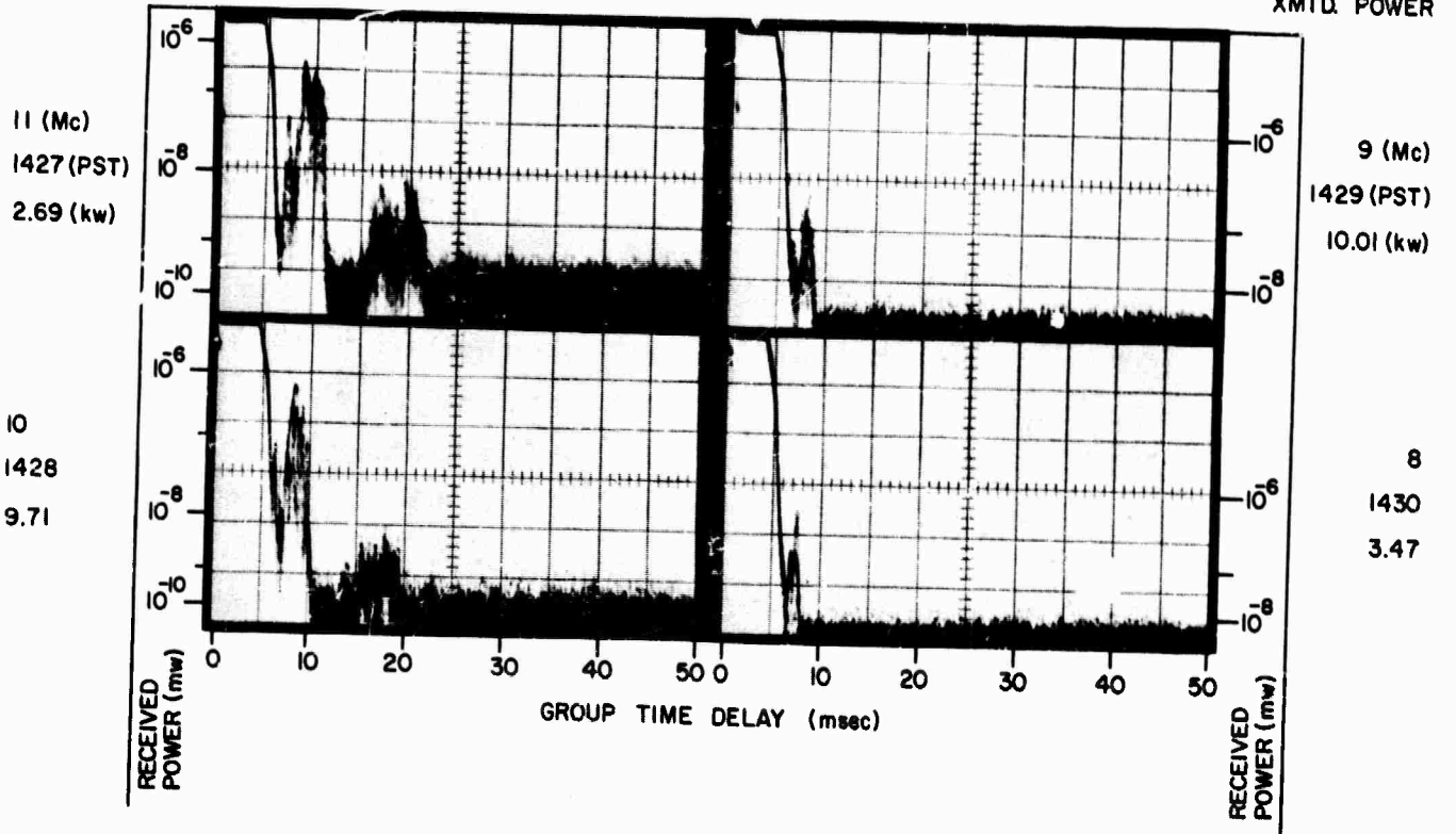
A RECORDS, 9 MAR 1965, 302° BEARING
