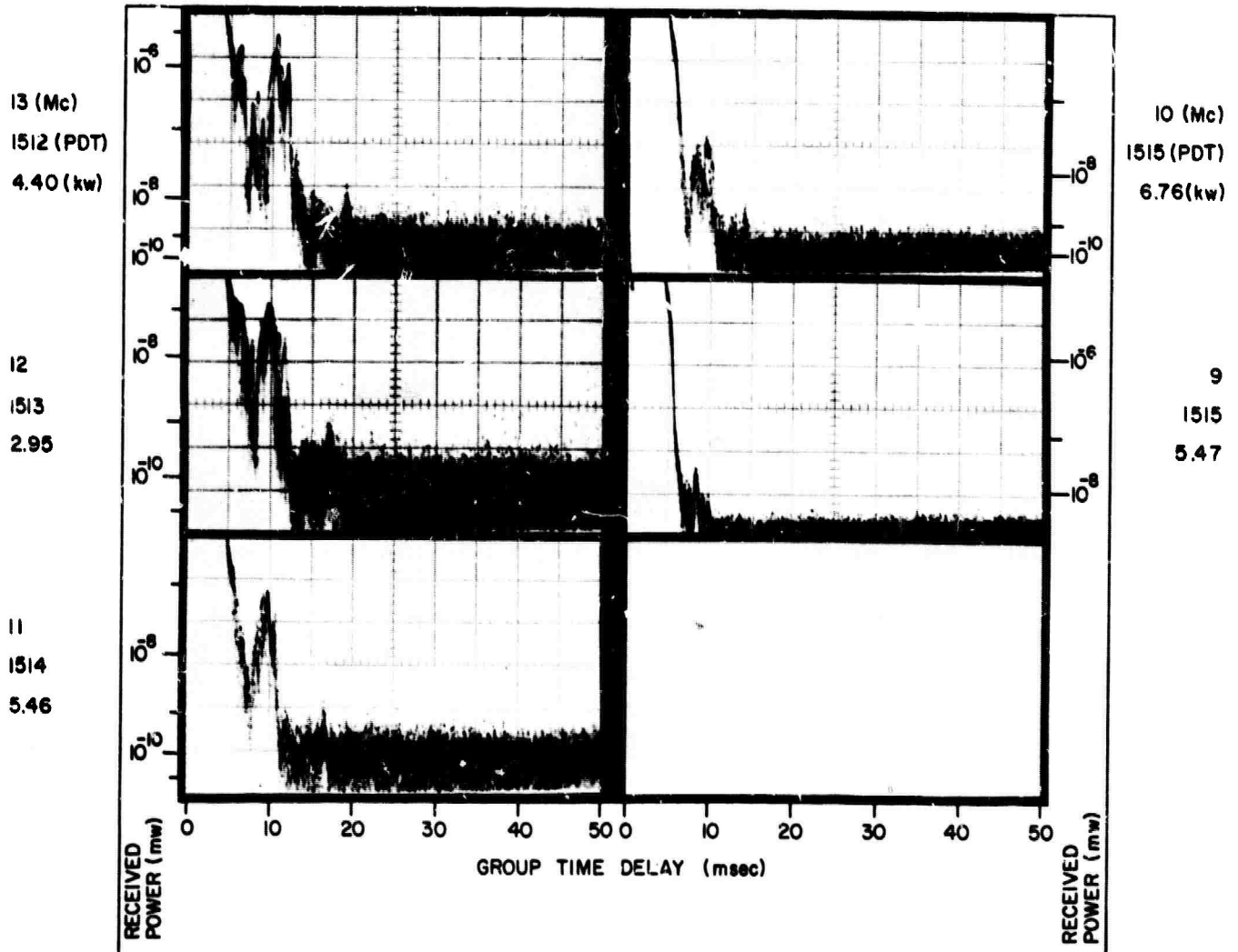
A RECORDS, 28 APR 1965, 122° BEARING
