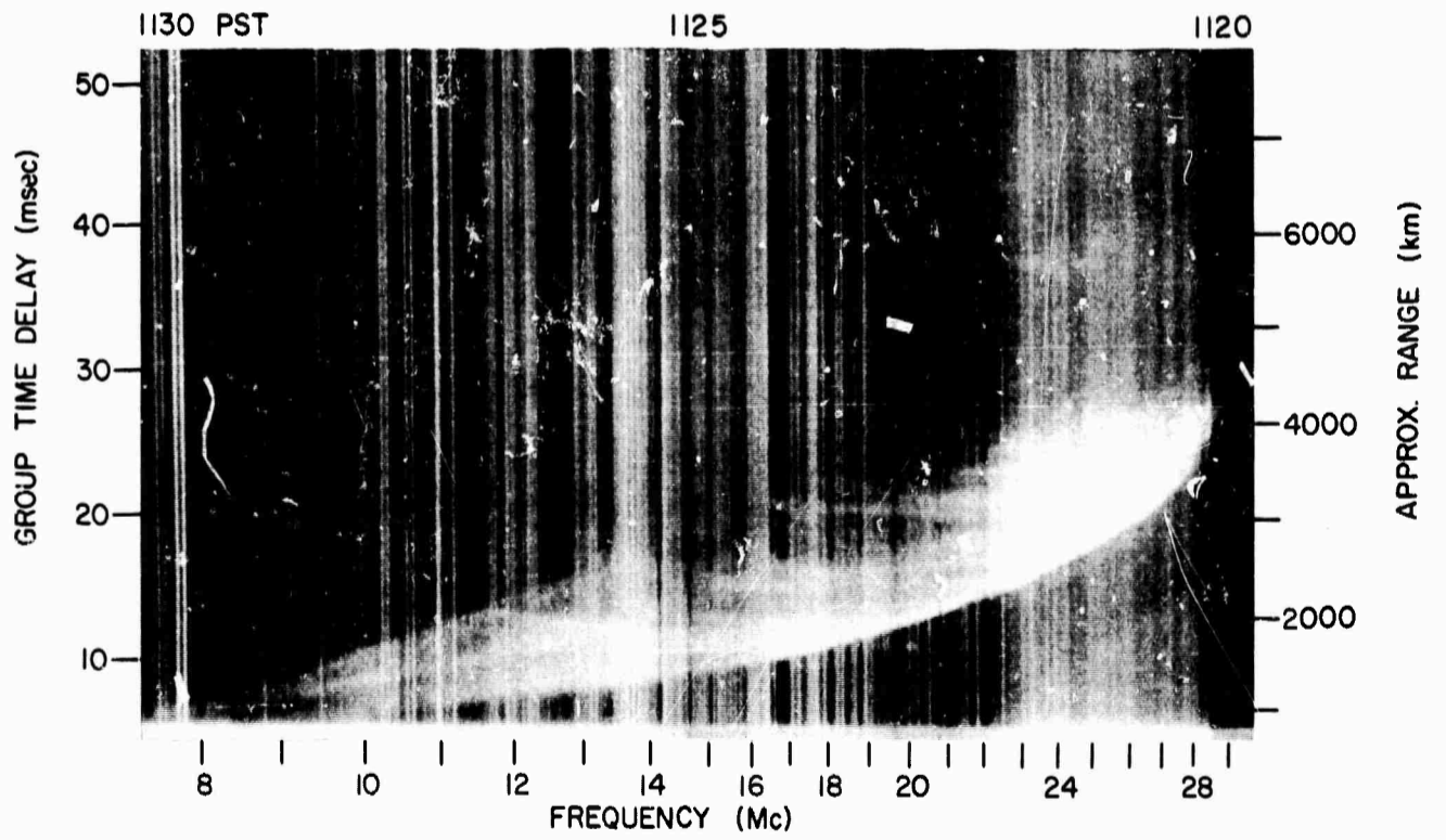
Z RECORDS, 23 FEB 1965, 122° BEARING
