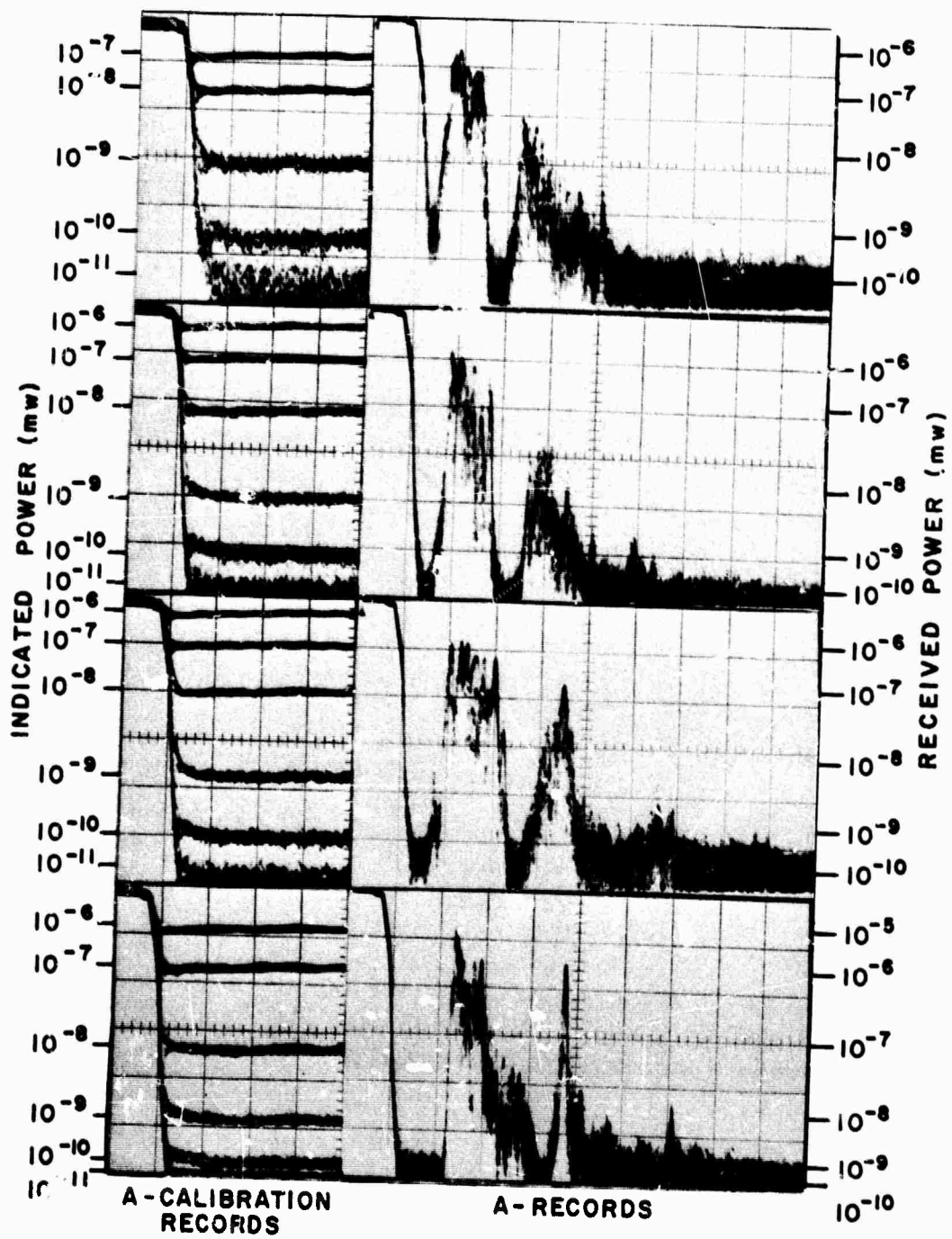
FIG. 9. EXAMPLE OF ORIGINAL A-CALIBRATIONS.
