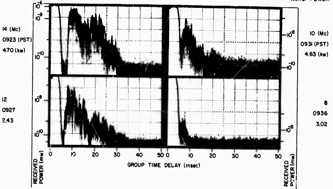
A RECORDS, 3 NOV 1964, 302° BEARING
