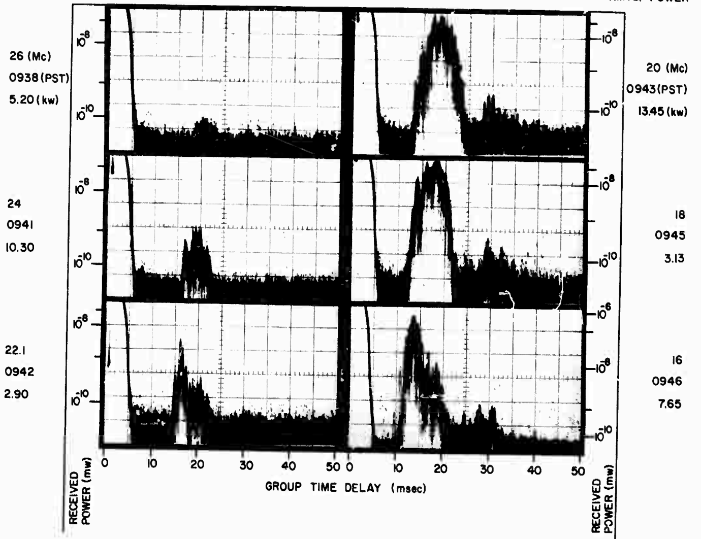
A RECORDS, 27 OCT 1964, 302° BEARING
