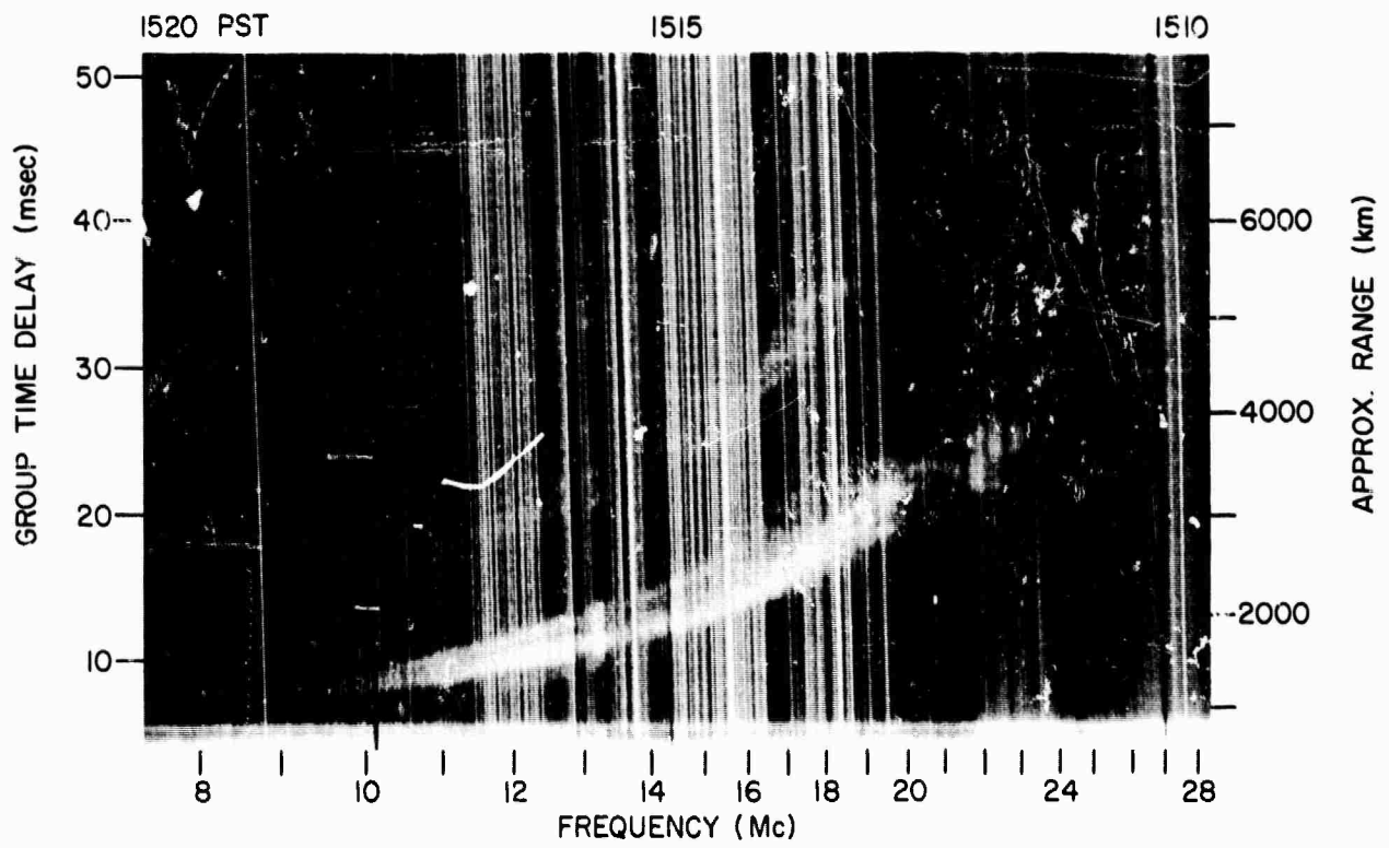
Z RECORDS, 11 MAR 1965, 302° BEARING
