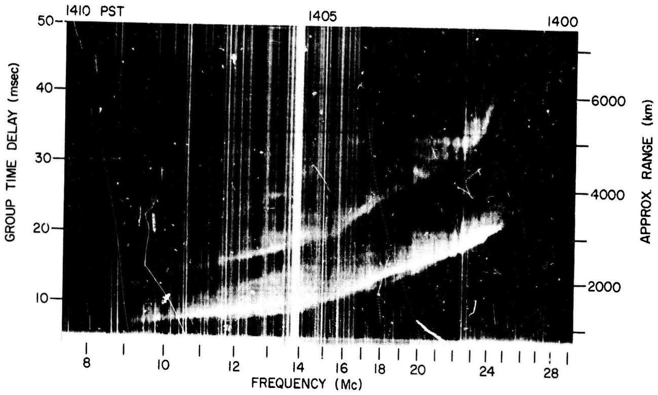
Z RECORDS, 7 NOV 1964, 302° BEARING
