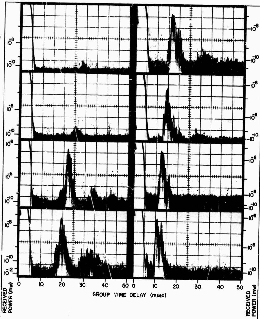
A RECORDS, 27 APR 1965, 122° BEARING
