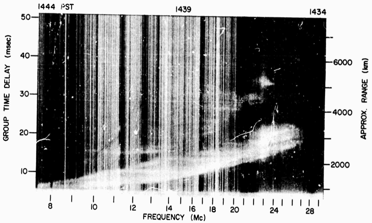
Z RECORDS, 23 FEB 1965, 122° BEARING
