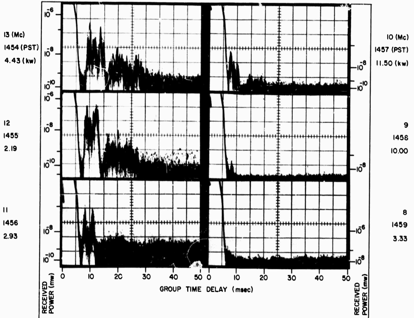
A RECORDS, 16 MAR 1965, 302° BEARING
