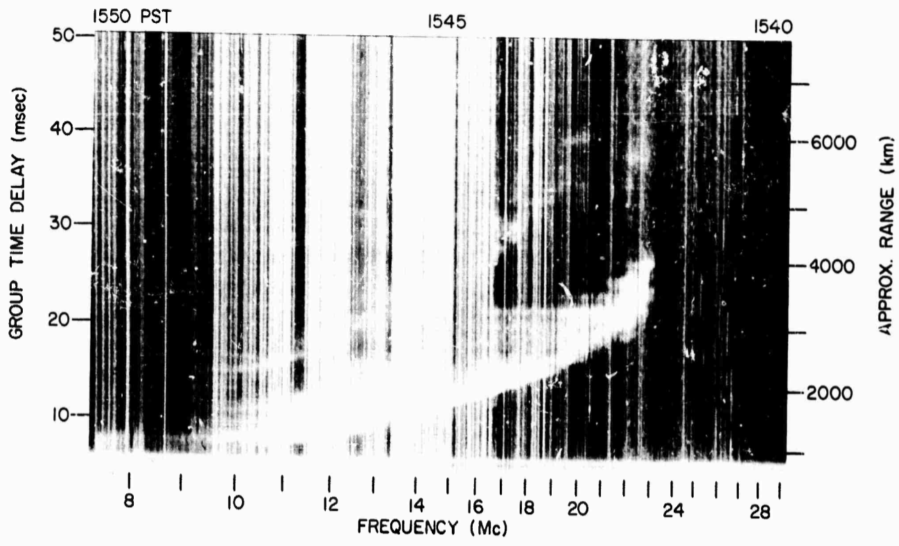
Z RECORD, 16 FEB 1965, 122° BEARING
