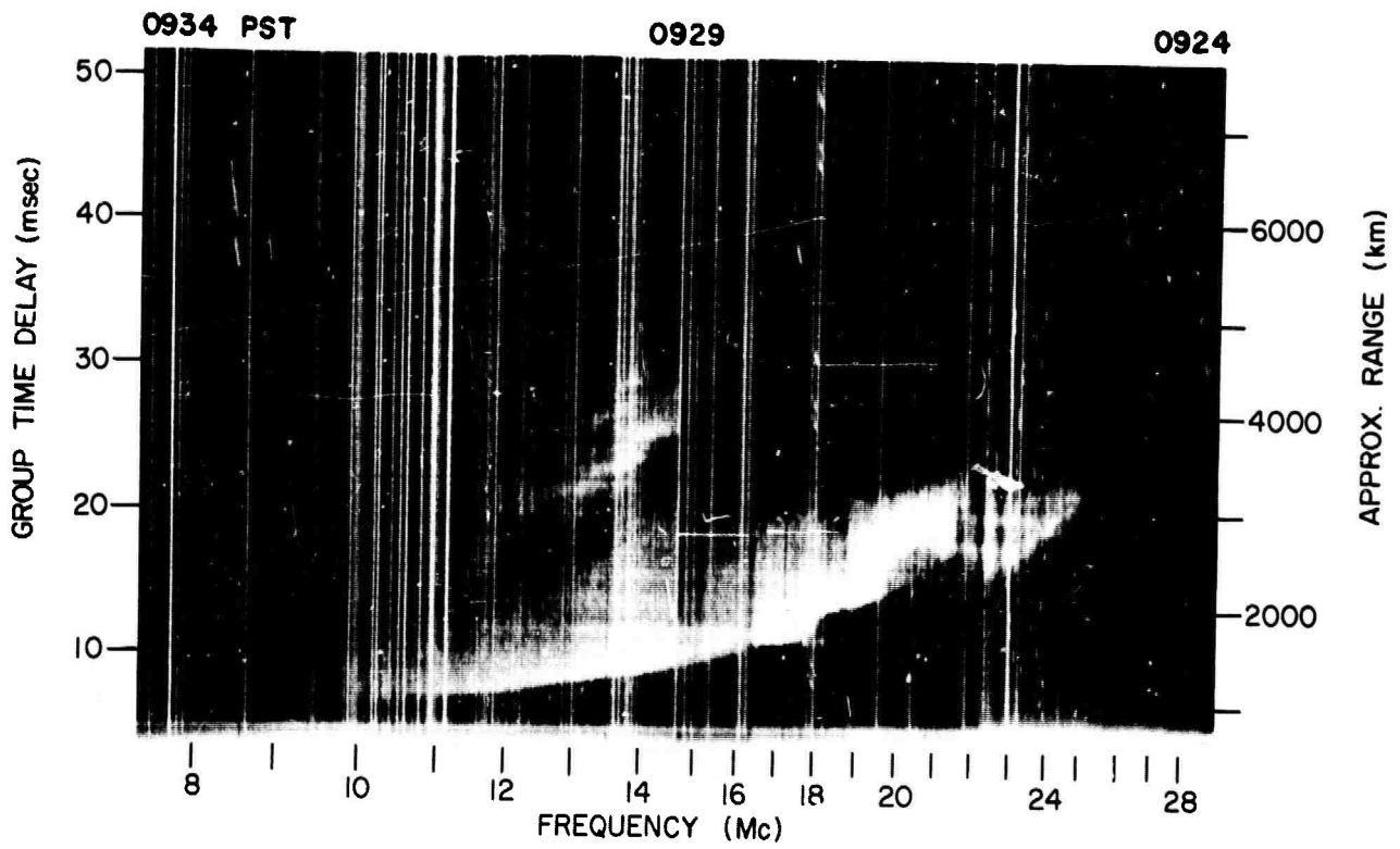
Z RECORDS, 27 OCT 1964, 302° BEARING
