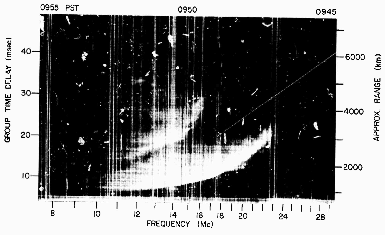
Z RECORDS, 7 NOV 1964, 302° BEARING
