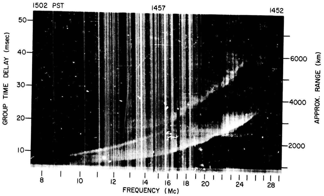
Z RECORD, 12 MAR 1965, 302° BEARING
