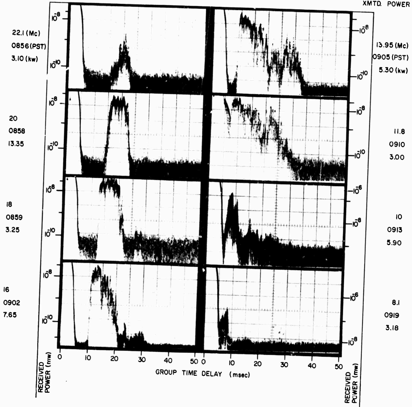
A RECORDS, 27 OCT 1964, 302° BEARING
