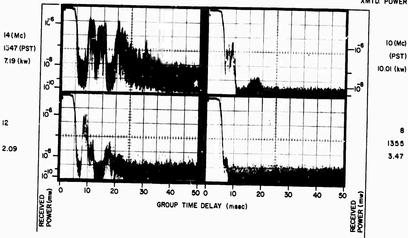
A RECORDS, 8 MAR 1965, 302° BEARING
