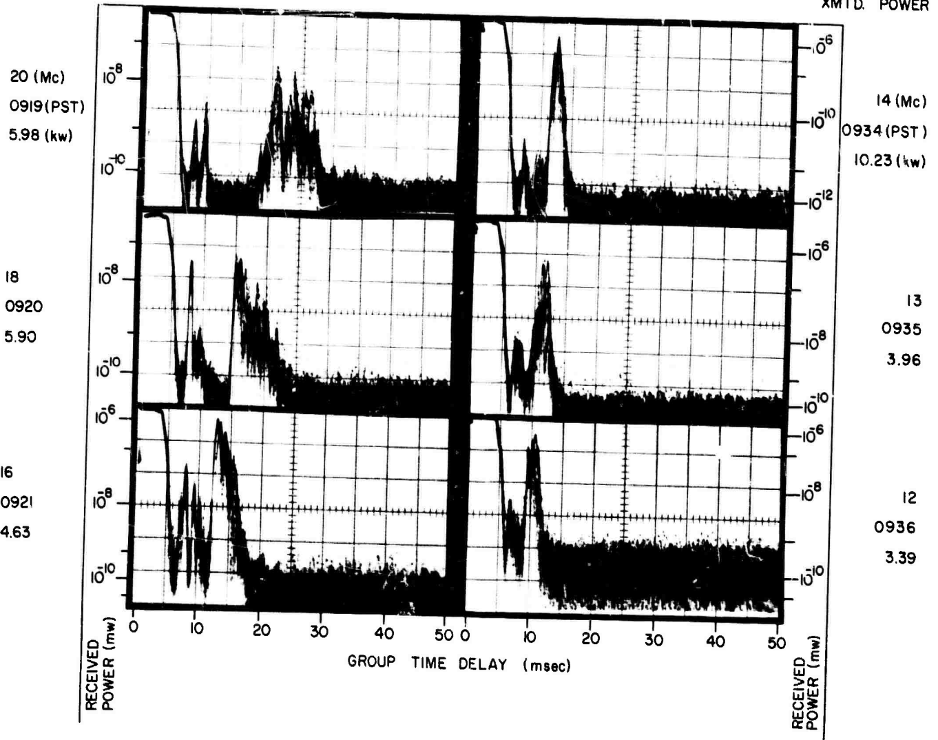
A RECORDS, 14 APR 1965, 122° BEARING
