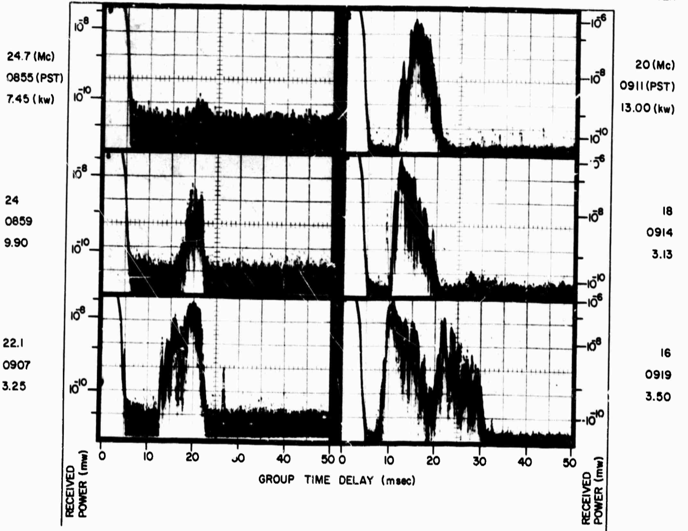
A RECORDS, 3 NOV 1964, 302° BEARING
