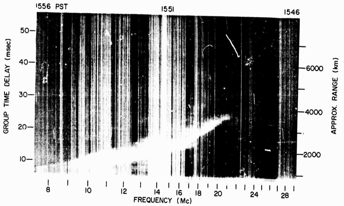
Z RECORDS, 22 APR 1965, 122° BEARING
