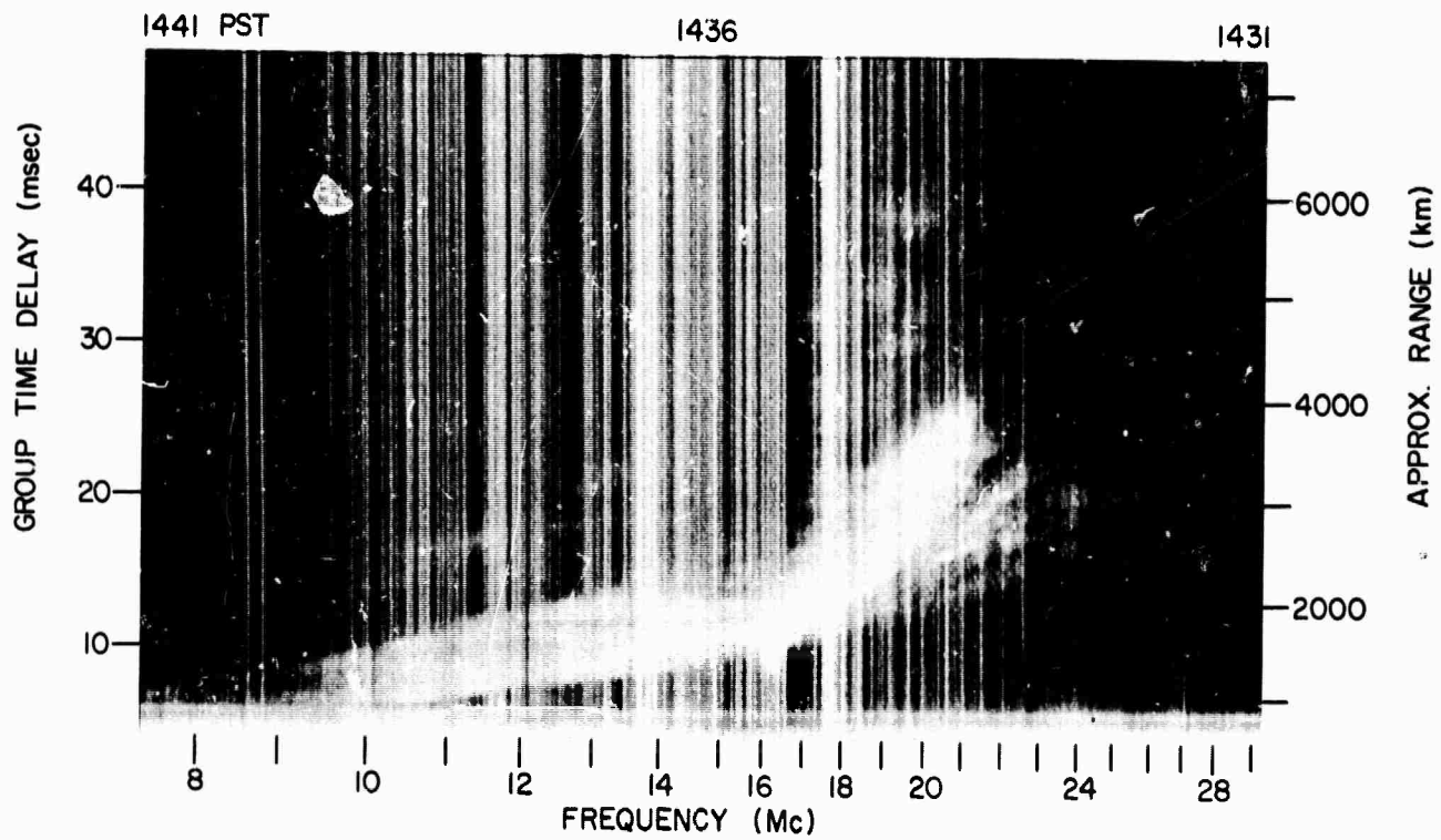
Z RECORDS, 18 FEB 1965, 122° BEARING
