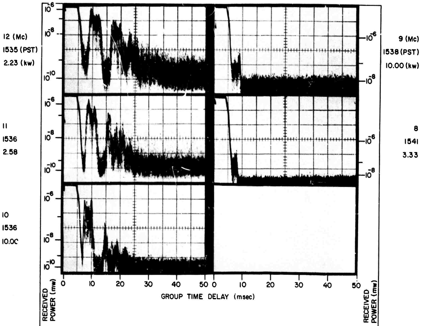
A RECORDS, 9 MAR 1965, 302° BEARING
