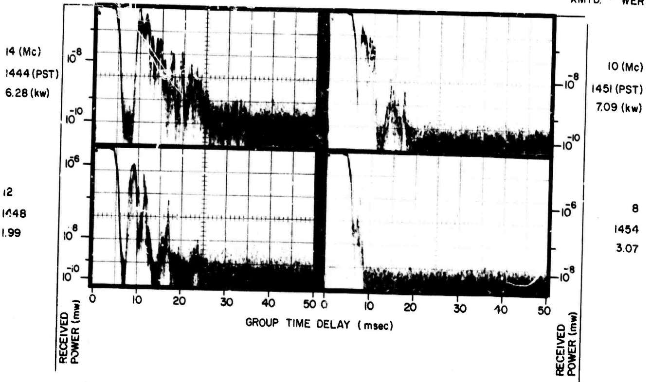
A RECORDS, 23 FEB 1965, 122° BEARING
