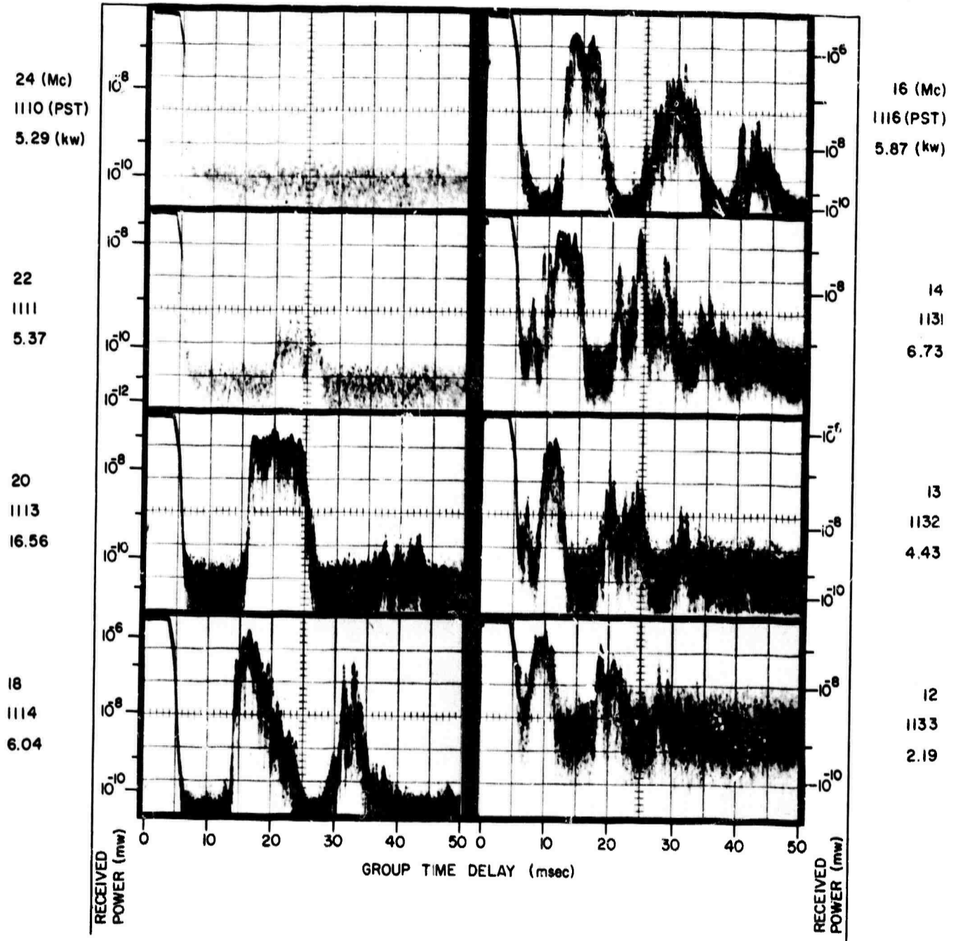
A RECORDS, 9 MAR 1965, 302° BEARING
