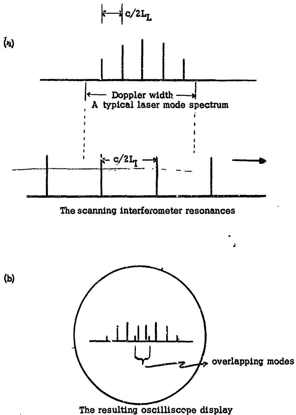
Fig. 18 a. A diagram showing the scanning interferometer resonances separated by c/2L_I , less than the Doppler broadened gain curve. b. The resulting oscilloscope display with overlapping mode spectra.
