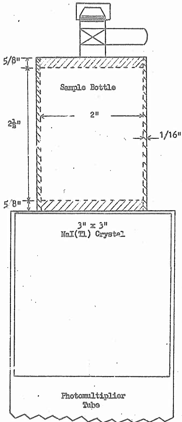
Diagram of Scintillation Detector and Sample Bottle
