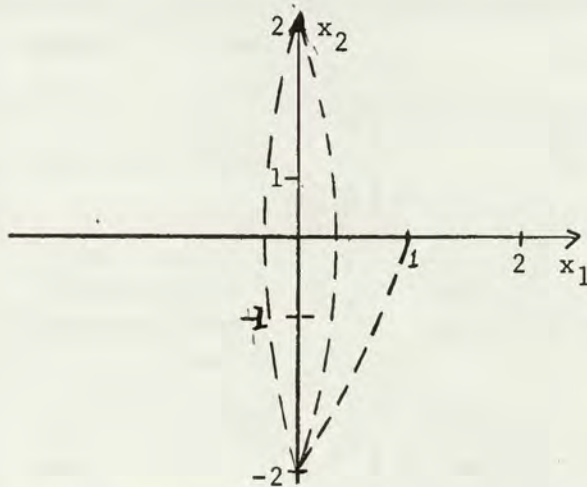
Figure II-1: Phase Plane For Example Problem
