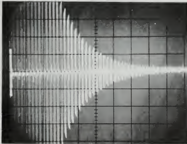
Figure 2-5 A receiver's output display at 100 MHz
