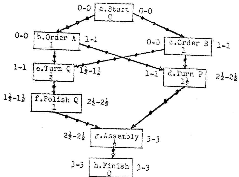
FIGURE 5 THEORETICAL MINIMUM-TIME NETWORK DIAGRAM FOR SAMPLE PROJECT
