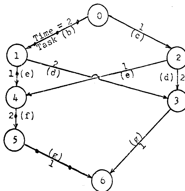
FIGURE 6 NETWORK DIAGRAM IN NODAL FORM
