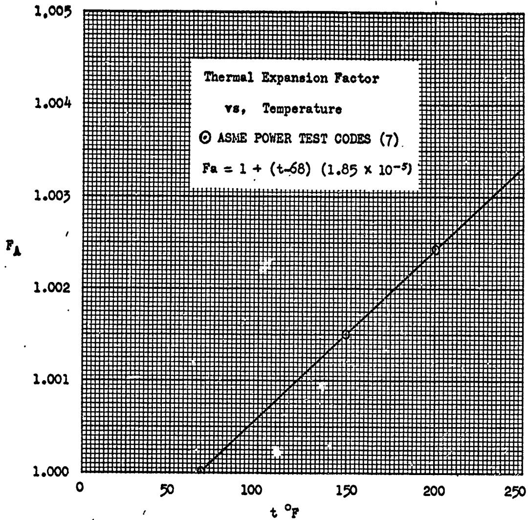
Figure 8. Thermal expansion factor vs. temperature.
