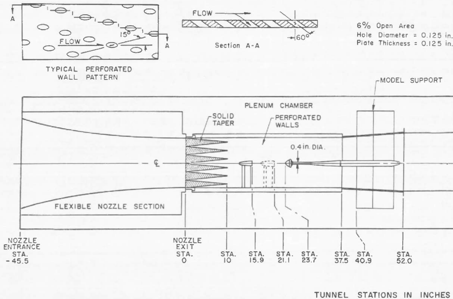
Fig. 1 Schematic of Tunnel 1T with a Typical Decelerator-Payload Installation
