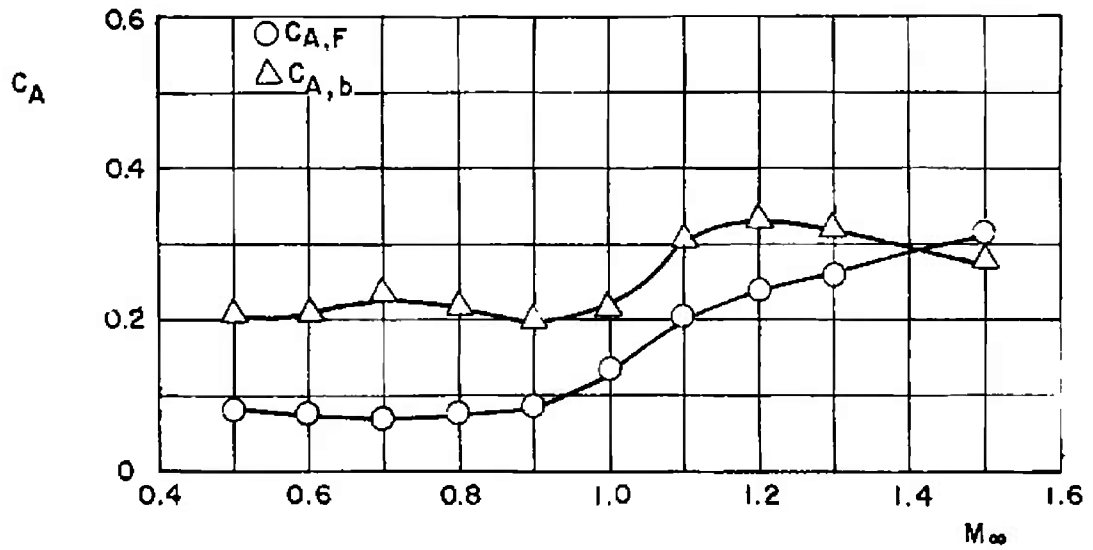
Fig. 11 Effect of Mach Number Variation on the C_{A,F} and C_{A,b} for the Static Stability Model, \alpha = 0^\circ
