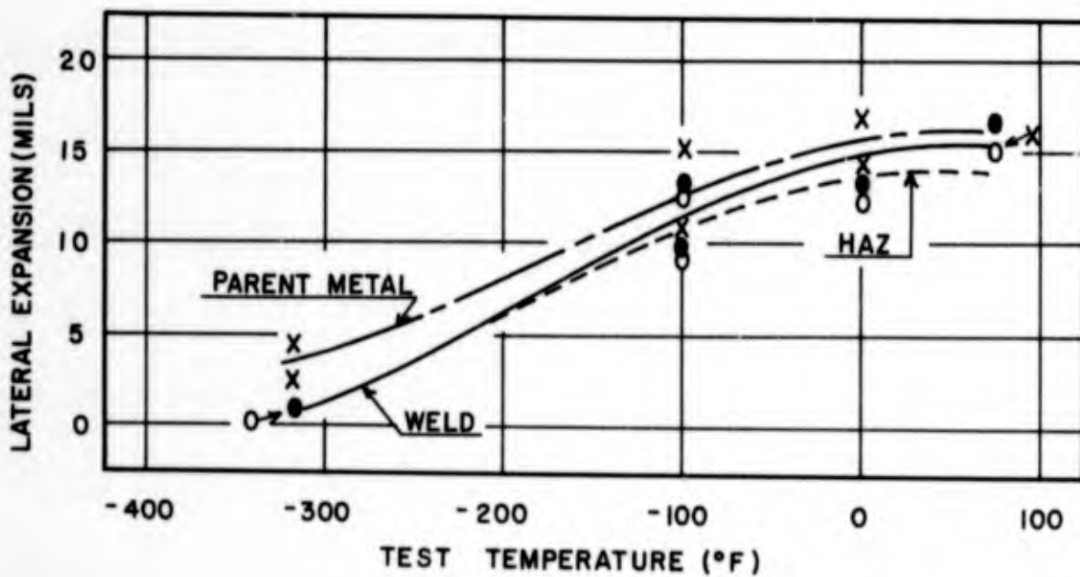
Figure 61. Charpy V-Notch Impact Properties of TIG Weld No. M303 Made in HP 9-l-25 1-Inch Plate at 10 ipm in Helium Using Filler Wire No. 19.
