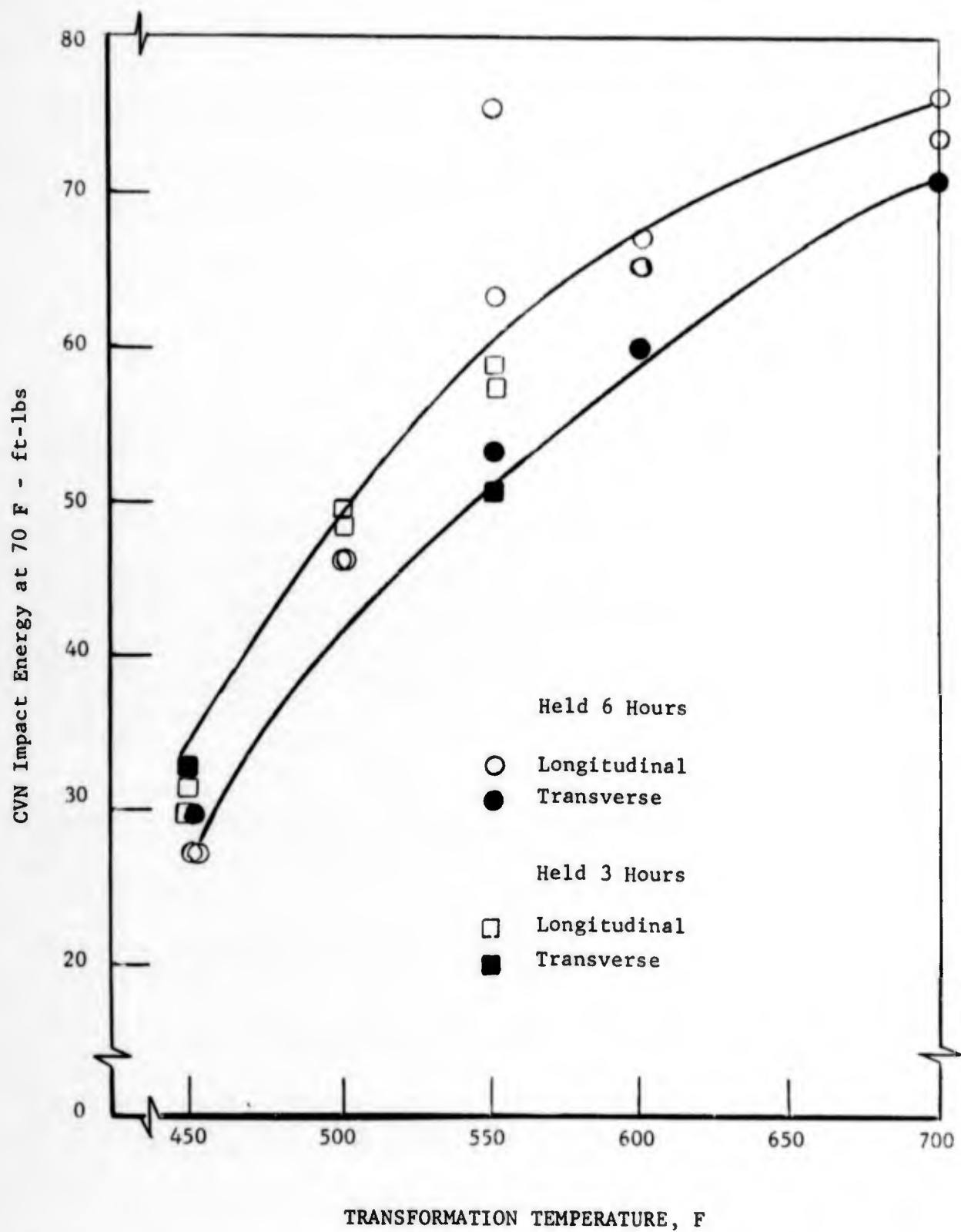
Figure 5. Impact Resistance as a Function of Bainitic Transformation Temperature of HP 9-4-43 Steel. (Heat 3950831) (Ref. 5)
