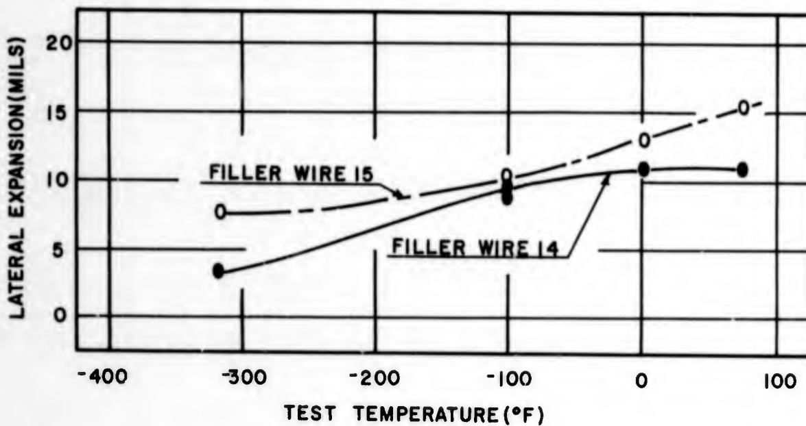
Figure 37. Charpy V-Notch Impact Properties of Martensitic HP 9-4-20 TIG Weld Metal.
