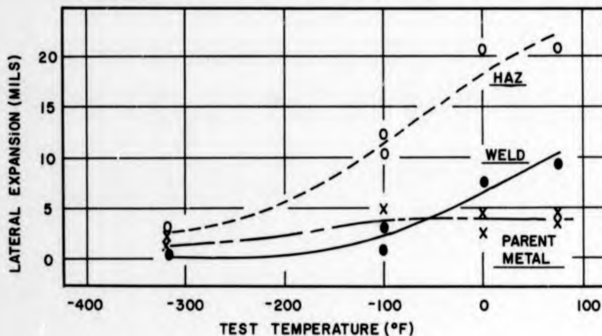
Figure 127. Charpy V-Notch Impact Properties of Laititic HP 9-4-45 Weld Metal and Heat Affected Zones for TIG Weld No. 0306.
