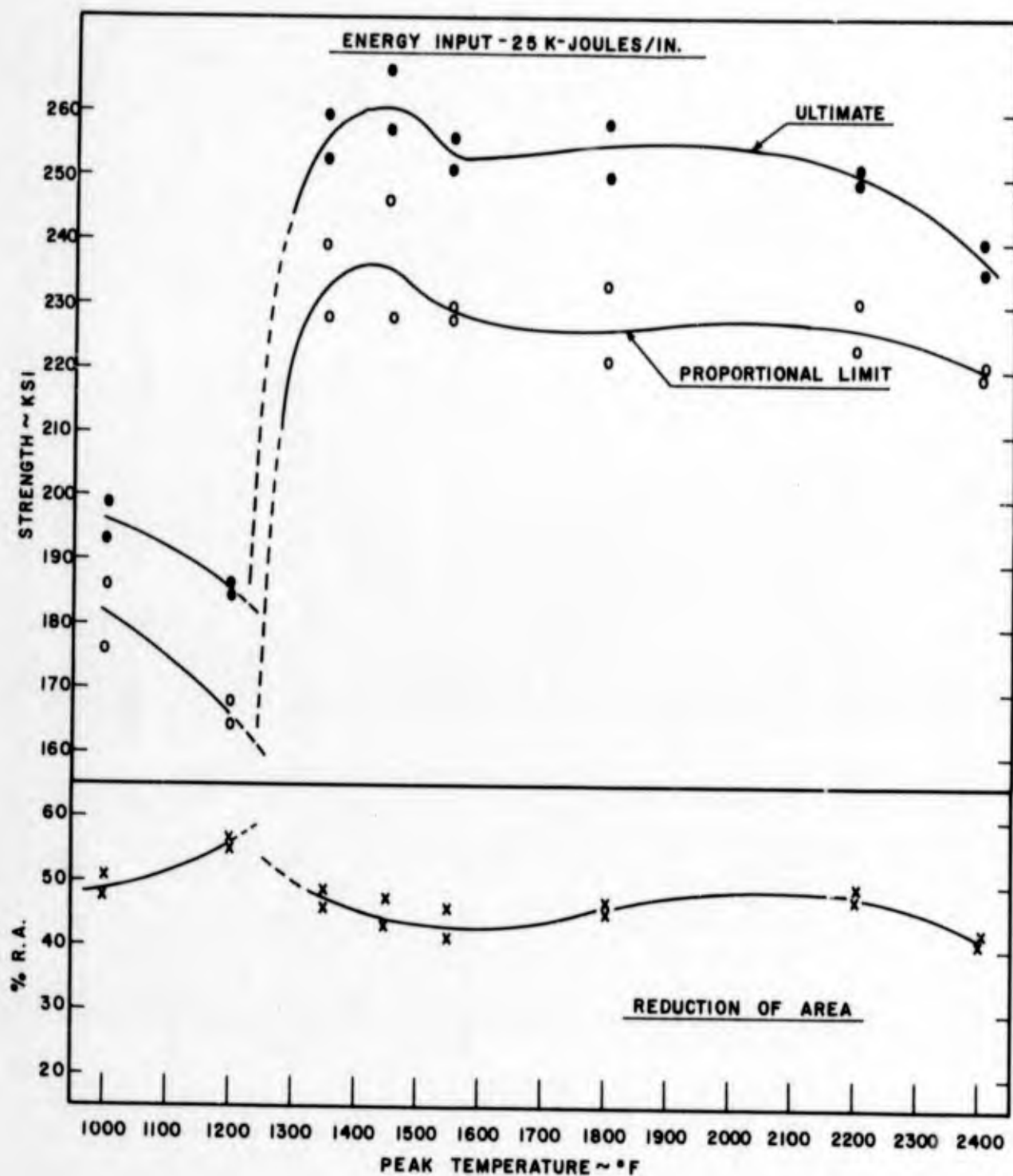
Figure 146. Influence of Peak Temperature of Synthetic Weld Thermal Cycle on the Tensile Properties of HP 9-4-45 Bainitic Steel - 25 K Joules/in Energy Input.
