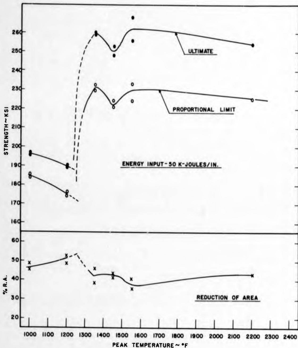
Figure 147. Influence of Peak Temperature of Synthetic Weld Thermal Cycle on the Tensile Properties of HP 9-4-45 Bainitic Steel. 50 K Joules/in. Energy Input.
