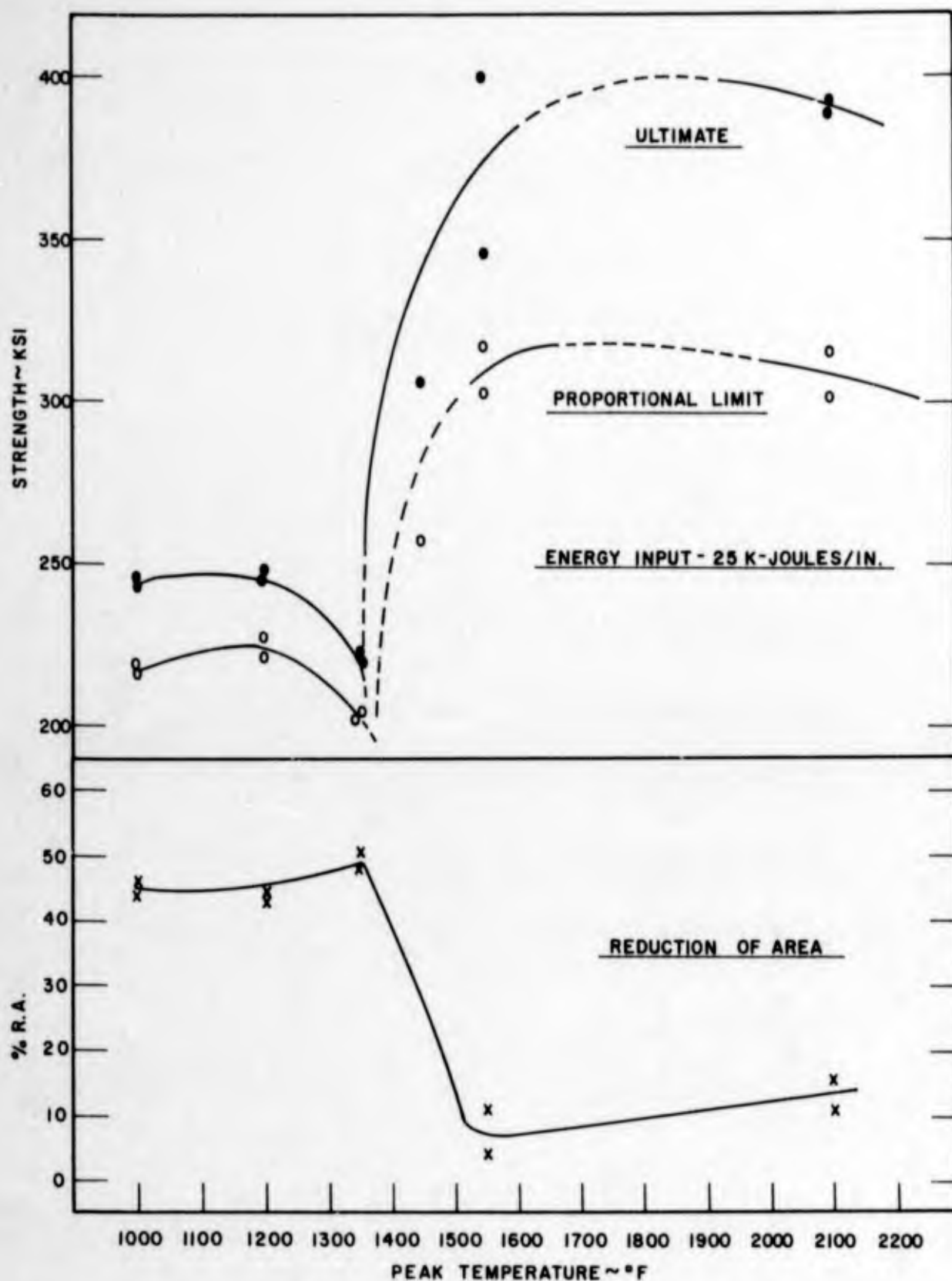
Figure 144. Influence of Peak Temperature of Synthetic Weld Thermal Cycle on the Tensile Properties of D6AC Martensitic Steel. 25 K Joules/in. Energy Input.
