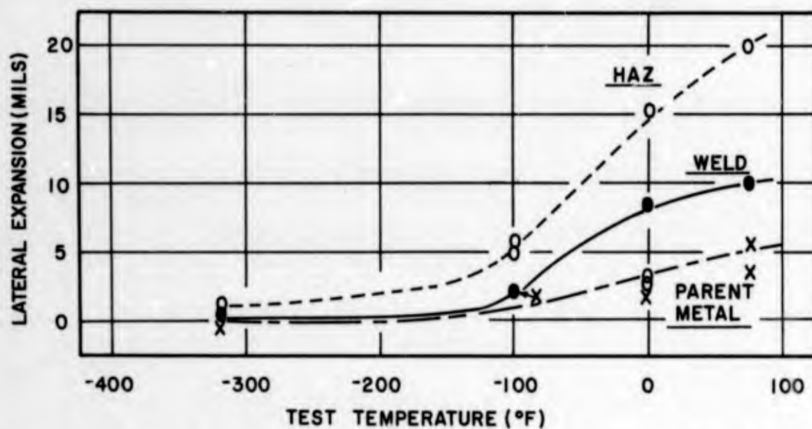
Figure 99. Charpy V-Notch Impact Properties of Martensitic D6AC Weld Metal and Heat Affected Zones for TIG Weld No. S304.
