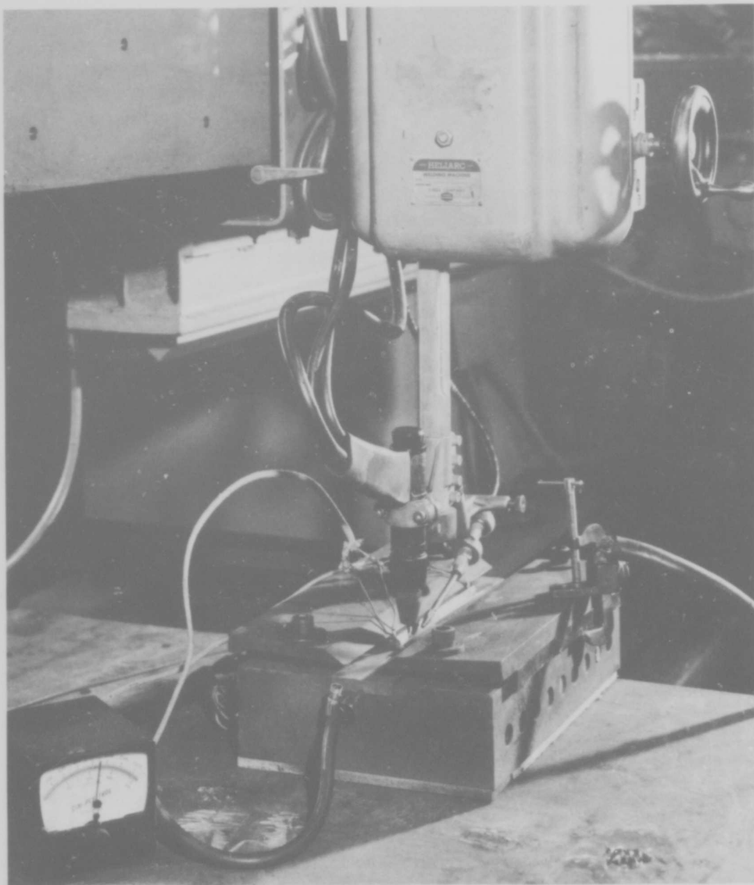
Figure 8 Welding Fixture and Heliarc Torch
