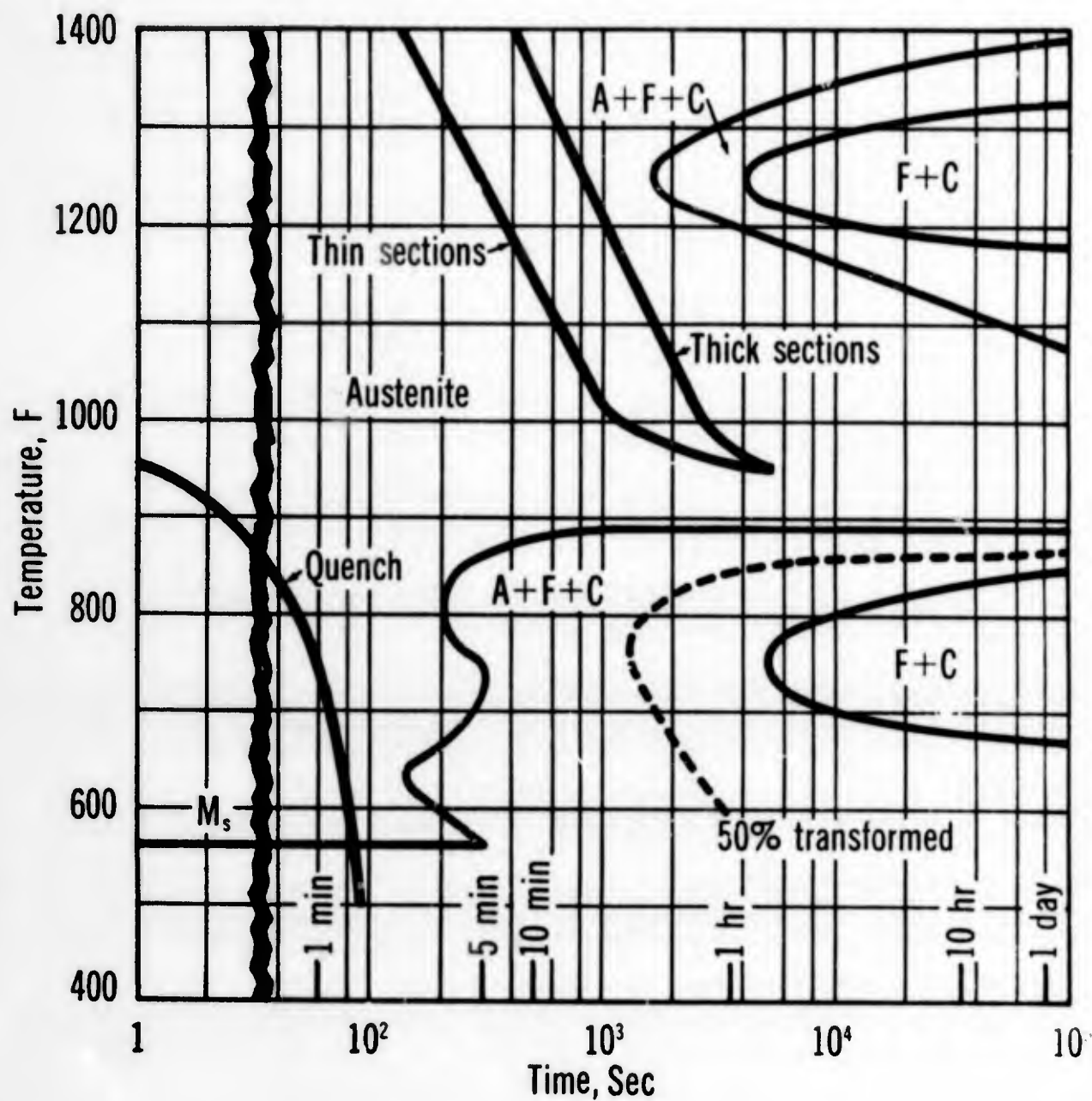
Figure 137. Isothermal Transformation Diagram for D6AC Steel. (Ref. 16).
