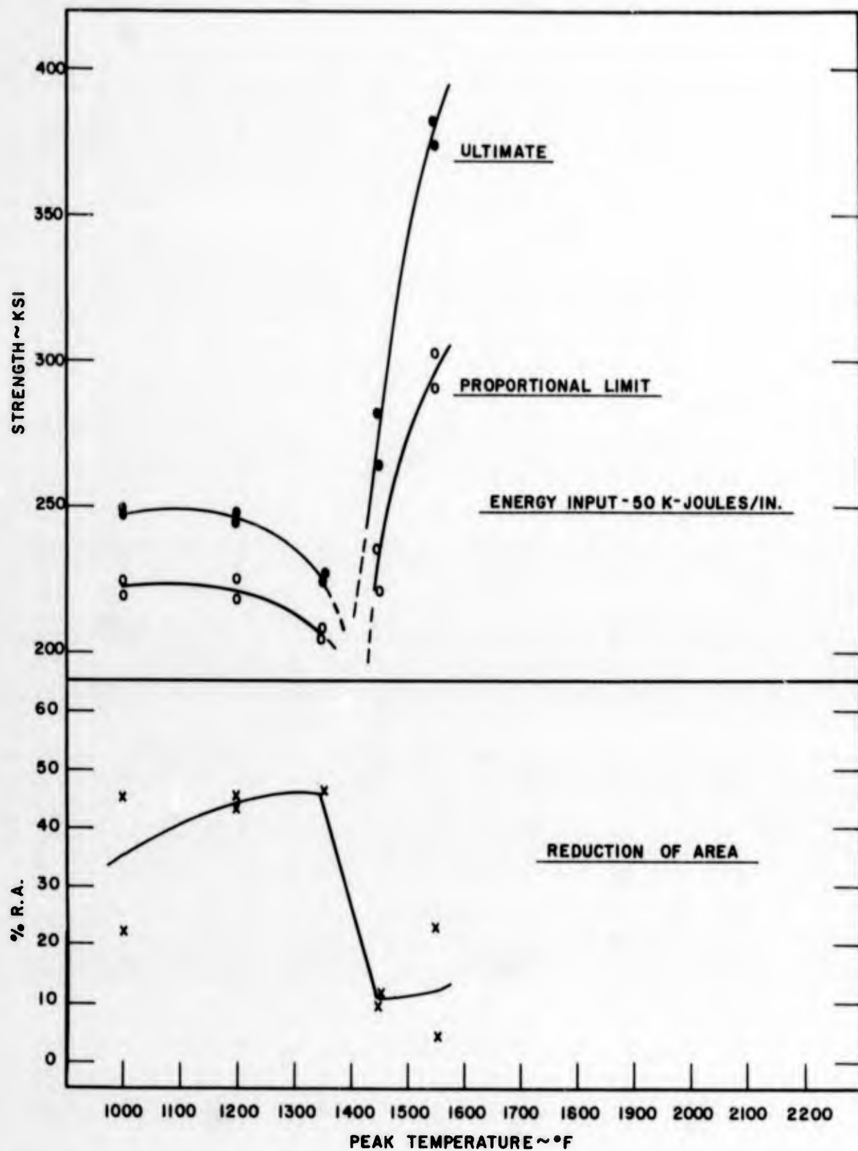
Figure 145. Influence of Peak Temperature of Synthetic Weld Thermal Cycle on the Tensile Properties of D6AC Martensitic Steel. 50 K Joules/in. Energy Input.
