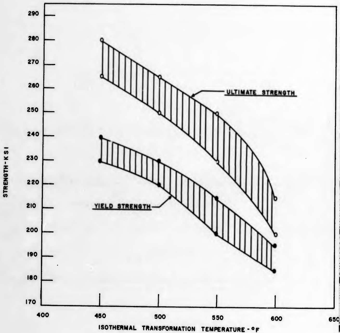
Figure 103. The Effect of Transformation Temperature on the Ultimate and Yield Strengths of HP 9-4-45 Steel.
