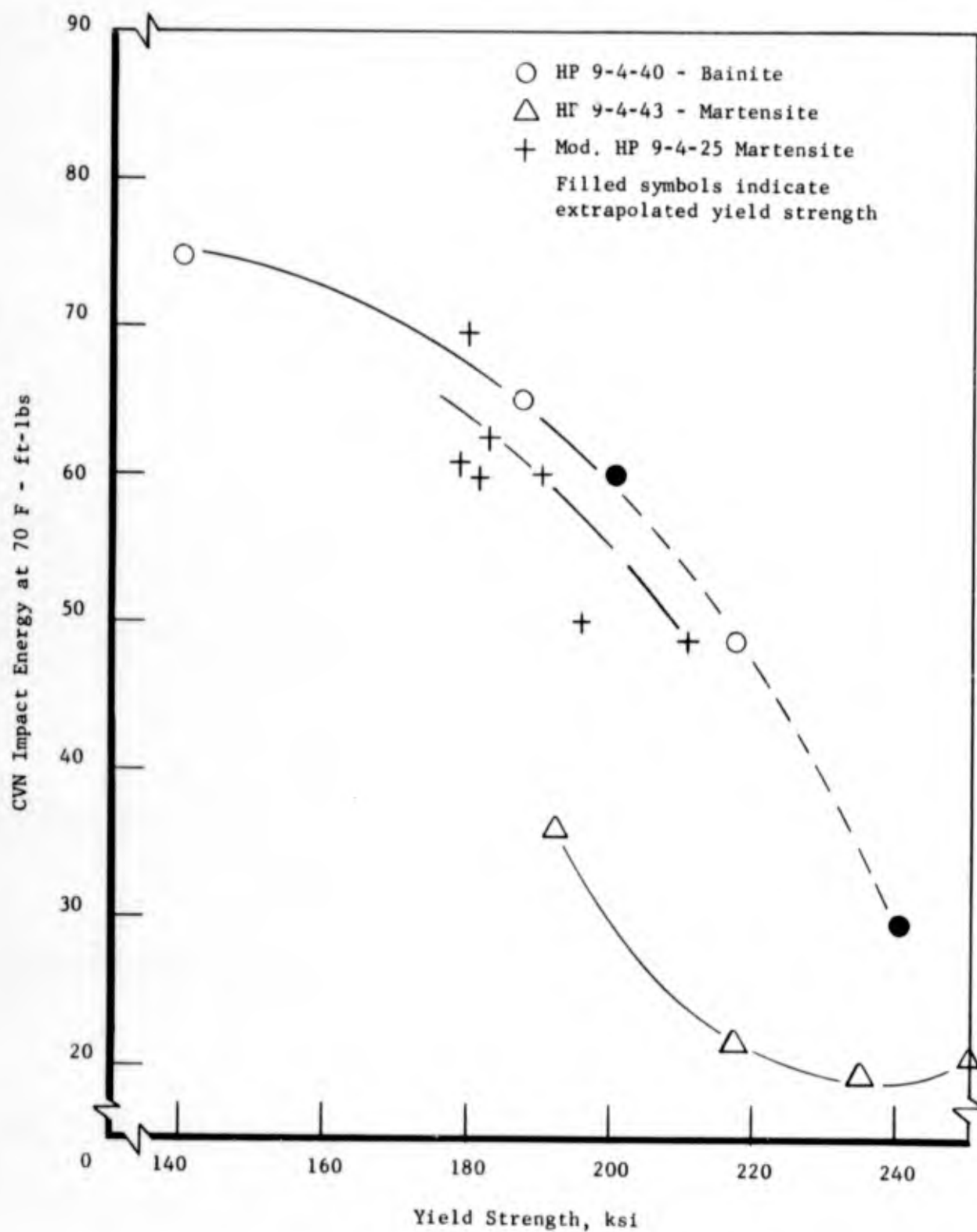
Figure 3. Impact Resistance of Tempered Martensitic and Bainitic Structures as Related to Yield Strength in HP 9-4-X Alloy Steels. (Ref. 5)
