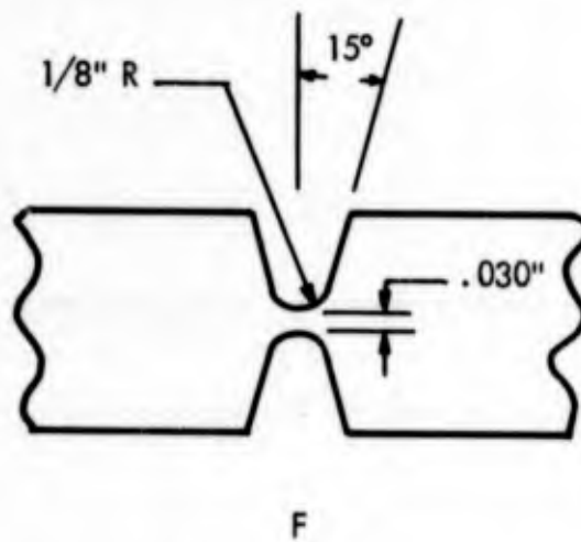
Figure 7. Weld Joint Designs for 1 Inch Plate.
