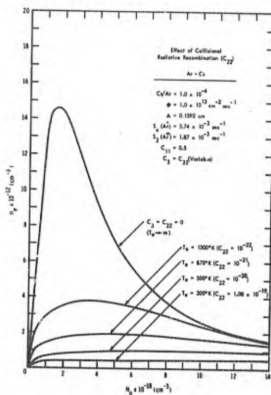
Fig. 5. Effect of collisional-radiative recombination ( C_3, C_{22} ) on electron number density.
