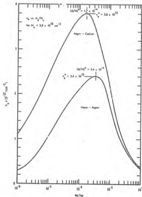
Fig. 3. Electron number density ( n_e ) as a function of the ratio of the gas constituents ( A_0/N_0^e ) for N_0 = 3.0 \times 10^{18} \text{ cm}^{-3} .
