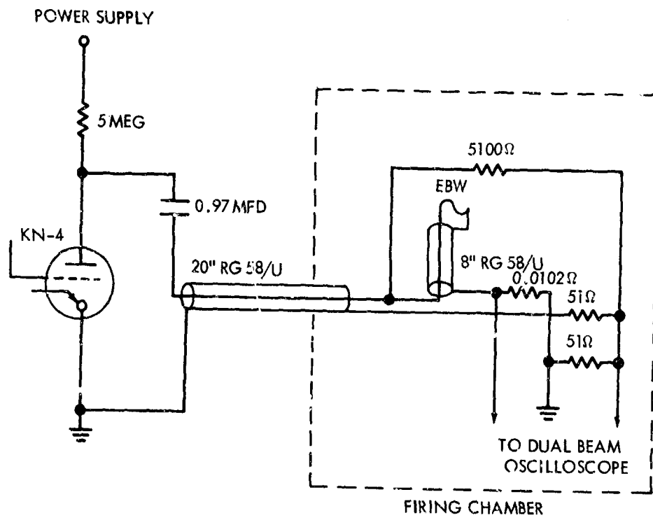
FIG. 1 TEST CIRCUIT
