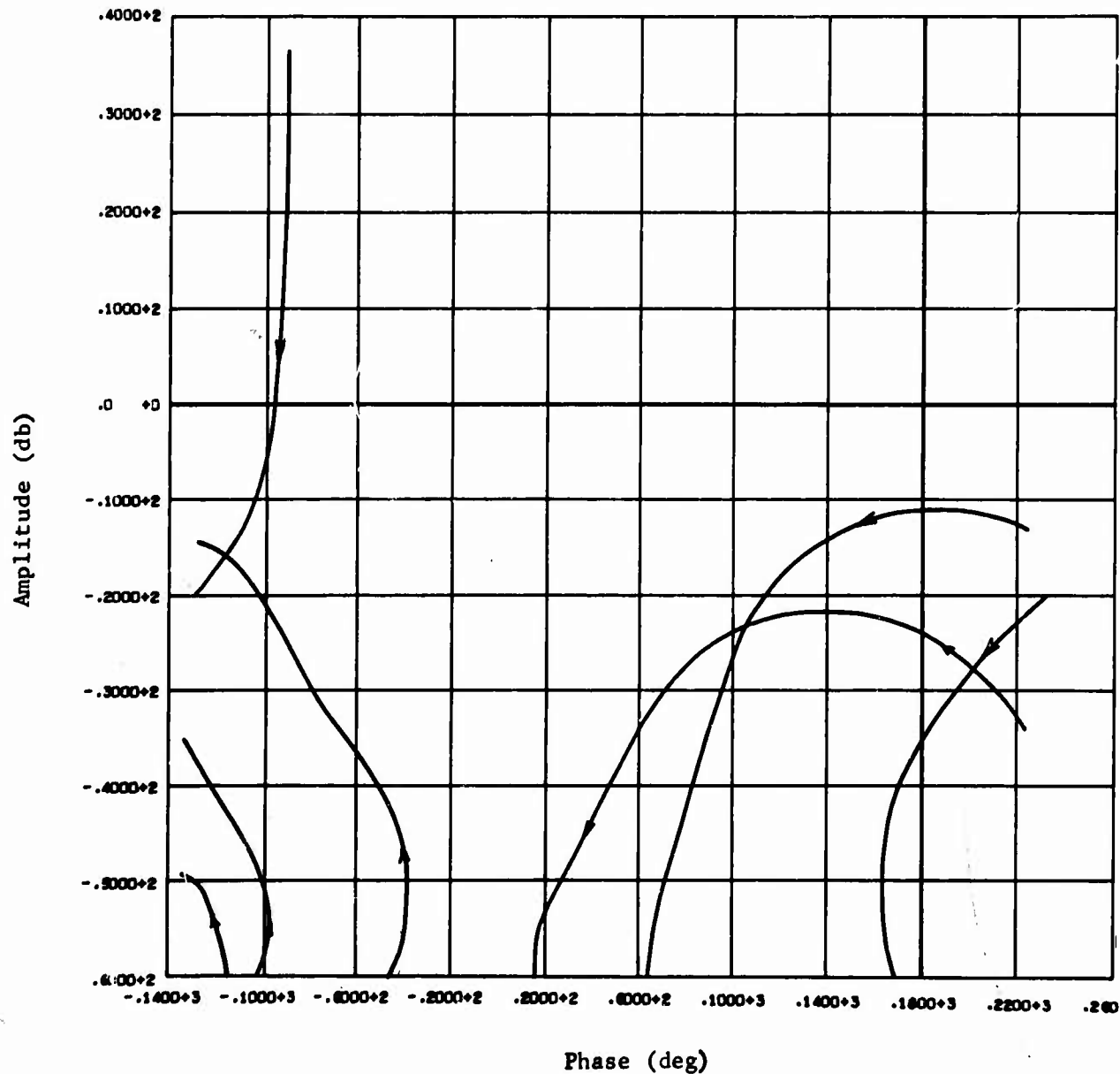
Fig. C-46 Open Loop Frequency Response, Pitch and Yaw Axis, Stage II Midflight (AGC)
