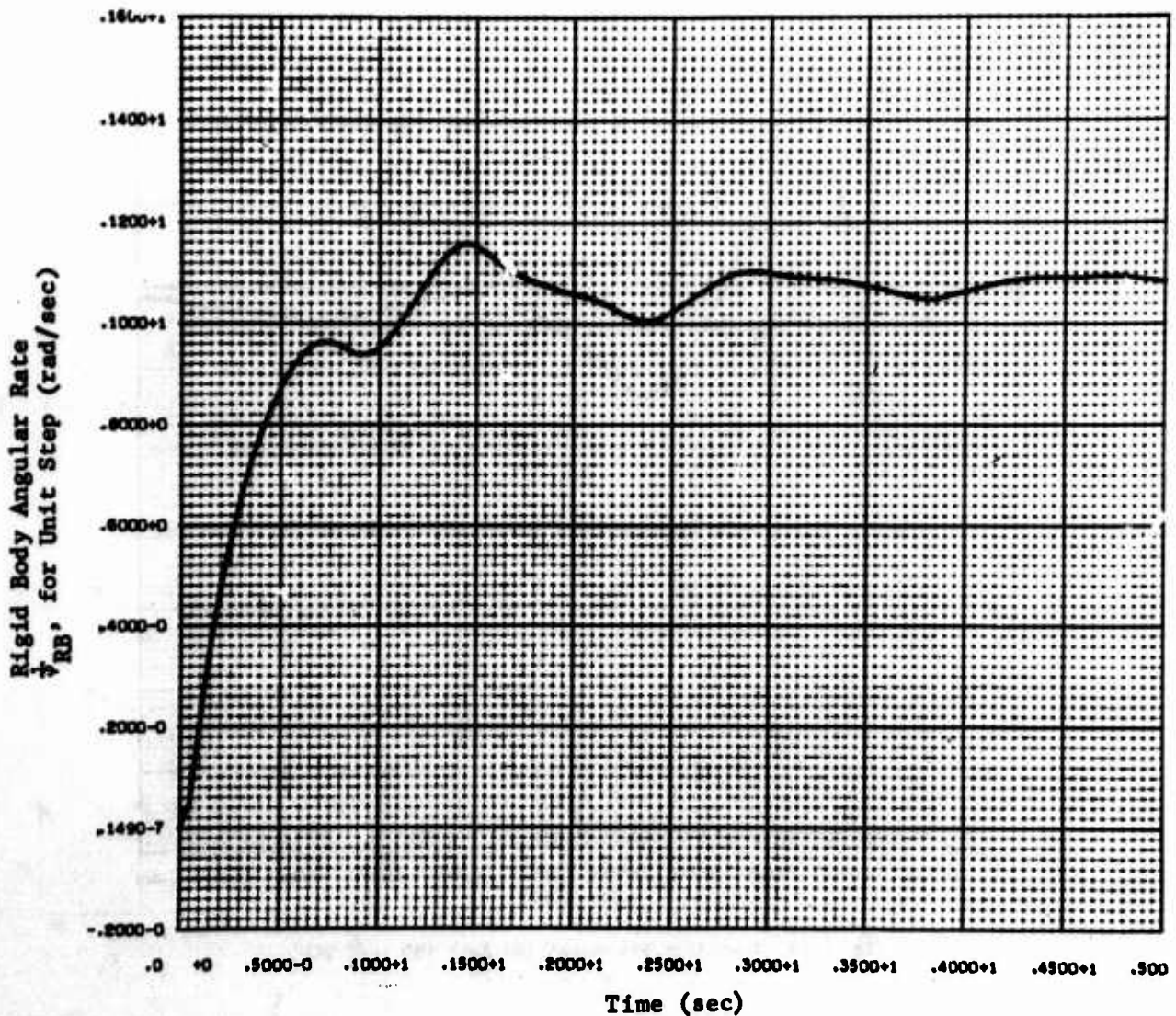
Fig. C-27 Transient Response, Yaw Axis (80 sec, AGC)
