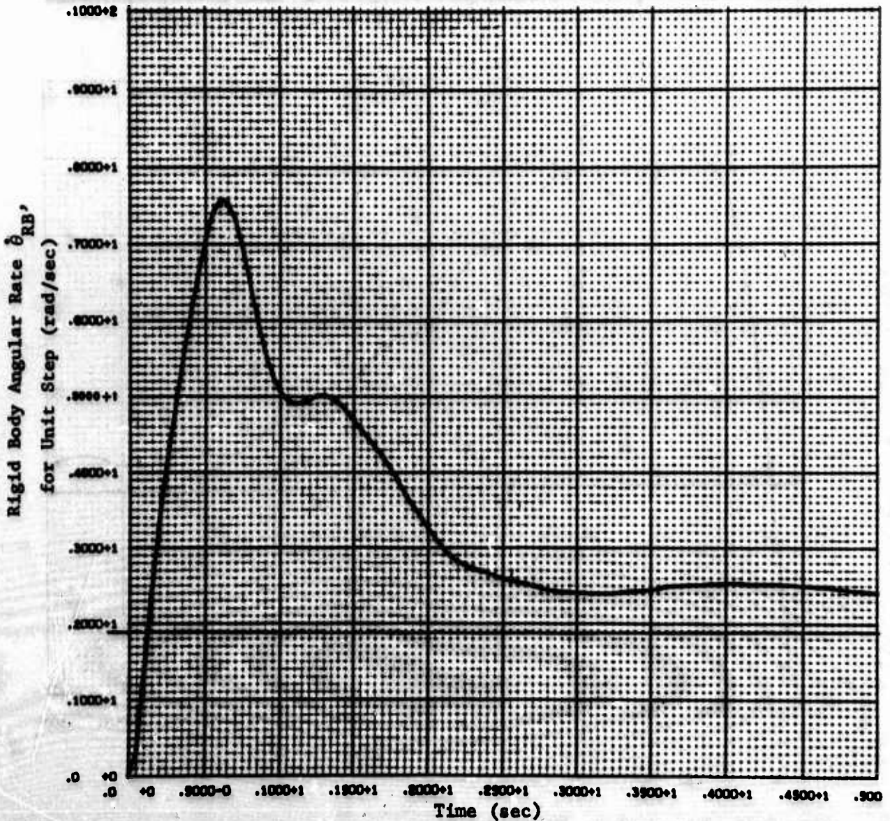
Fig. C-38 Transient Response, Pitch Axis, with Load Relief (80 sec, BGC)
