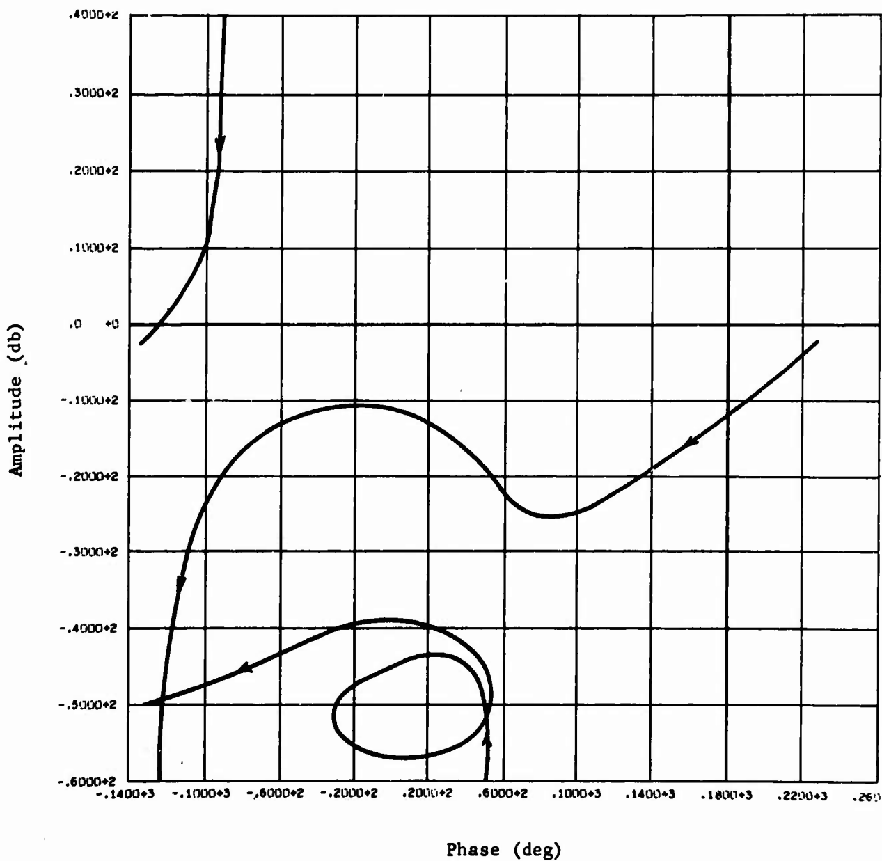
Fig. C-44 Open Loop Frequency Response, Roll Axis, Stage I
