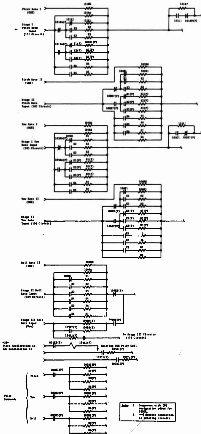
Fig. E-4 Broader FIDOL Adapter-Programmed Changes
