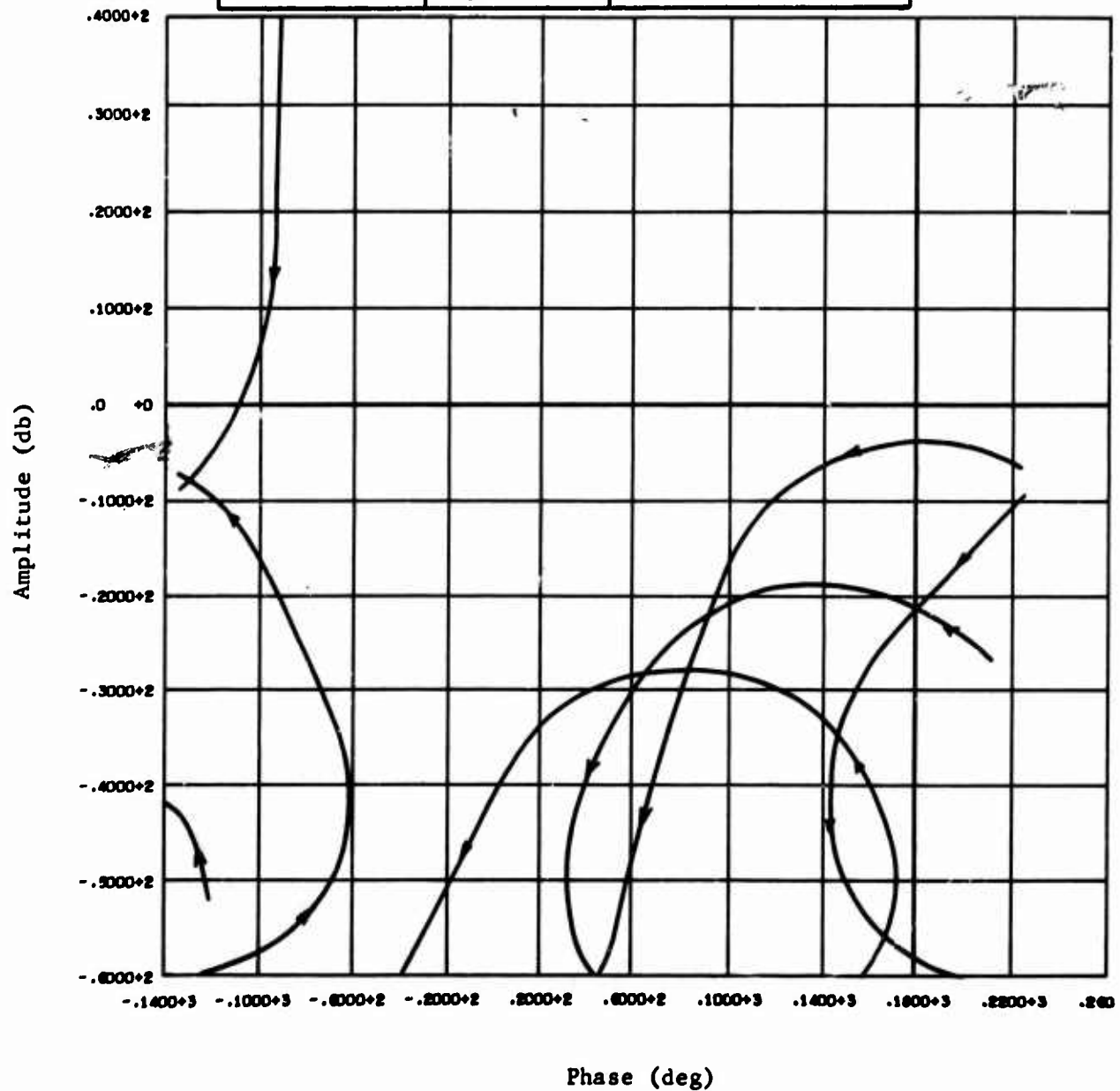
Fig. C-47 Open Loop Frequency Response, Pitch and Yaw Axes, Stage II Burnout
