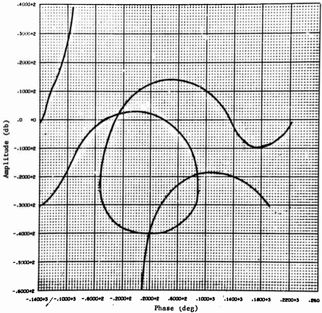
Fig. C-52 Open Loop Frequency Response, Roll Axis (60 sec)
