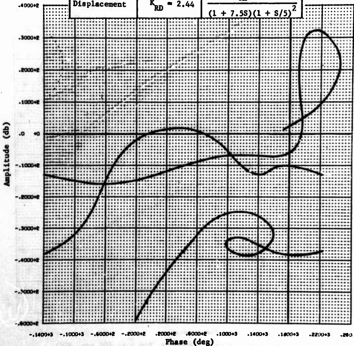
Fig. C-21 Open Loop Frequency Response, Yaw Axis (105 sec)
