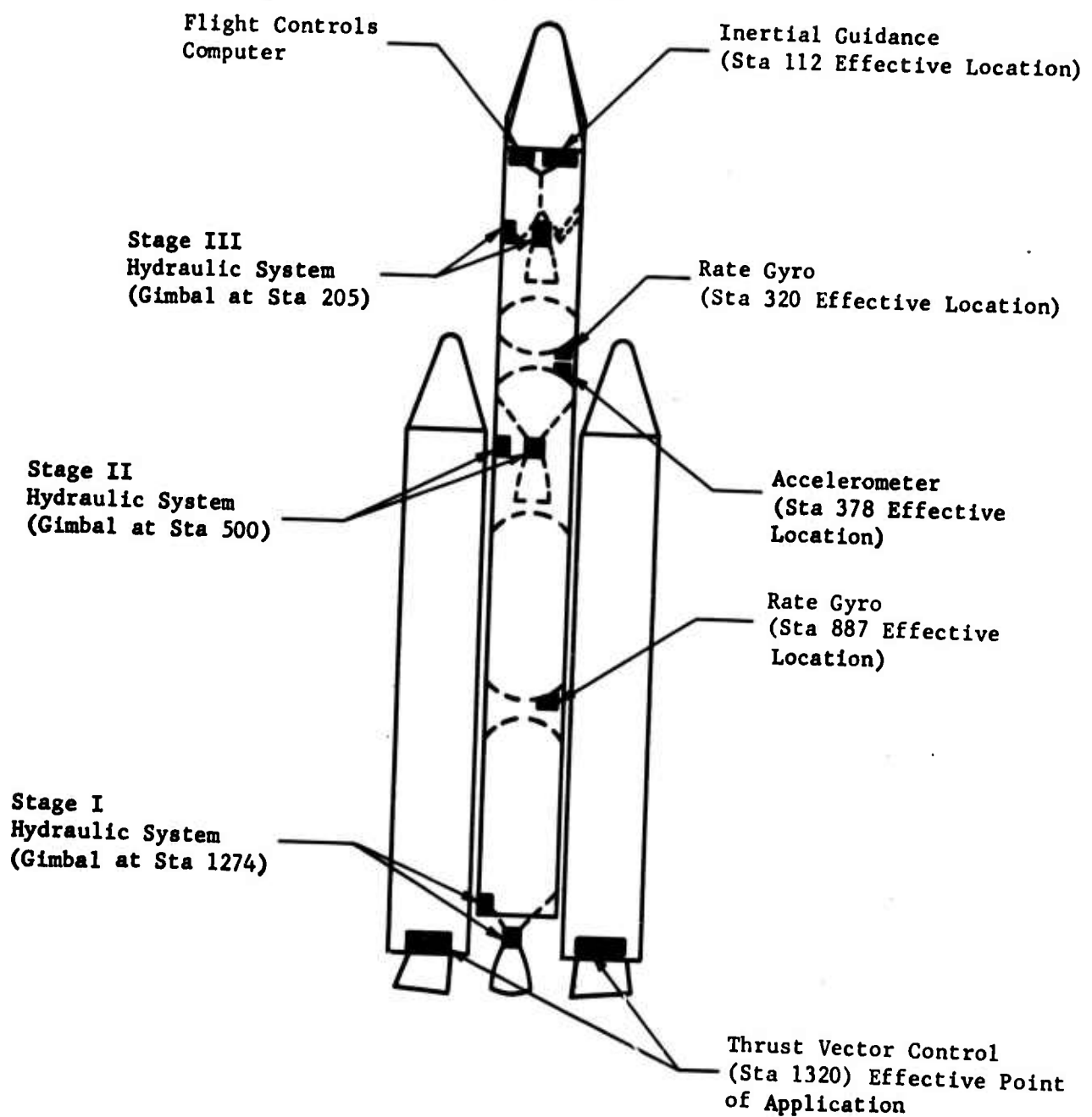
Fig. I-1 Flight Control System
