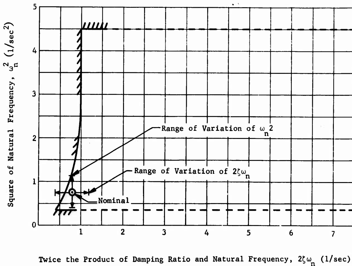
Fig. 22 Broader System Handling Characteristic Variation Due To Tolerances (Stage 0, Pitch Axis, 60 sec)
