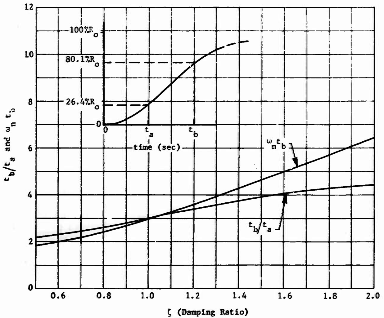
Fig. B-4 Responses with Overshoot Ratios Less than 0.05
