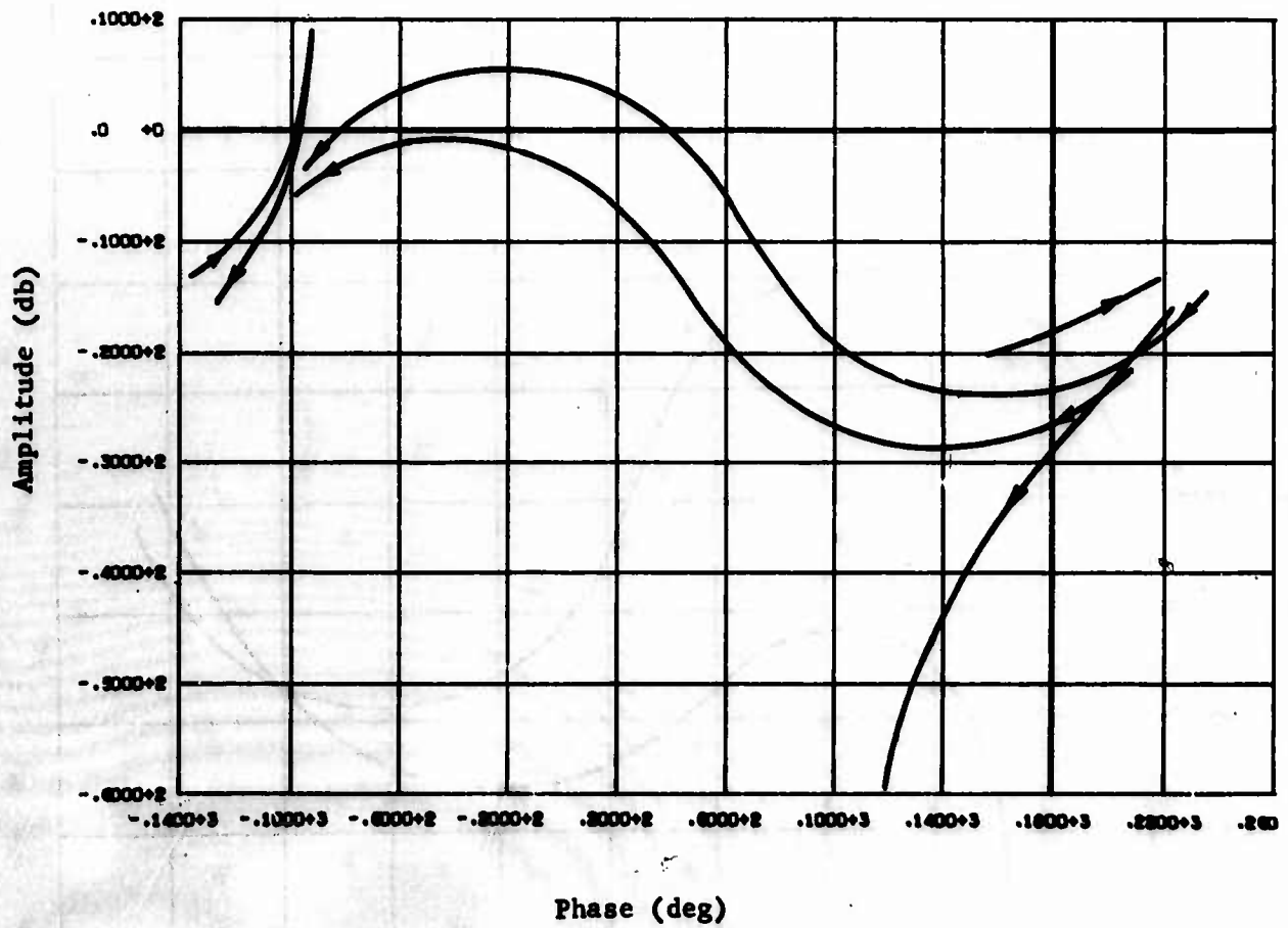
Fig. C-40 Open Loop Frequency Response, Pitch and Yaw Axis, Stage I Start
