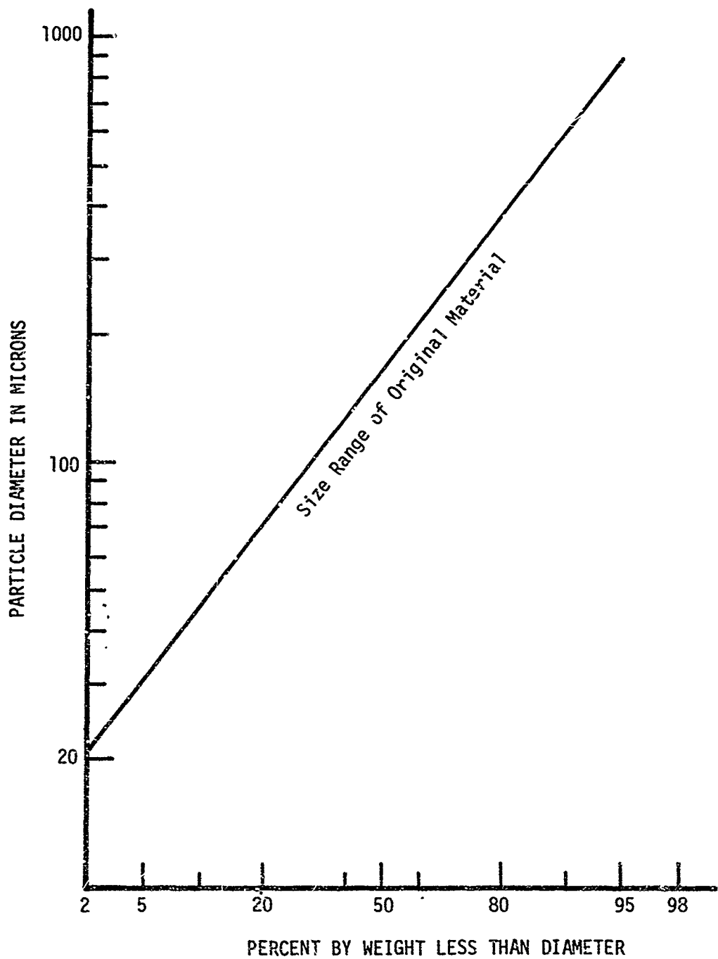
Figure 8. Size Distribution of Mill Scale Particles.
