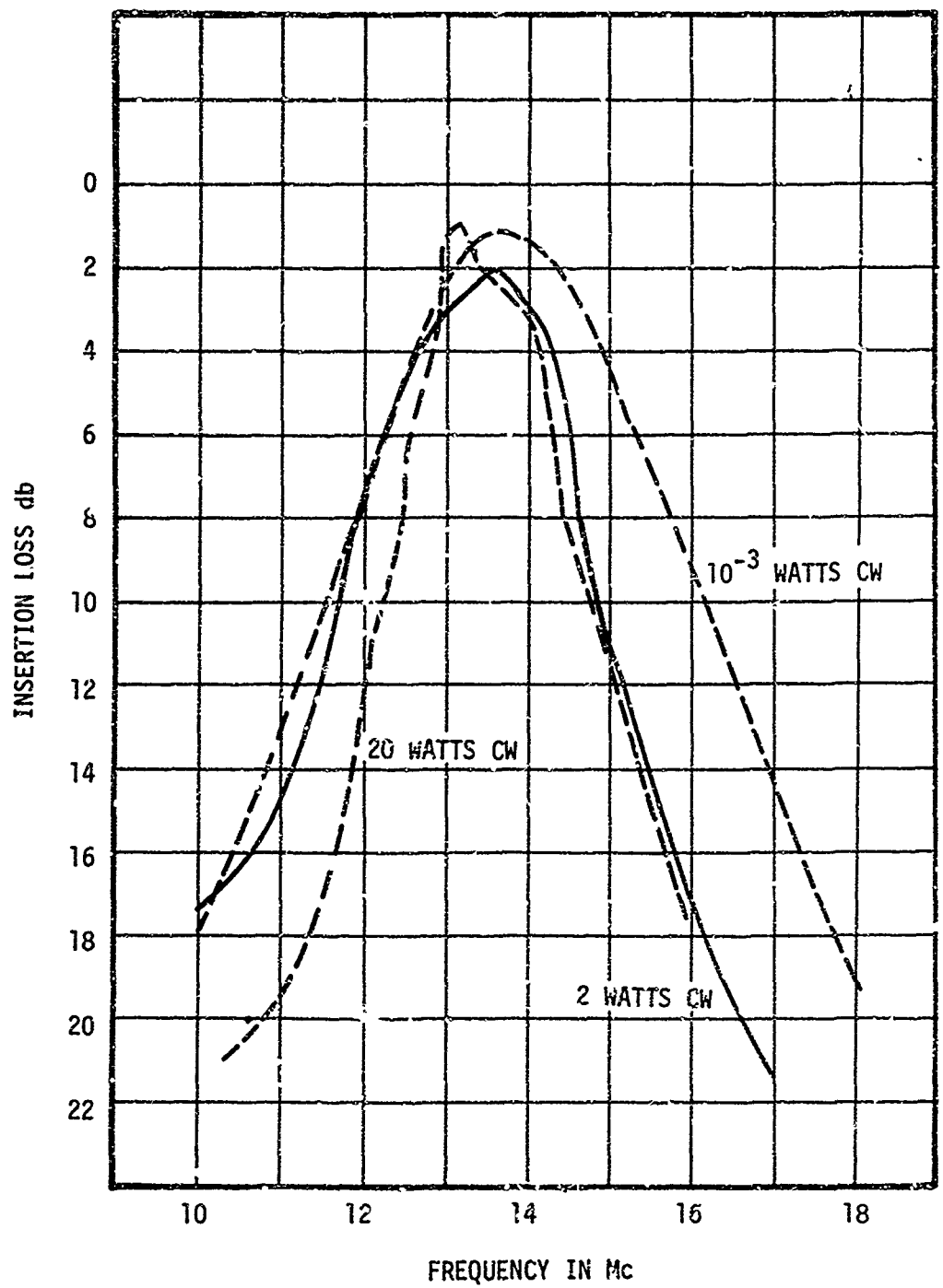
Figure 45. Effect of CW Power Level on Ferrite Filter.
