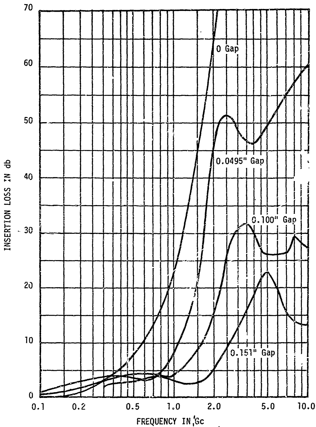
Figure 34. Measured Effect of Gap on Loss.
