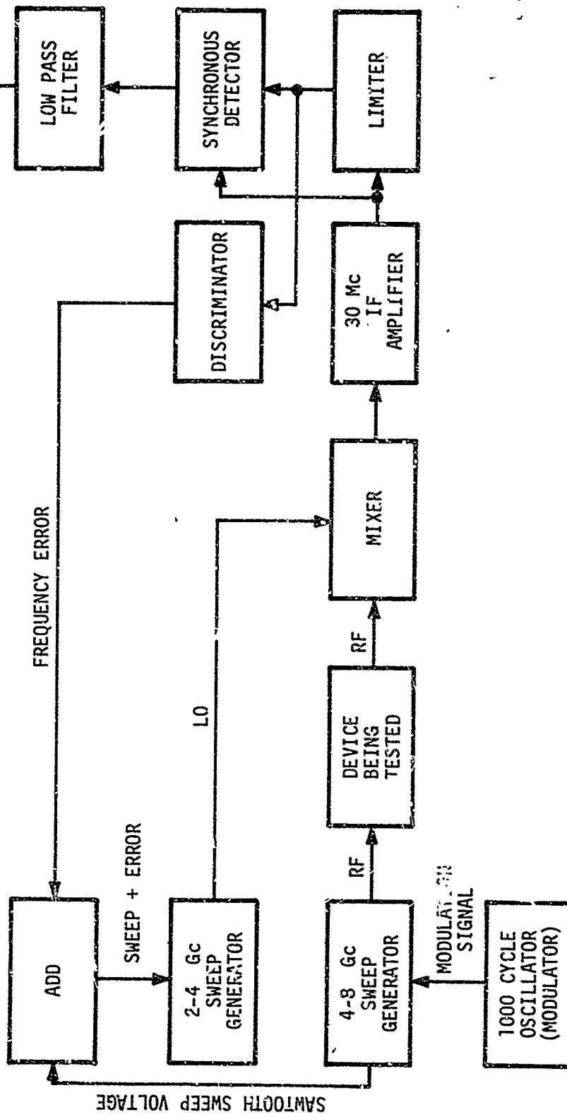
Figure 53. Superheterodyne Measurement System.
