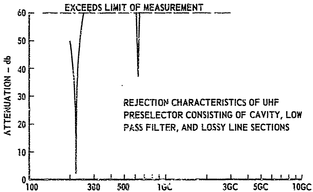
Figure 27. Preselector Loss Characteristics.
