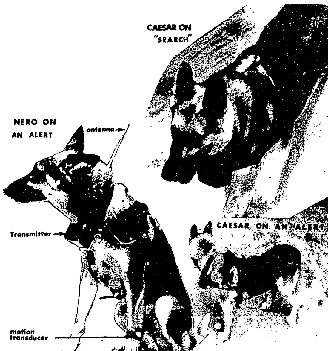
FIG. 2 POSITION AND USE OF THE SPECIAL EQUIPMENT
