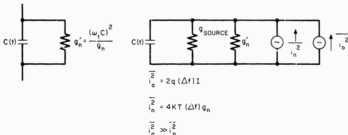
Fig. C-2. Noise model of input circuit.
