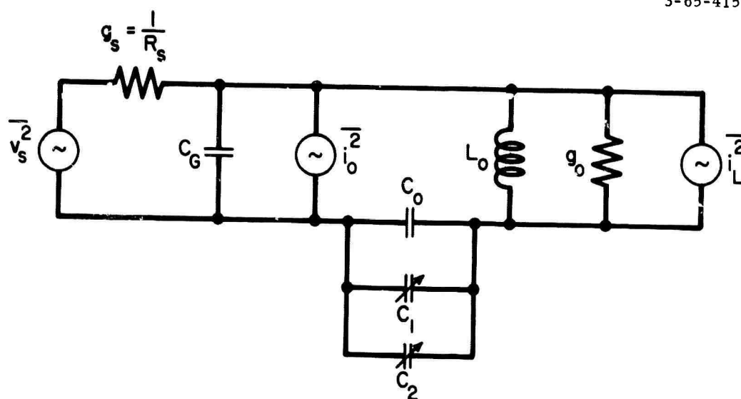
Fig. 14. Noise circuit of low frequency reactance converter.
