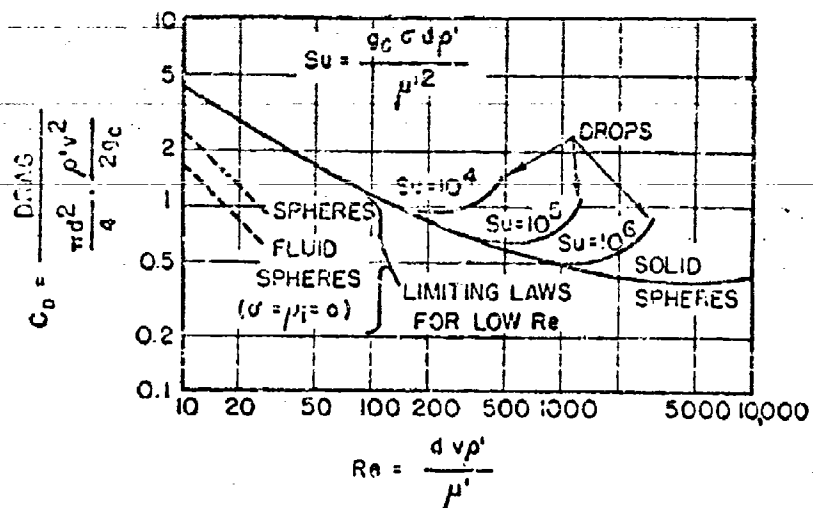
FIGURE 5. DRAG COEFFICIENTS OF SPHERES AND DROPS (Hughes and Gilliland) 7
