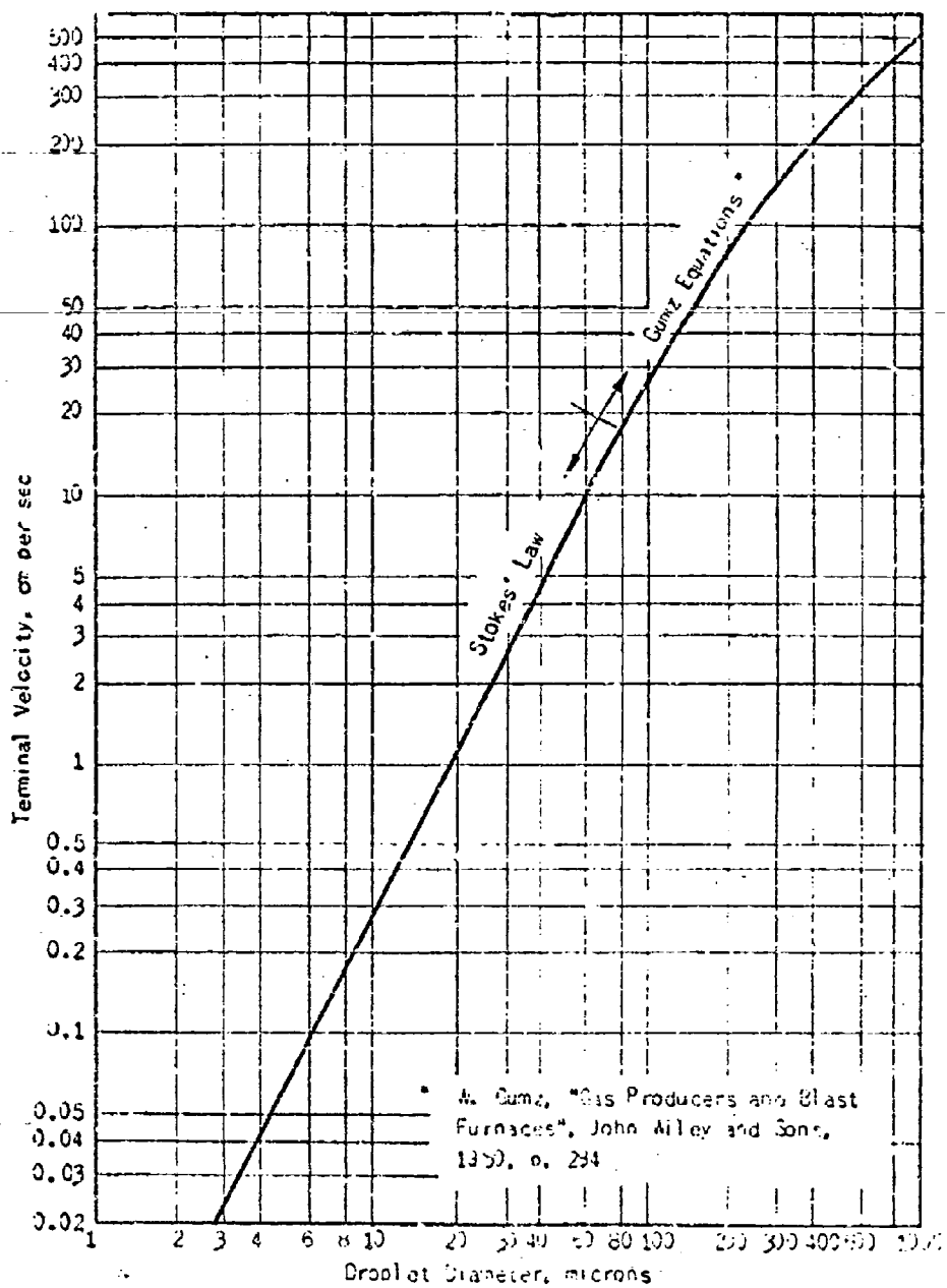
FIGURE 4. TERMINAL VELOCITY OF WATER DROPLETS IN AIR AT 70 F
