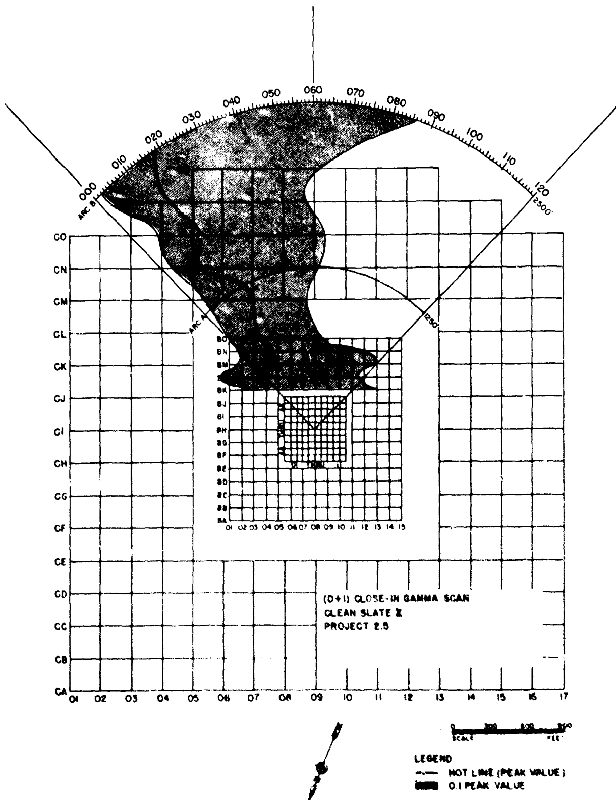
Figure 6.7 Close-in gamma survey, CS II.
