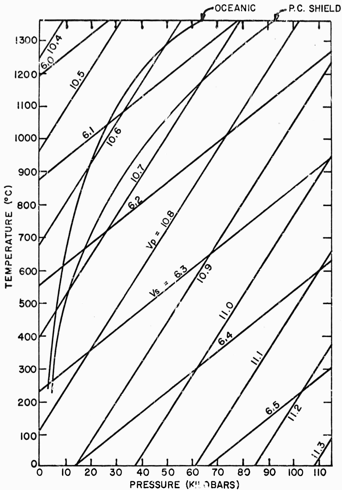
FIG 2B: T-P PLOT AT CONSTANT SOUND VELOCITY FOR \text{Al}_2\text{O}_3 WITH GEOTHERMIC GRADIENTS SUPERPOSED
