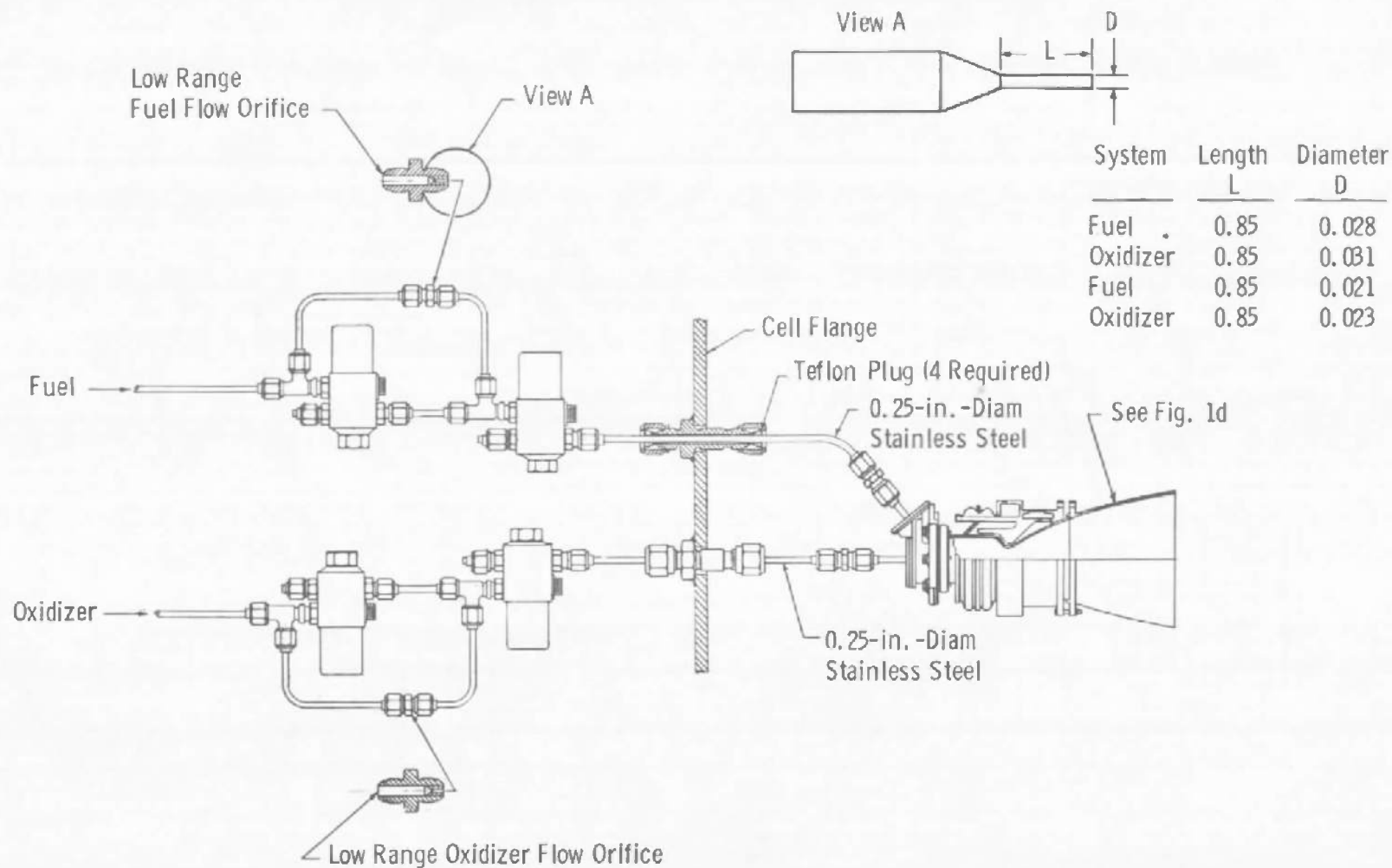
Fig. 2 Model Rocket Engine Propellant System for Configuration D Engine Throttling
