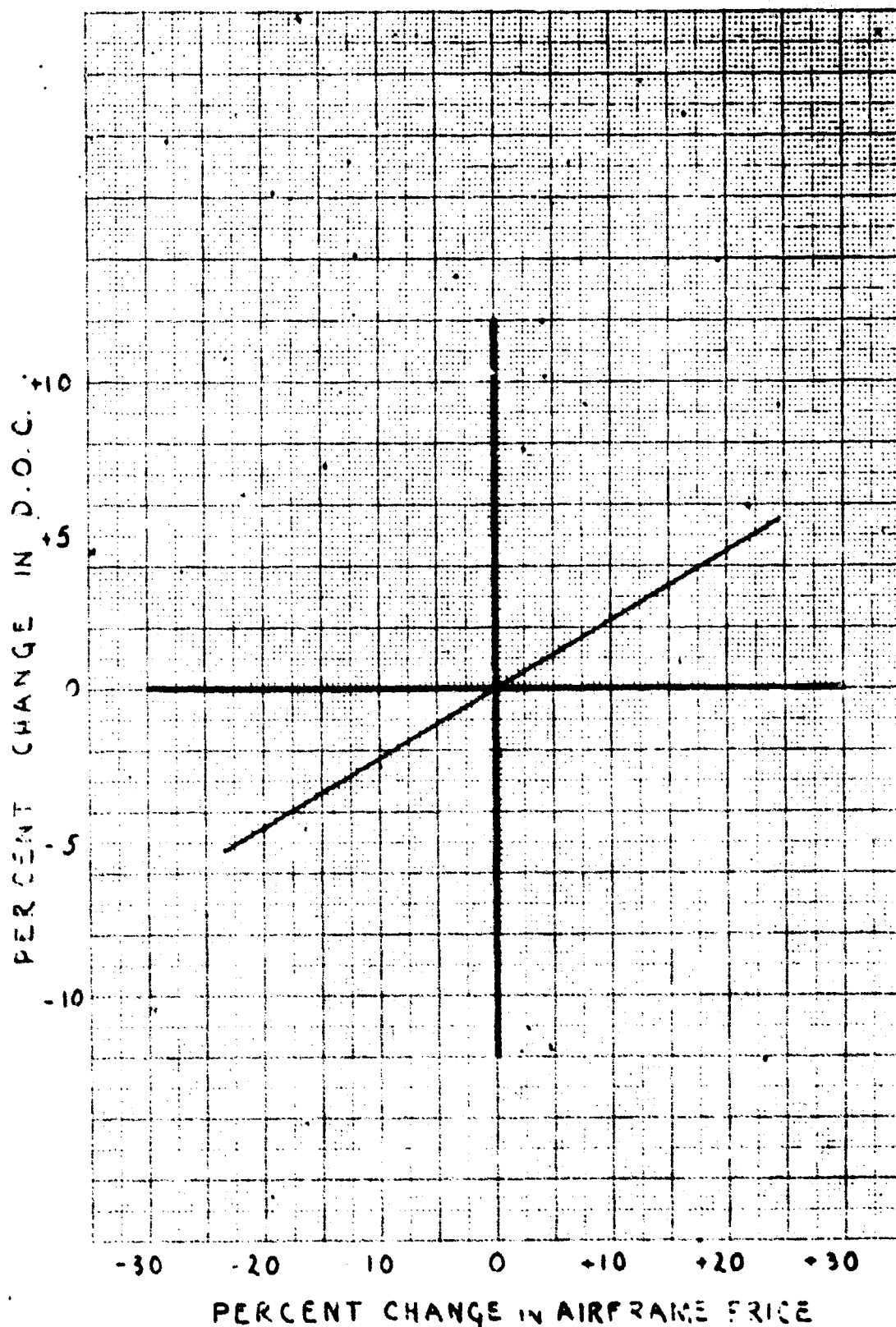
Fig. 5-5 Airframe Price Vs DOC (SCAT 15P)
