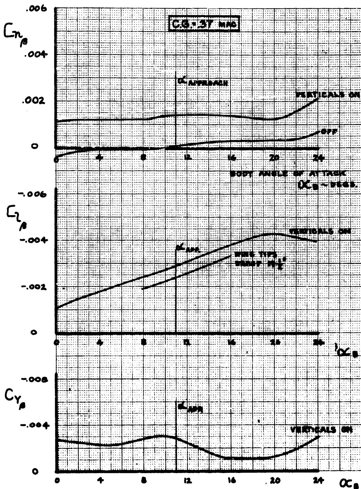
Fig. 3-37 Estimated Lateral-Directional Static Derivatives at Approach
