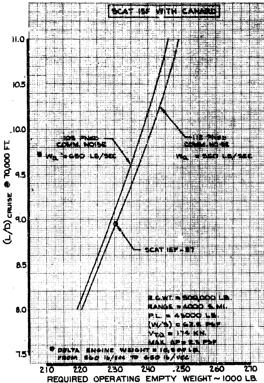
Fig. 3-21 (L/D) - OEW Trade
