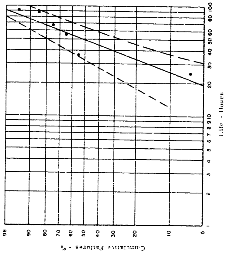
Figure 14 Weibull Plot of 2600°F Cyclic Oxidation Test Results; IRW Cr-Ti-Si Coating on 20 Mil C129Y
