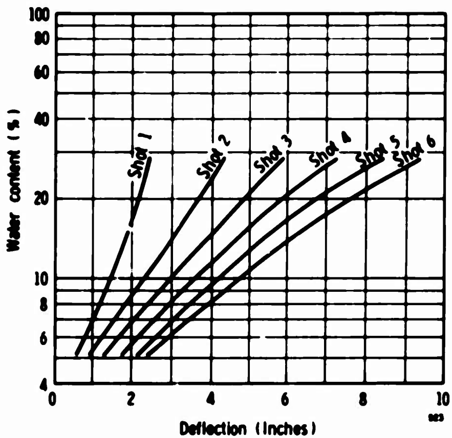
Figure 13. Moisture Content Vs Deflection Or Rotation At Clay Site
