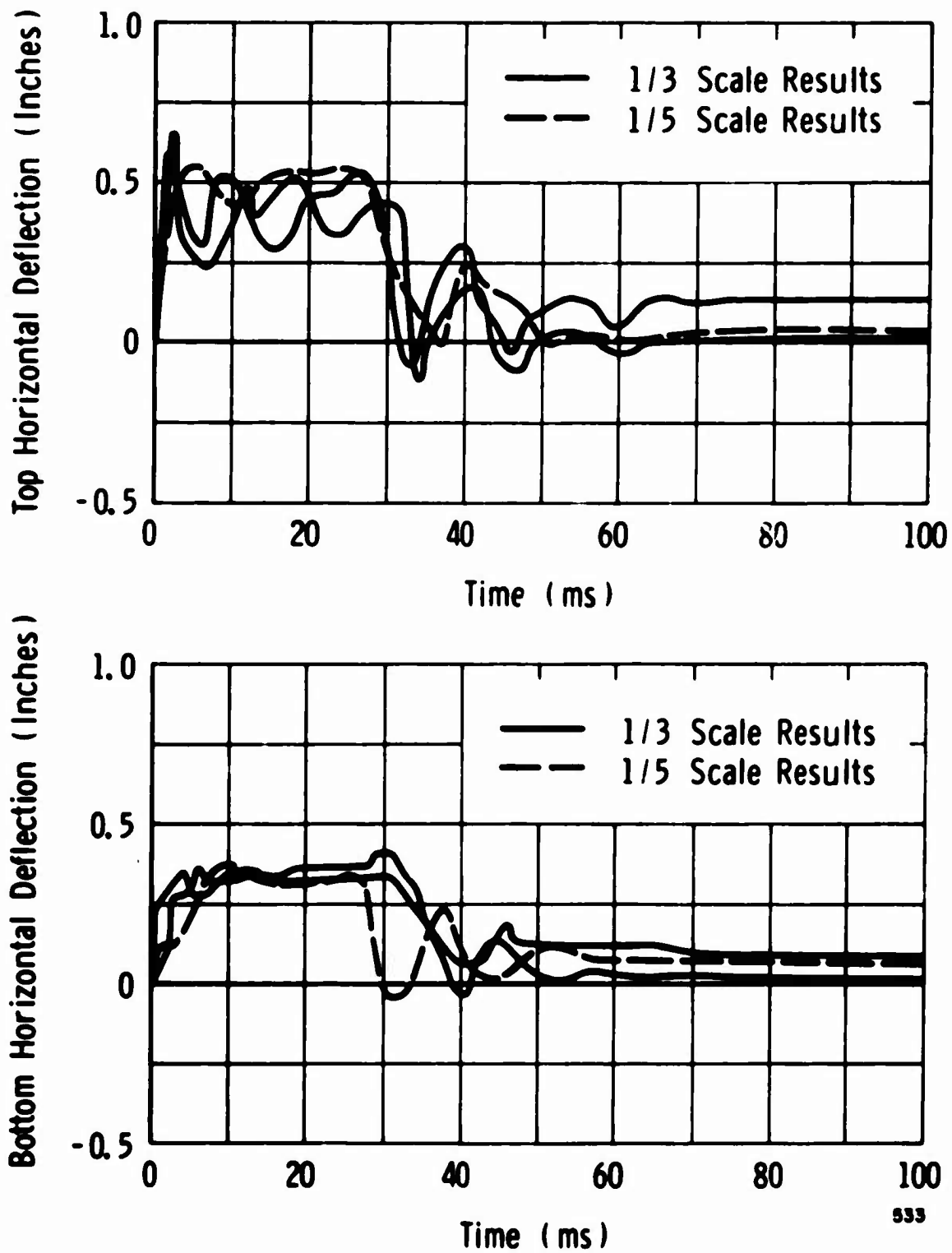
Figure 33. 2nd Test Series Comparing 1/3 And 1/5 Scale Spades
