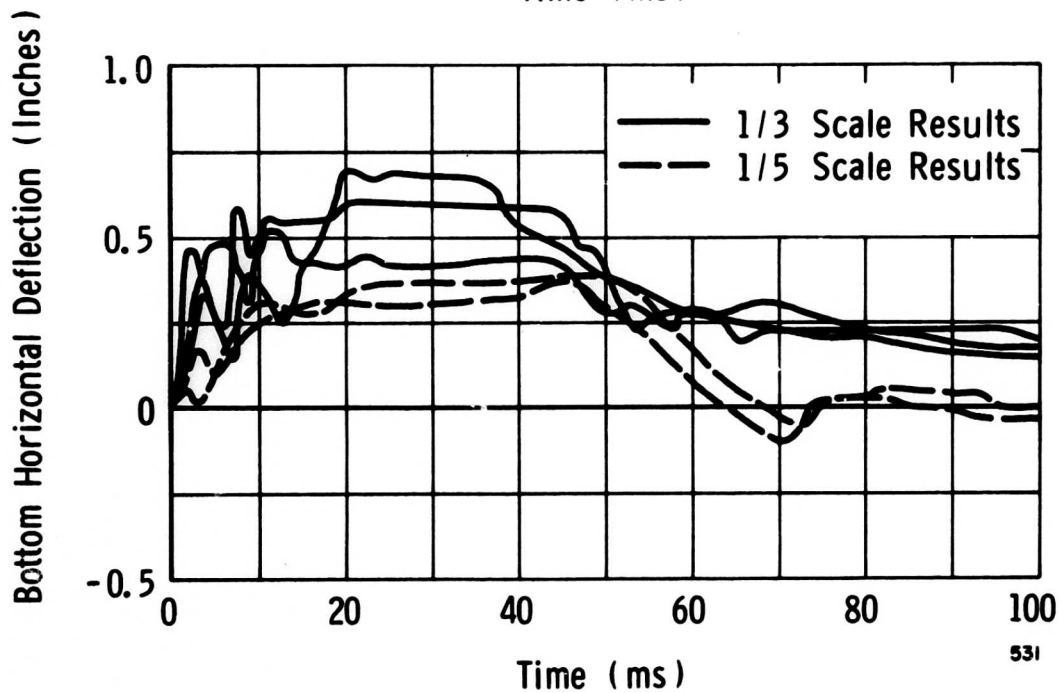
Figure 31. 1st Series Of Tests Comparing 1/3 And 1/5 Scale Spades
