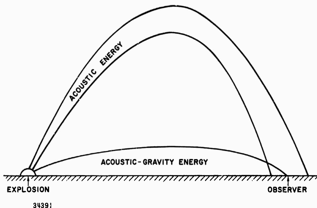
FIG. 49. GROUND CONFINEMENT OF ACOUSTIC-GRAVITY WAVES.
