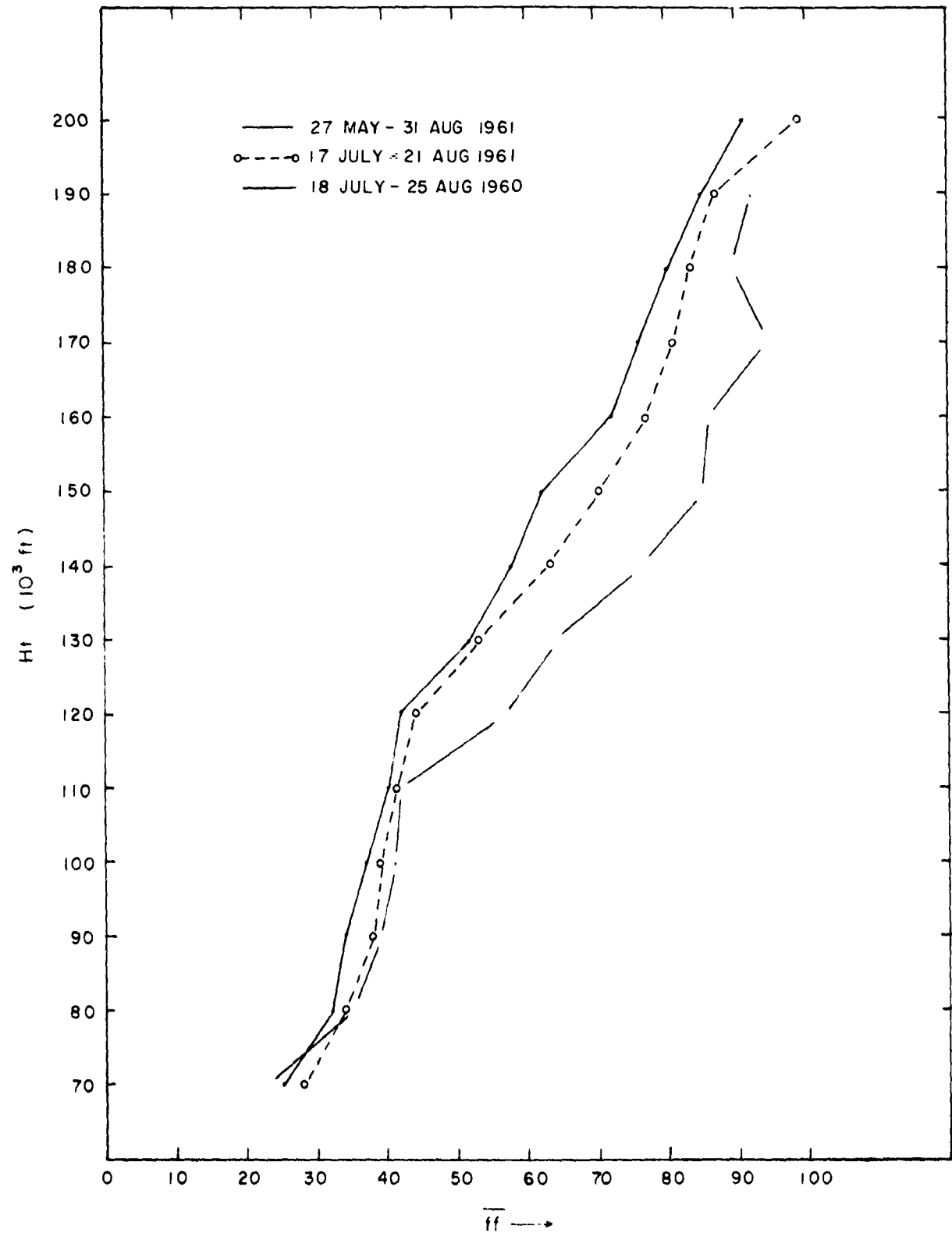
MEAN WIND SPEED WHITE SANDS FIG. 5.
