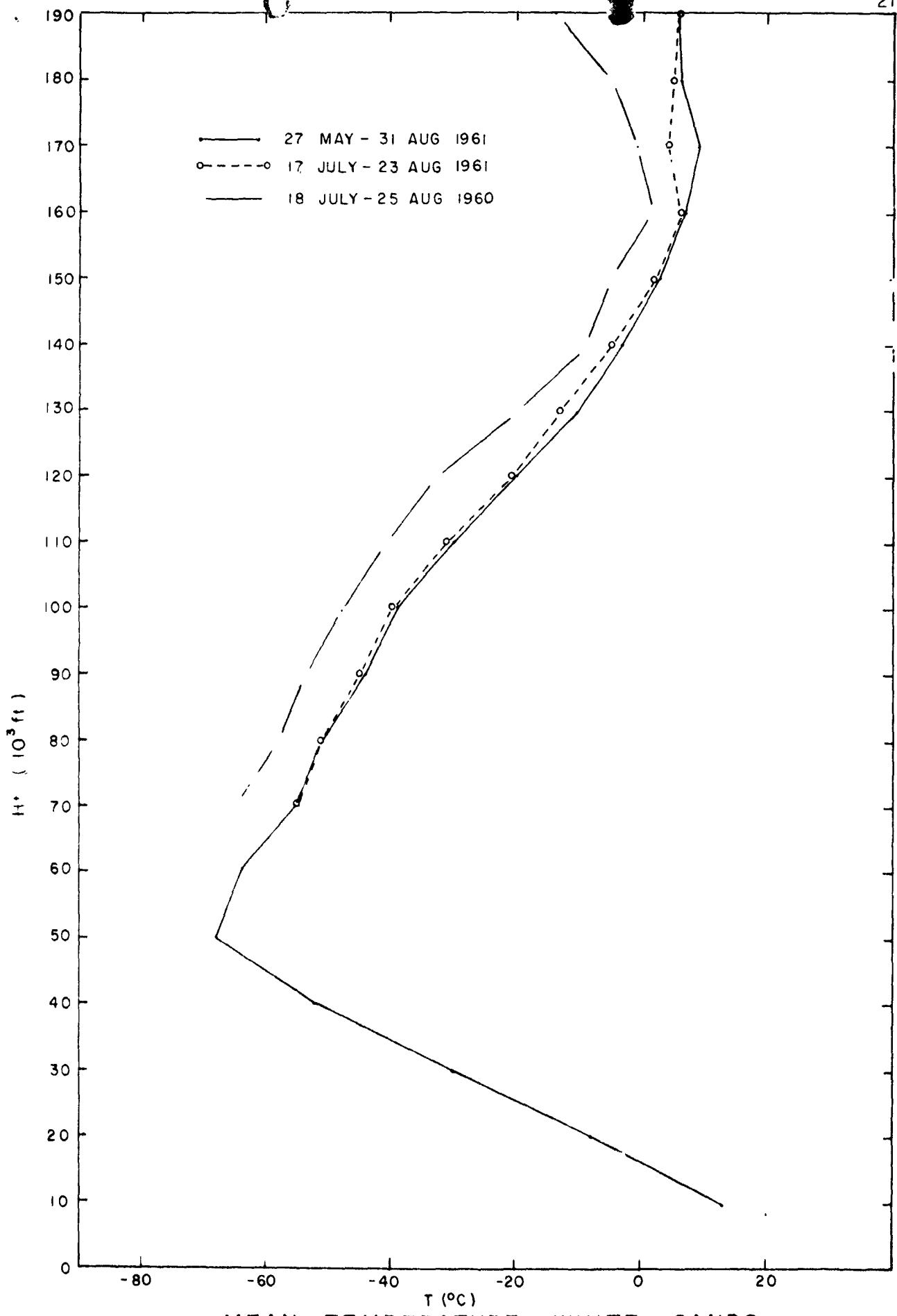
MEAN TEMPERATURE, WHITE SANDS FIG. 2.
