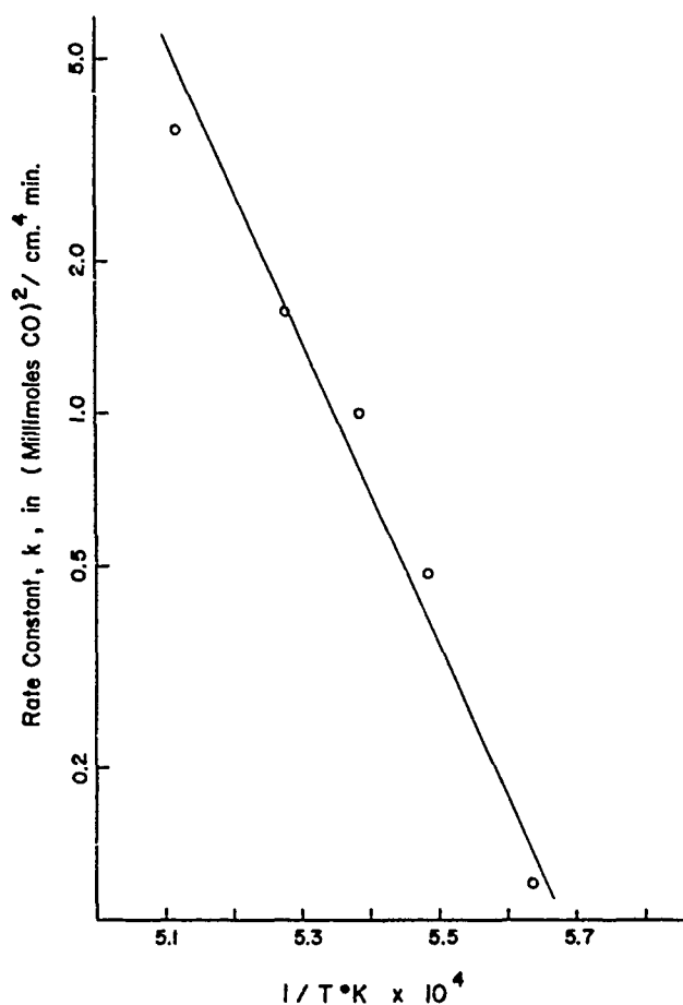
Figure 92. Arrhenius Plot for \text{HfSiO}_4\text{-C} System
