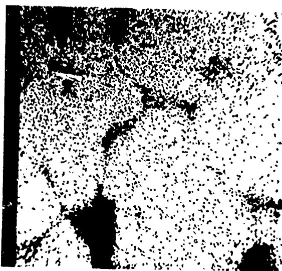
Figure 50. Hf Distribution
