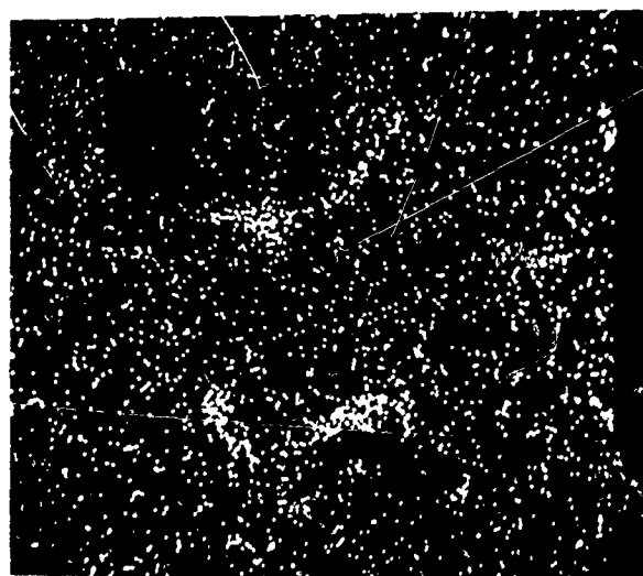
Figure 55. Ca Distribution
