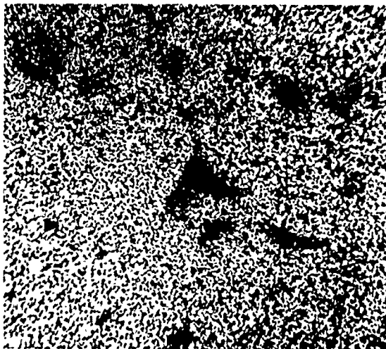
Figure 36. Zr Distribution
