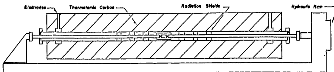
Figure 97. Hot-Pressed Furnace
