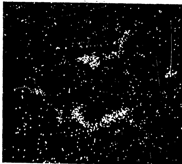
Figure 54. Si Distribution
