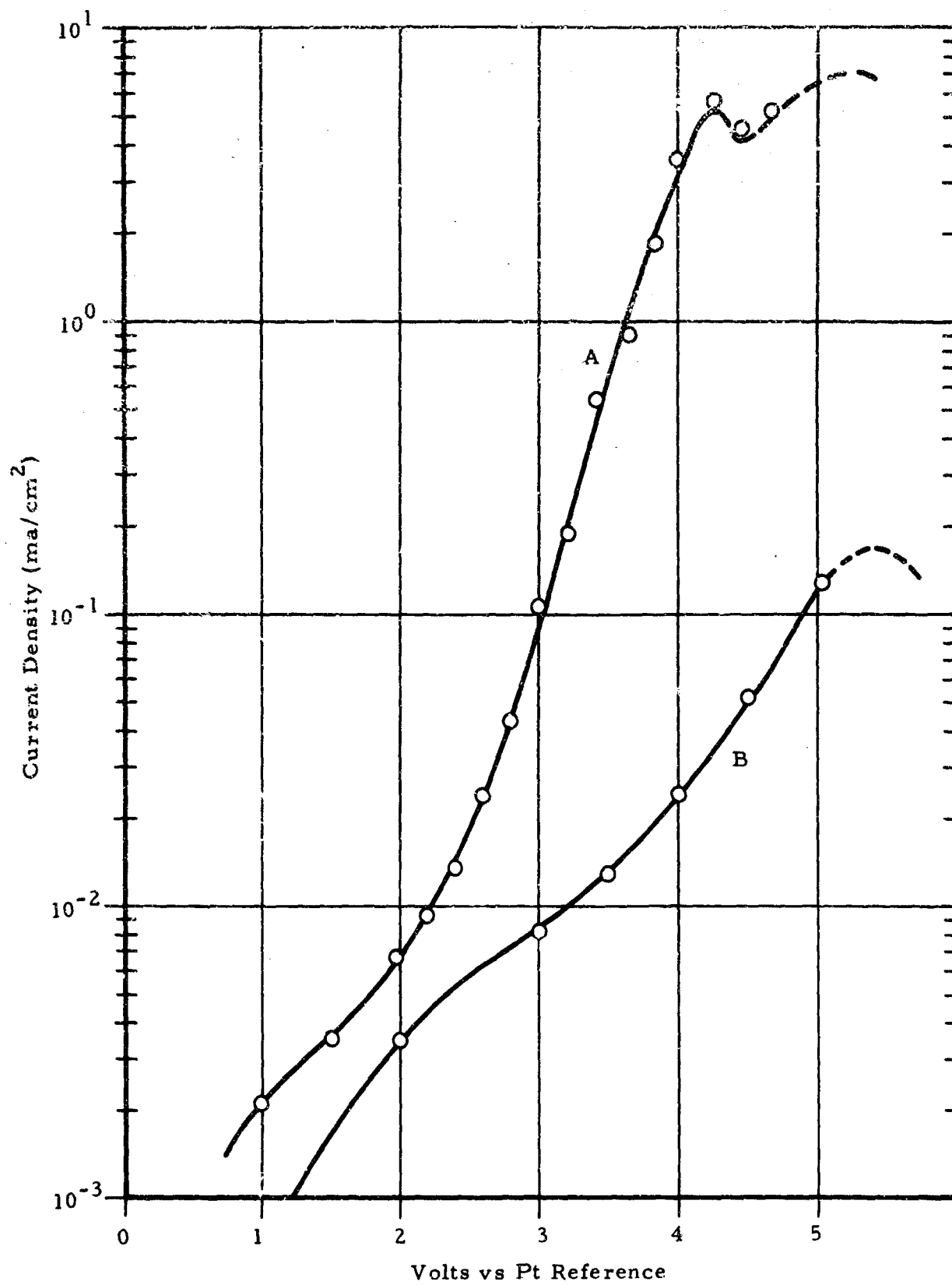
Figure 12. Polarization Curves of Passivated Nickel Electrodes in BrF 3
