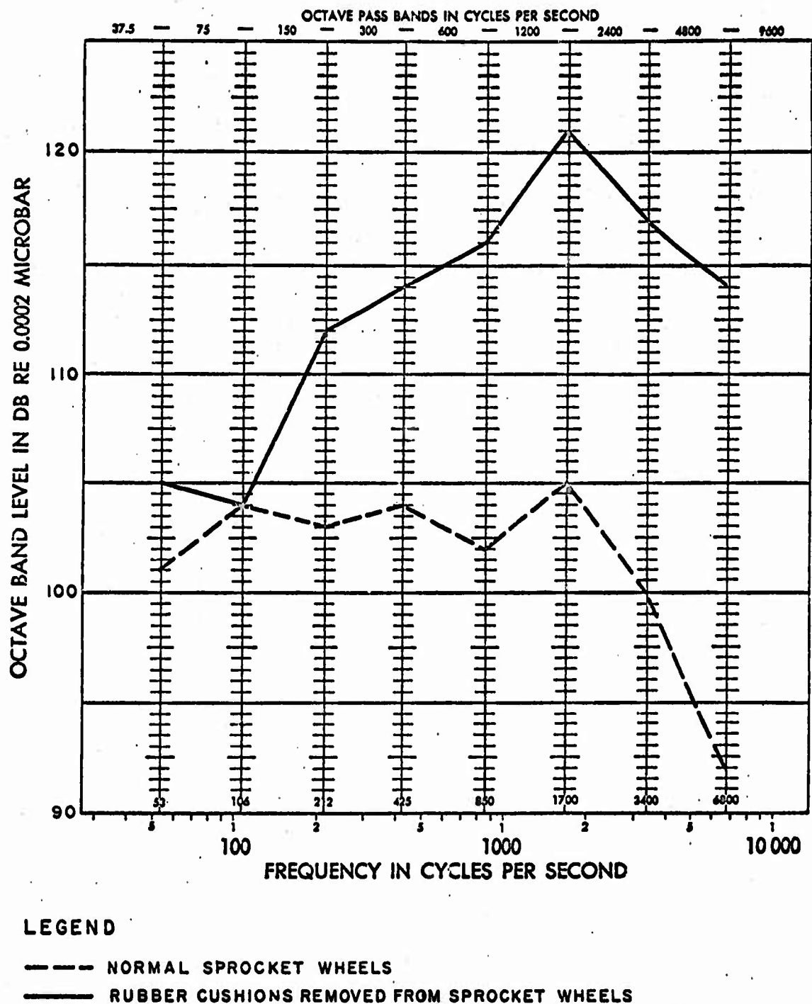
FIGURE 67. EXTERNAL SOUND SPECTRA AT 25 MPH MEASURED NEAR THE RIGHT DRIVE SPROCKET WITH AND WITHOUT THE RUBBER CUSHIONS ON THE SPROCKETS, VEHICLE ON BLOCKS.
