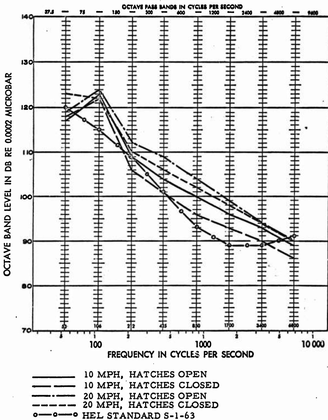
FIGURE 11. INTERNAL SOUND SPECTRA AT THE PASSENGER'S POSITION IN THE RIGHT REAR CORNER.
