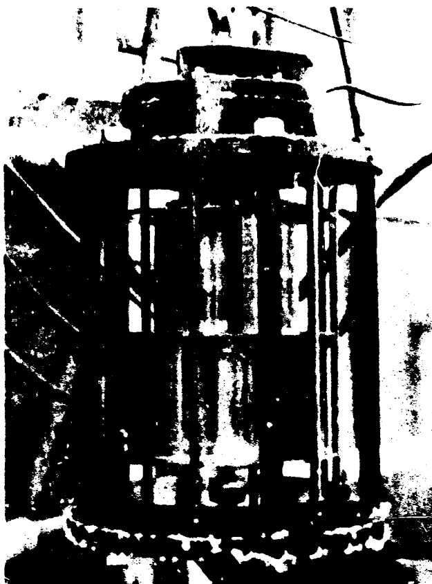
FIGURE 1b. SAVONIUS ROTOR PLACED AT 45-FOOT DEPTH, 30 JUNE - 7 AUGUST 1964
