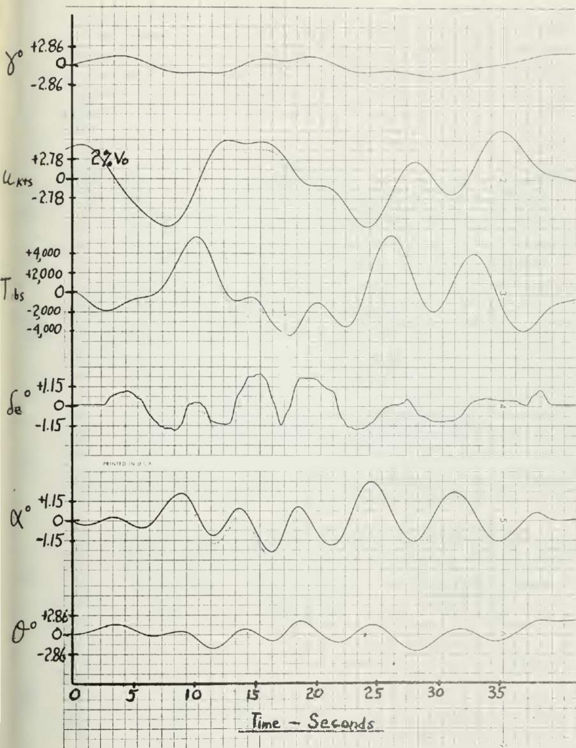
Time History, Human Pilot Controlled Flight on Glide Slope, Sinusoidal Input of 5 Knots Horizontal Gust, System 1-b
