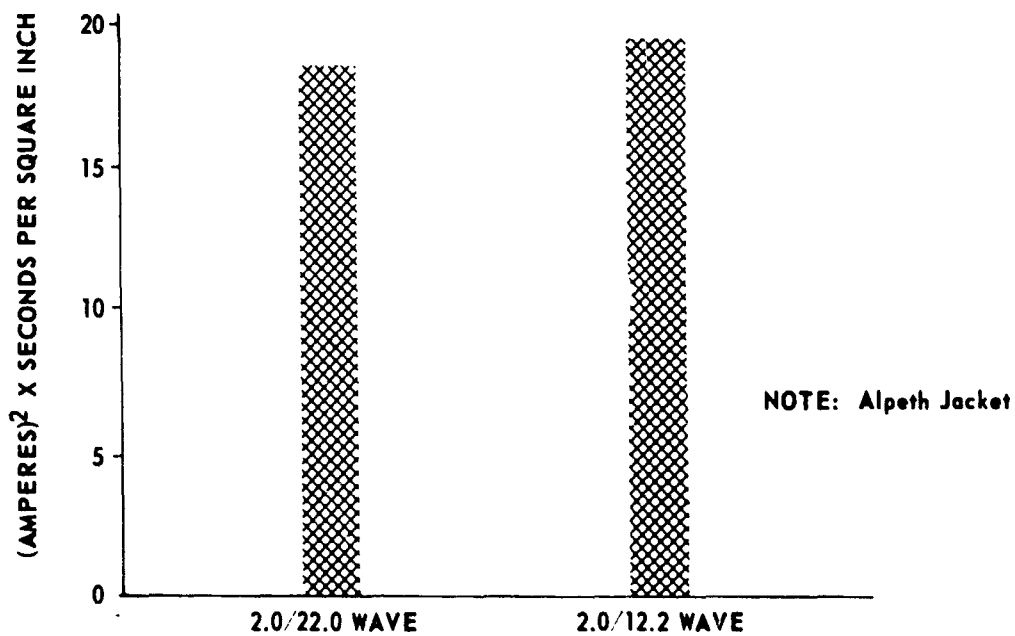
FIG. VI. EFFECT OF WAVESHAPES ON i^2t AT RUPTURE
