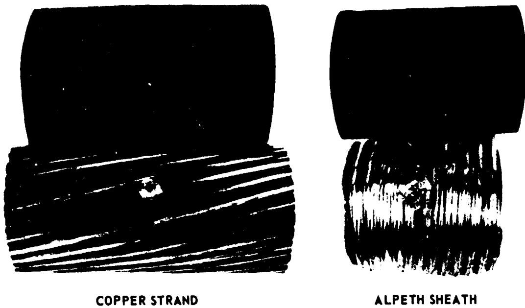
FIG. IV TYPICAL RUPTURES
