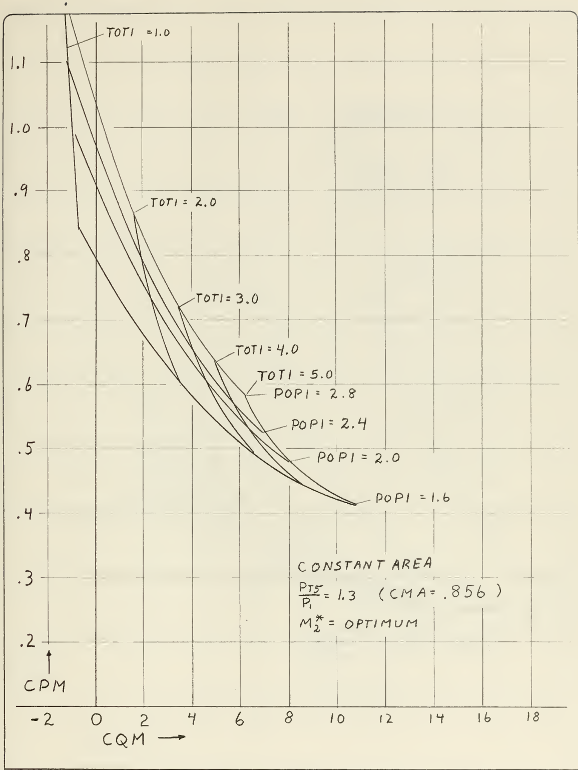
Constant area jet pump optimum performance, CPM vs CQM, for TOT1 and POPI variation, PT5P1 = 1.3 , M_2^* = \text{optimum}
