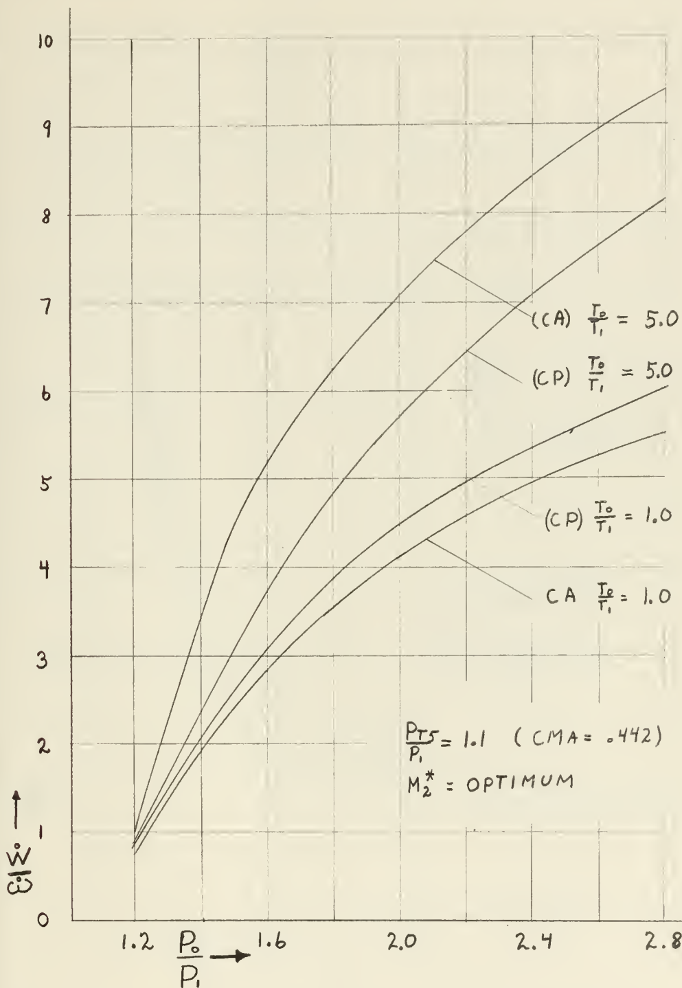
Mass flow ratio \left(\frac{\dot{W}}{\dot{W}_0}, \text{WMWJ}\right) vs Jet total pressure ratio \left(\frac{P_0}{P_1}, \text{POP}_1\right) constant pressure (CP) and constant area (CA), \frac{P_{T5}}{P_1} = 1.1
