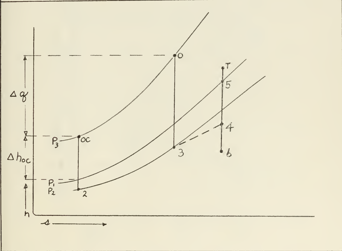
Typical constant area mixing jet pump enthalpy/entropy diagram.
