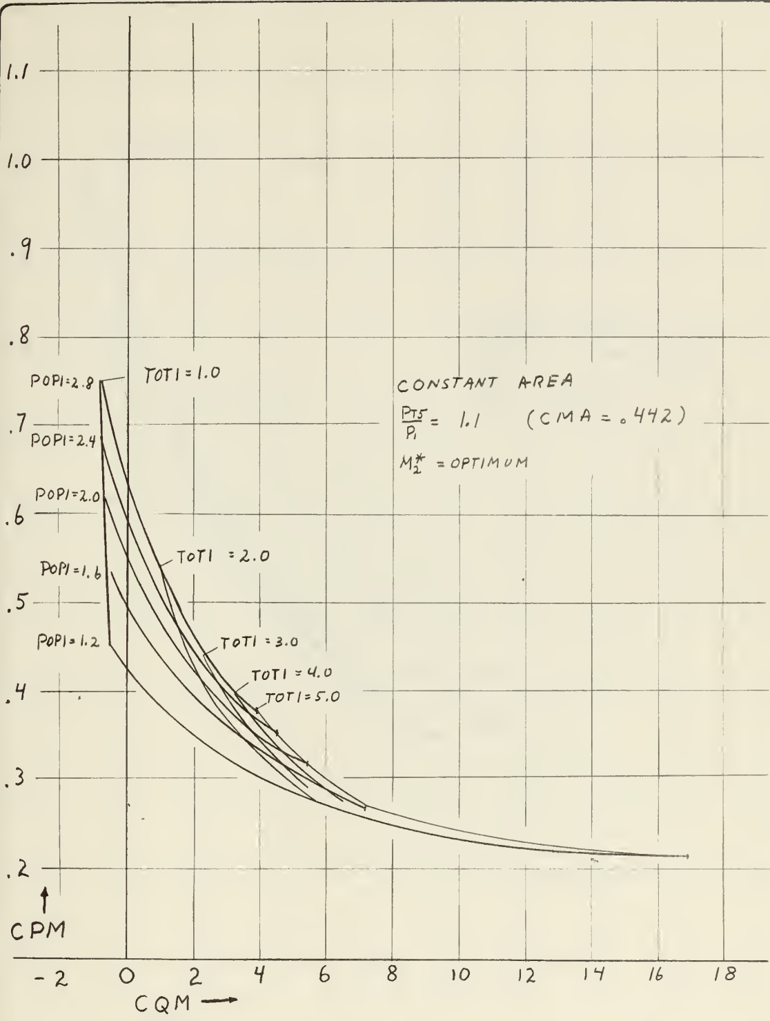
Constant area jet pump optimum performance, CPM vs CQM, for TOT1 and POP1 variation, P_{T5}P_1 = 1.1 , M_2^* = \text{optimum}
