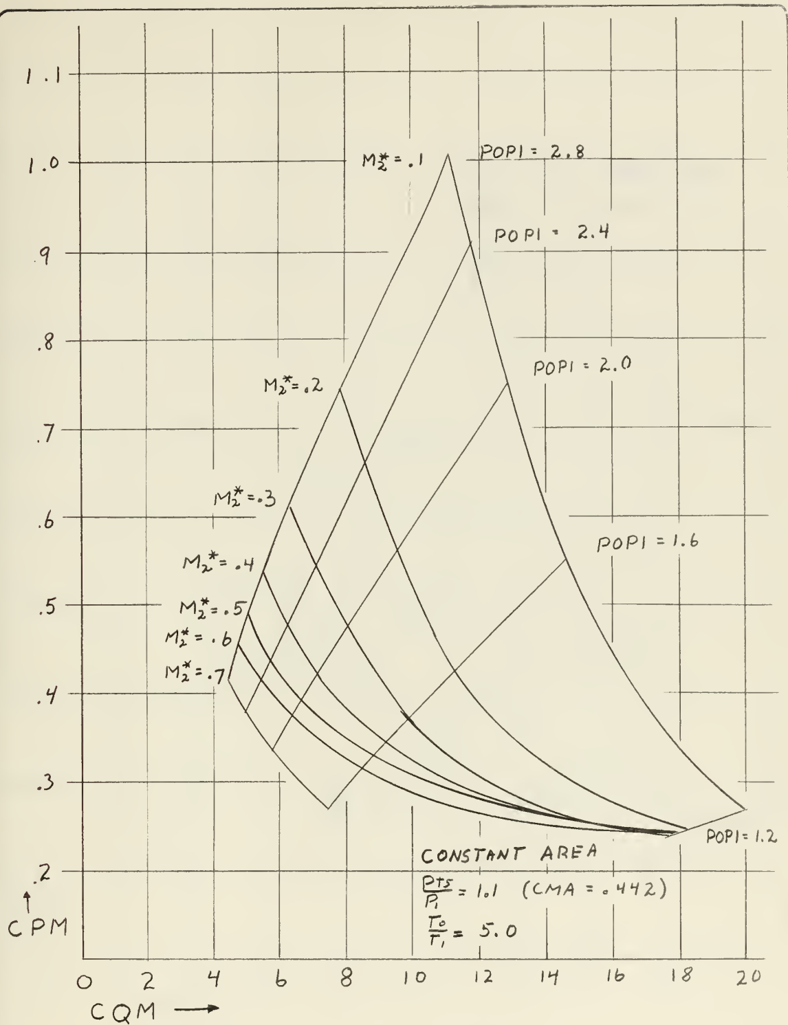
Typical constant area heated jet pump performance, CPM vs CQM, for M_2^* and POPI variation, PT5P1 = 1.1 , TOT1 = 5.0
