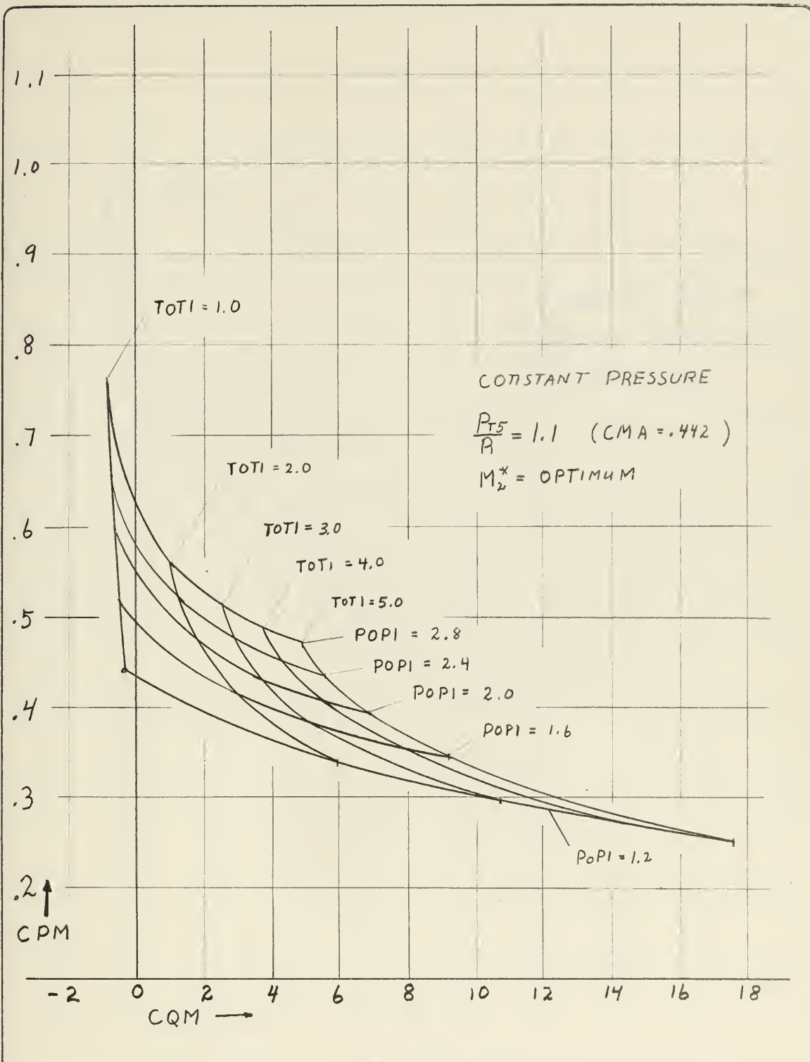
Constant pressure jet pump optimum performance, CPM vs CQM, for TOT1 and POP1 variation, P_{T5P1} = 1.1 , M_2^* = \text{optimum}
