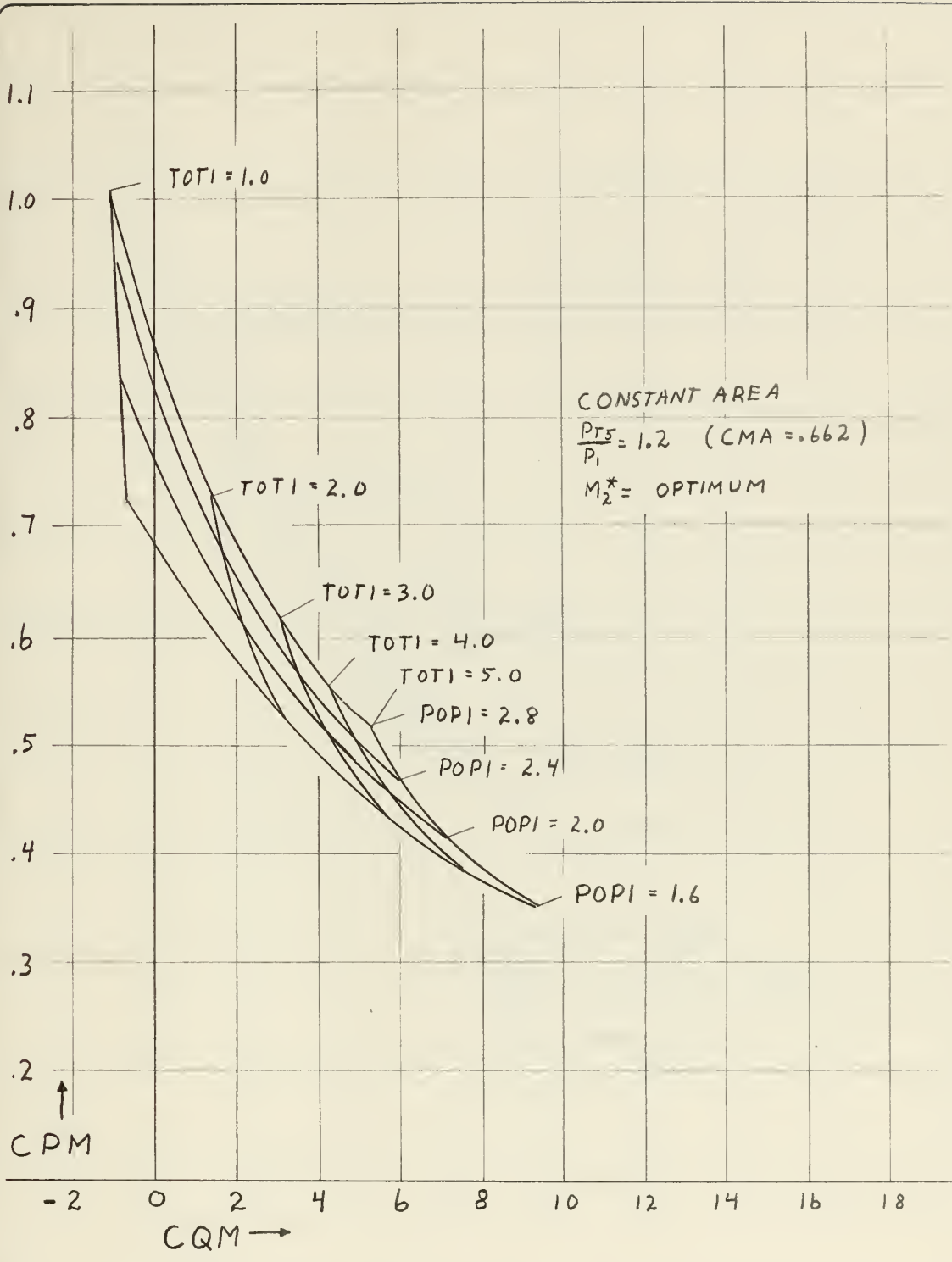
Constant area jet pump optimum performance, CPM vs CQM, for TOT1 and POPI variation, PT5P1 = 1.2 , M_2^* = \text{optimum}
