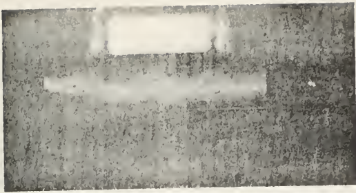
Fig. 37. Ion Oscillations 5 mm from cathode. Scale 005 Volt/cm vertical; 5 micro-sec/cm horizontal. Tube pressure 10 microns, Discharge current 65 milliamperes.
