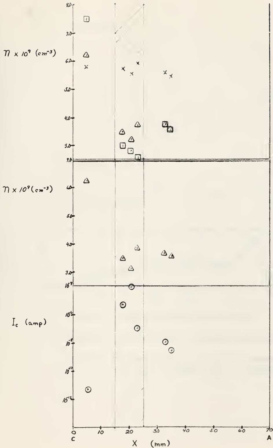
Fig. 32. Upper plot: (□) Electron density by Druyvesteyn (Δ) Electron density by frequency (x) Ion density (corrected)
