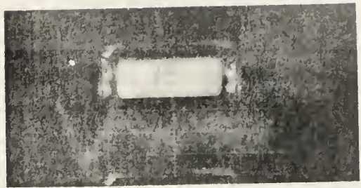
Fig. 38. Ion Oscillations 18 mm from cathode. Scale .02 Volt/cm vertical; 5 micro-sec/cm horizontal. Tube pressure 10 microns, Discharge current 65 milliamperes.
