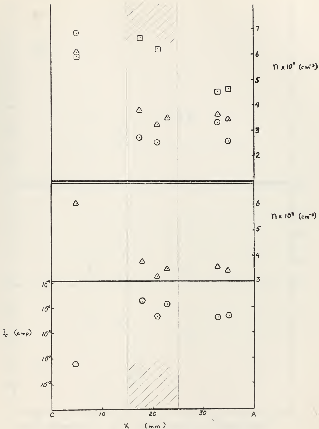
Fig. 30. Upper plot: ( \odot ) electron density by Druyvesteyn ( \triangle ) electron density by frequency ( \boxtimes ) ion density (corrected)
